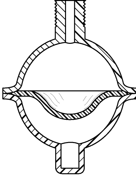
Existing design w/ Air Cushion compressed (air cushion compresses due to pressure)
