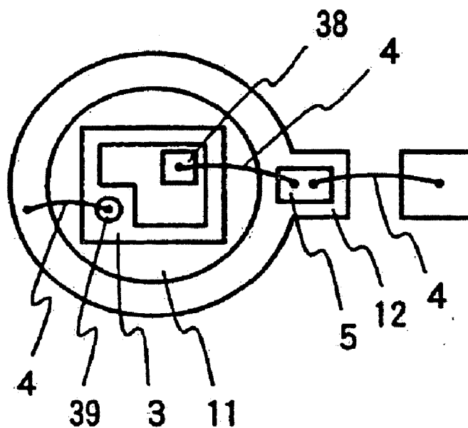
FIG. 2 (PRIOR ART)
