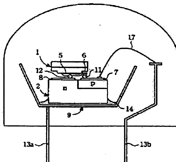
FIG. 3 (PRIOR ART)
