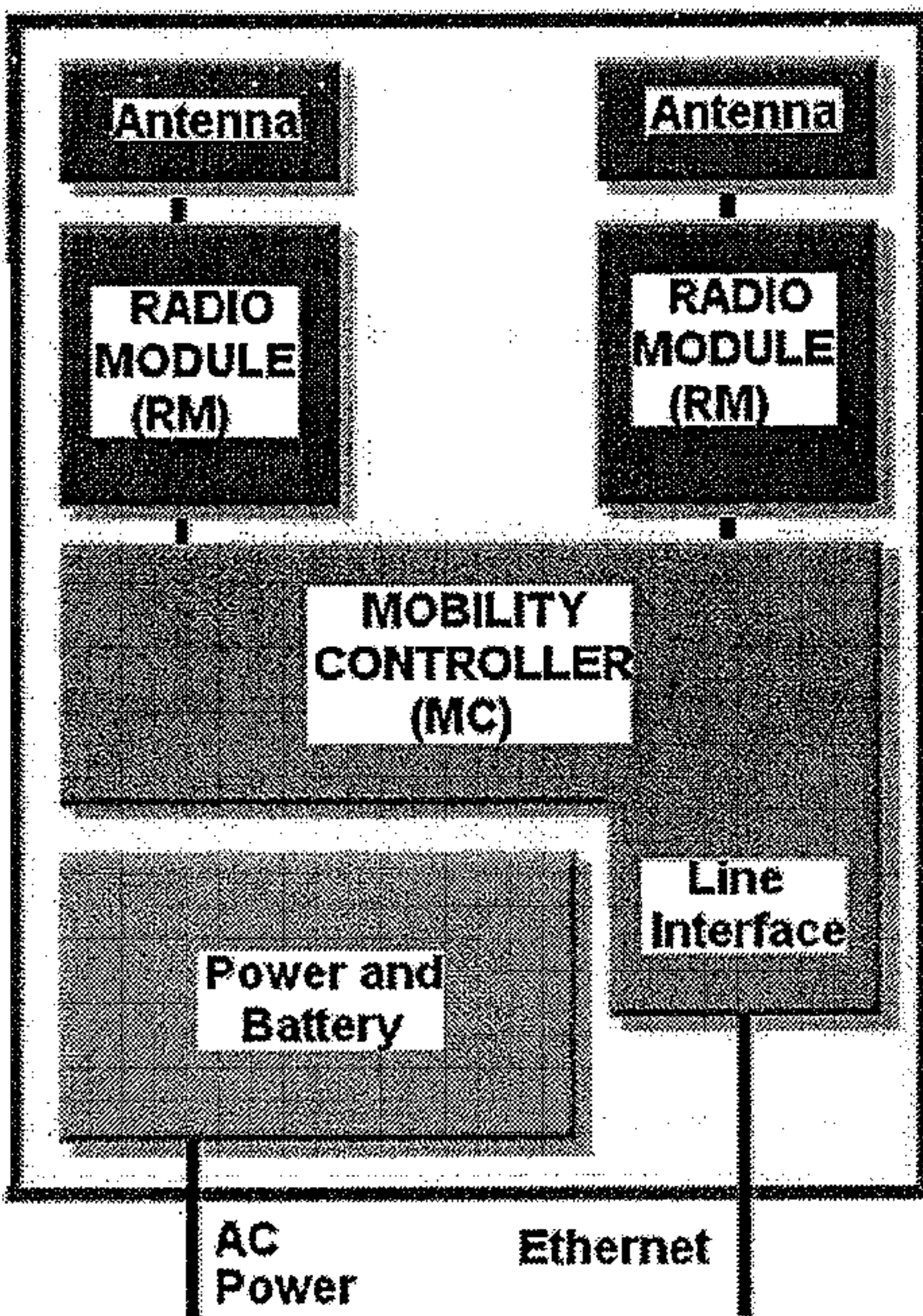
BelAir100D Internal Architecture
