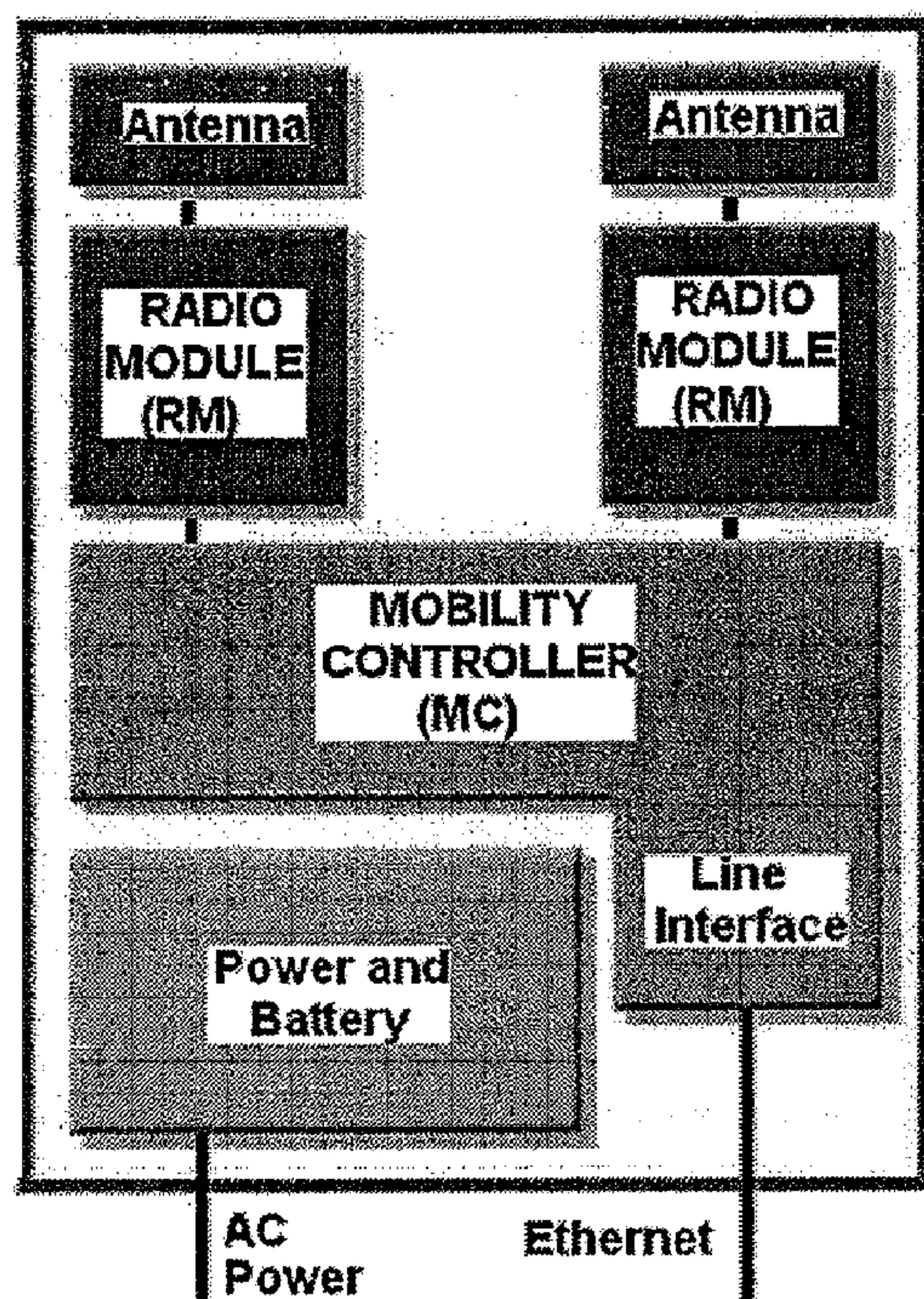
BelAir100D Internal Architecture
