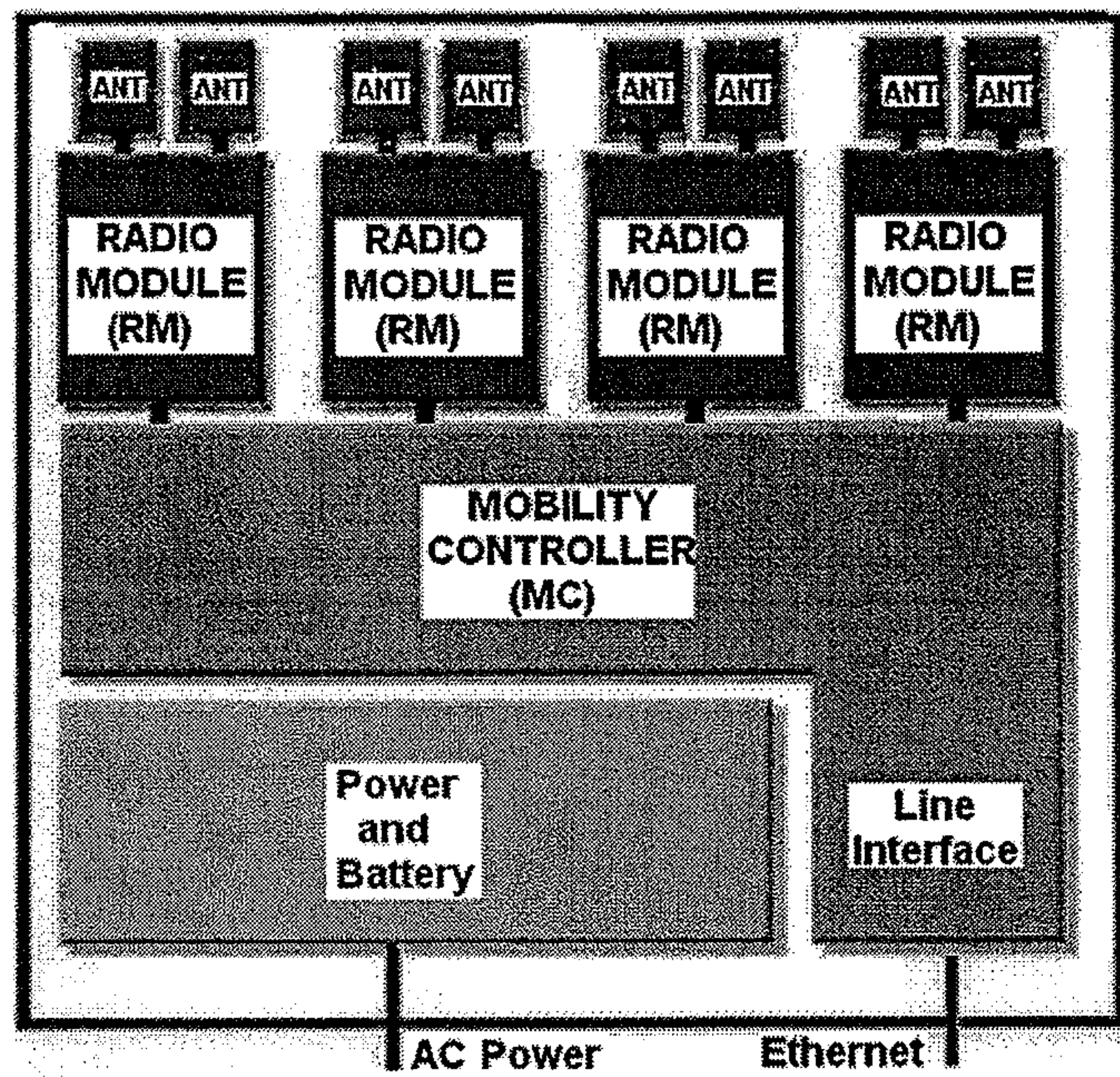
BelAir200D Internal Architecture
