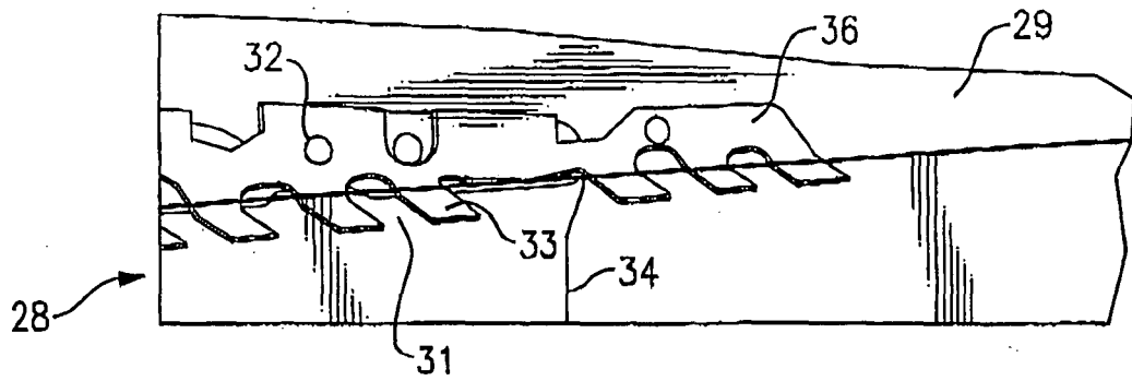
FIG. 5 Prior Art
