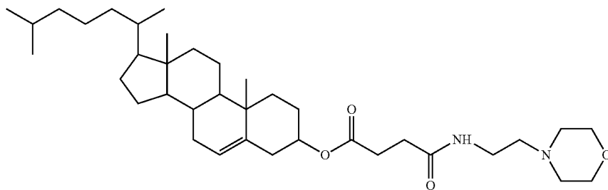
HisChol Histaminyl-Cholesterolhemisuccinate:
