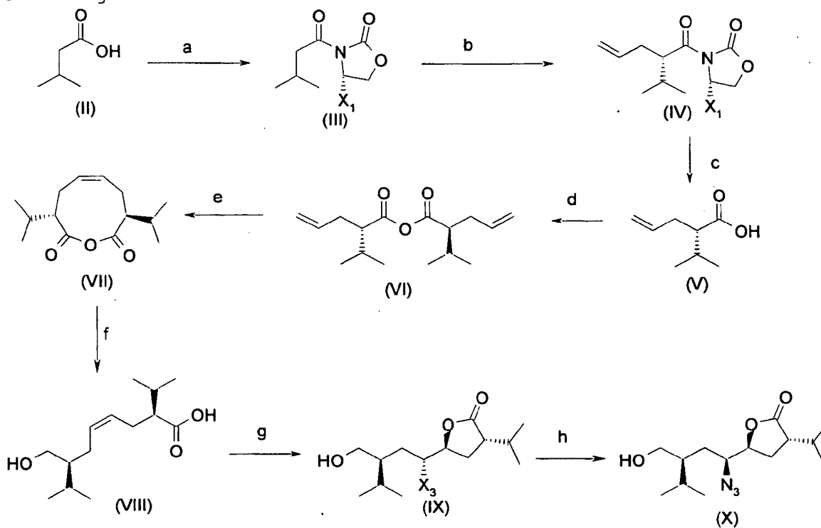
Scheme 1: A method for preparing a compound of formula (X) starting from isovaleric acid
