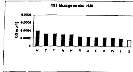
Figure 2A. Y61 Heavy Chain CDR H1 Mutagenesis
