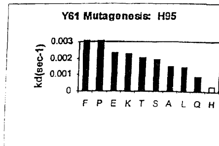
Figure 2D. Y61 Heavy Chain CDR H3 Mutagenesis
