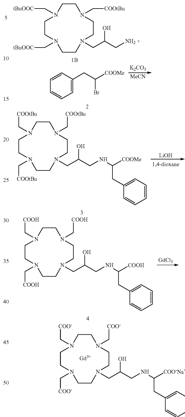
Scheme 15
