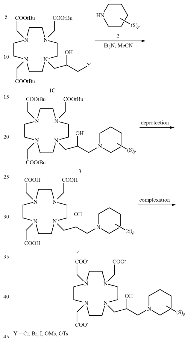
Scheme 2
