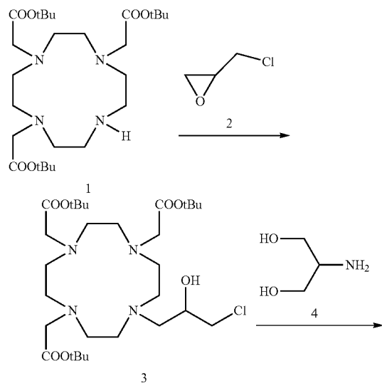
Scheme 19
