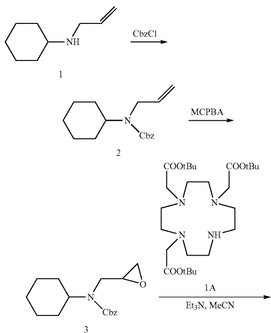
Scheme 17
