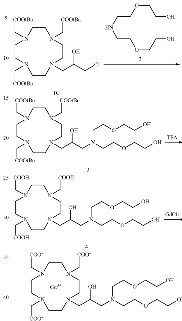
Scheme 20
