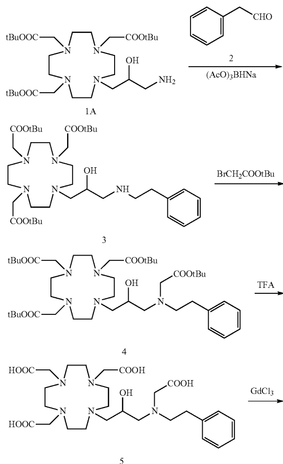
Scheme 22
