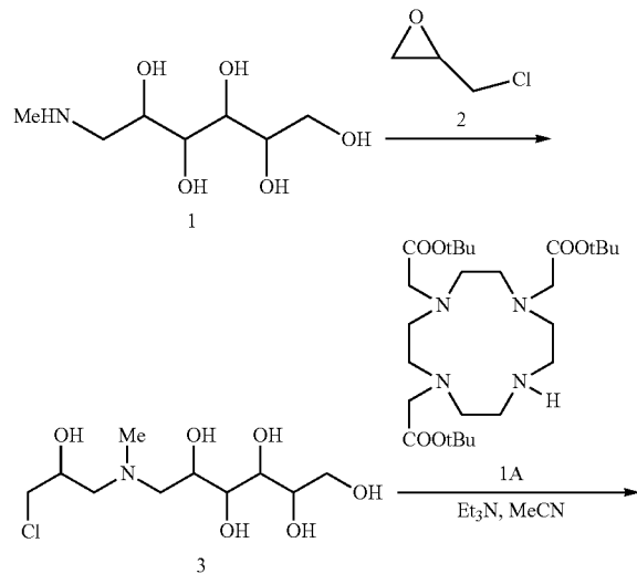
Scheme 21
