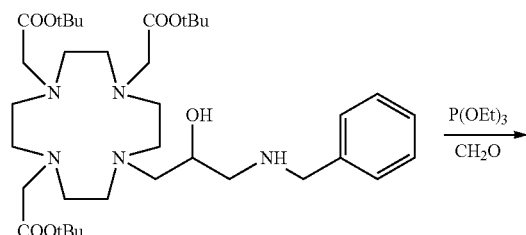
Scheme 13
