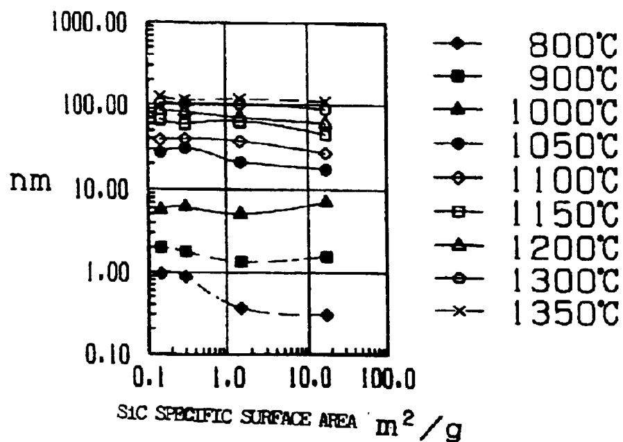
FIG. 4 THICKNESS OF OXIDE LAYER
