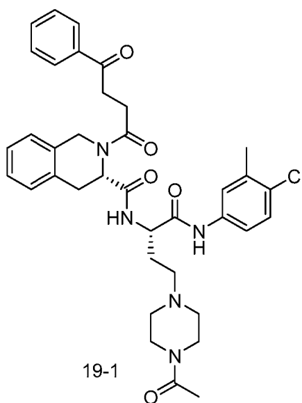
Scheme 19
