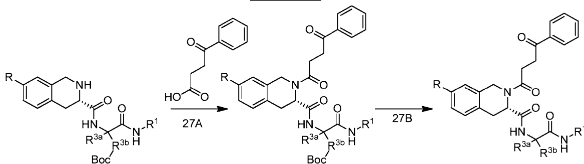
Scheme 27
