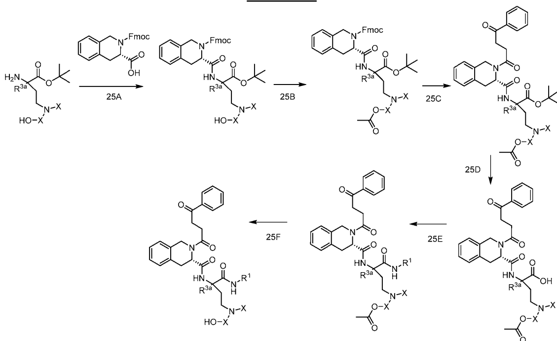
Scheme 25
