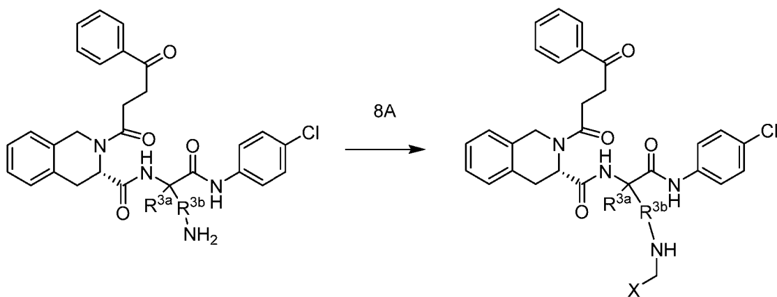
Scheme 8
