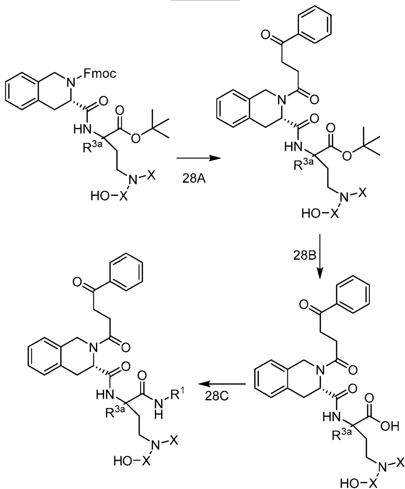
Scheme 28
