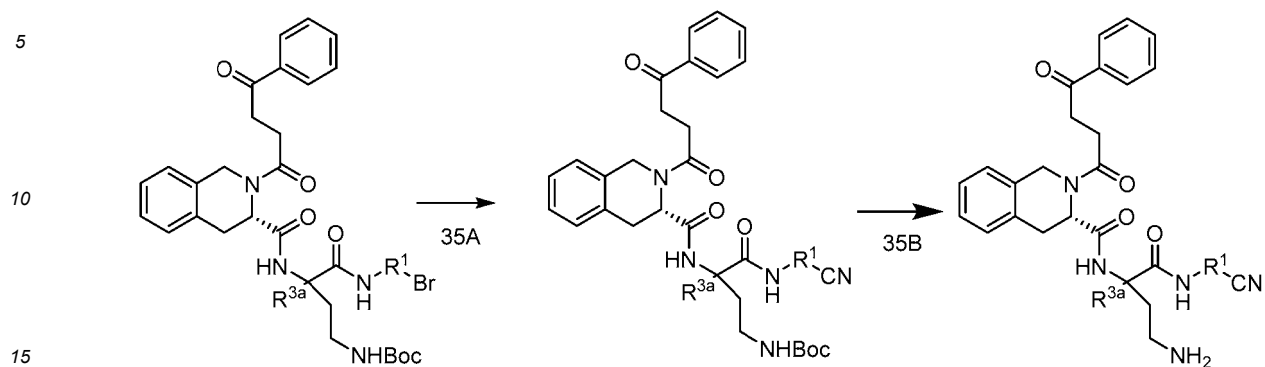
Scheme 35
