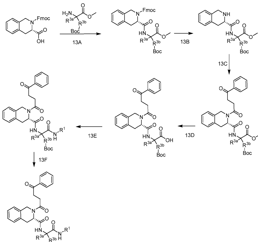
Scheme 13
