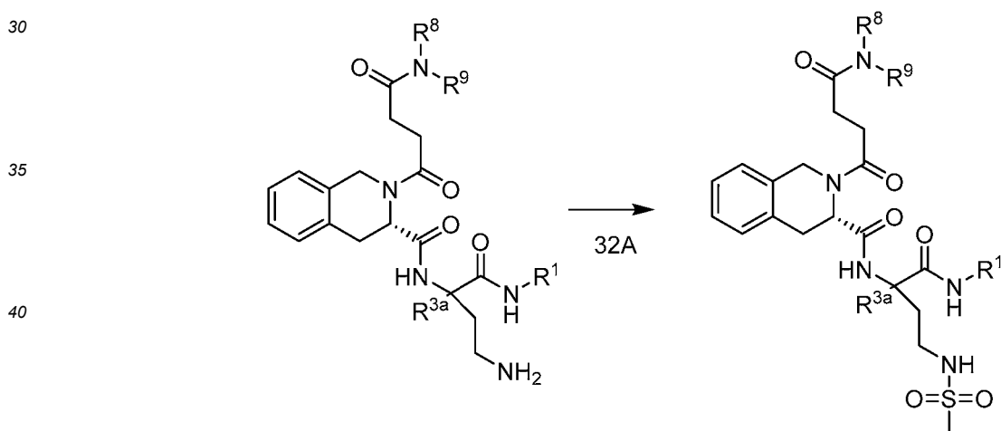
Scheme 32
