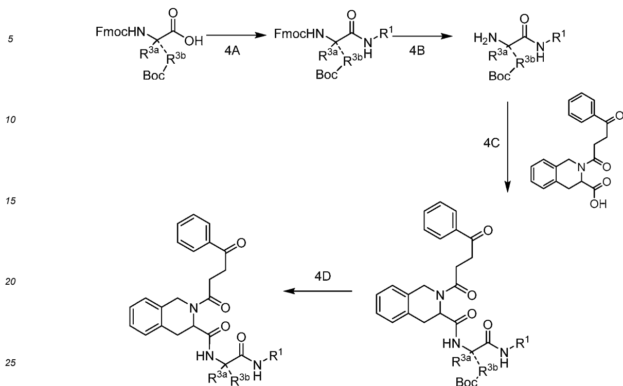
Scheme 4
