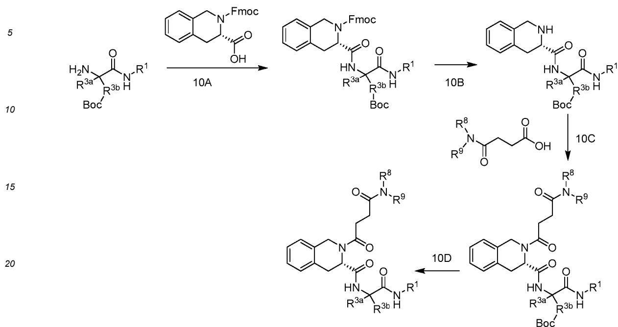
Scheme 10
