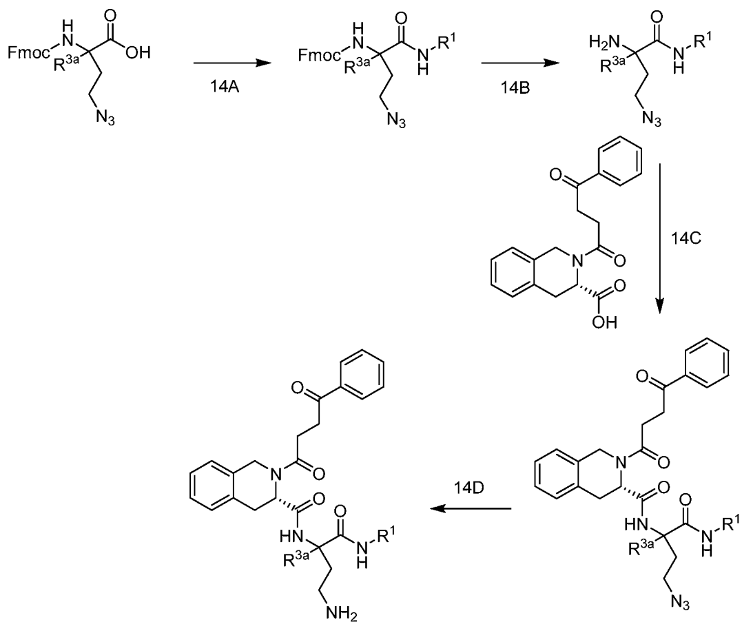
Scheme 14
