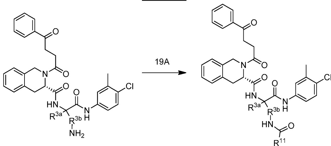
Scheme 19
