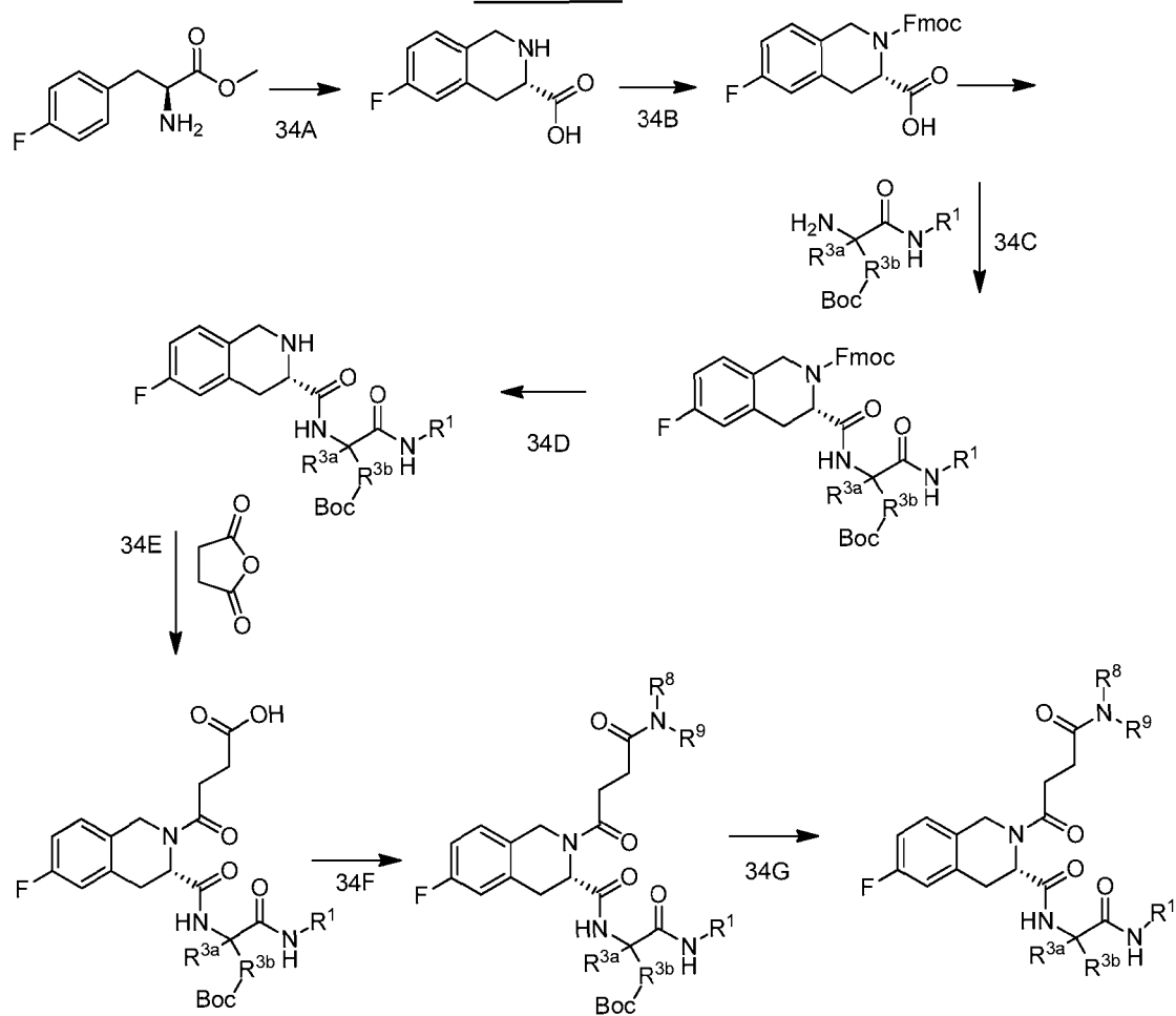
Scheme 34
