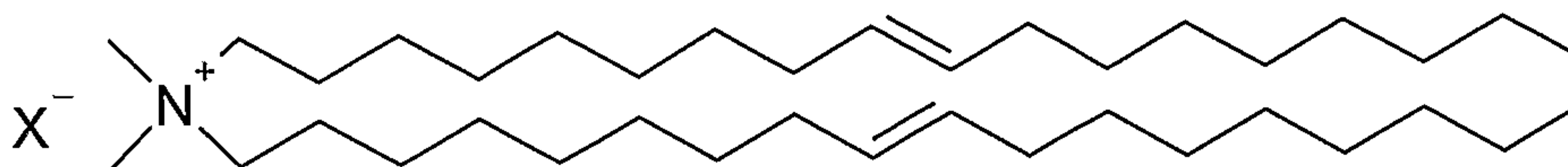
Dimethyldioctadecenylammonium (DODA-X)
