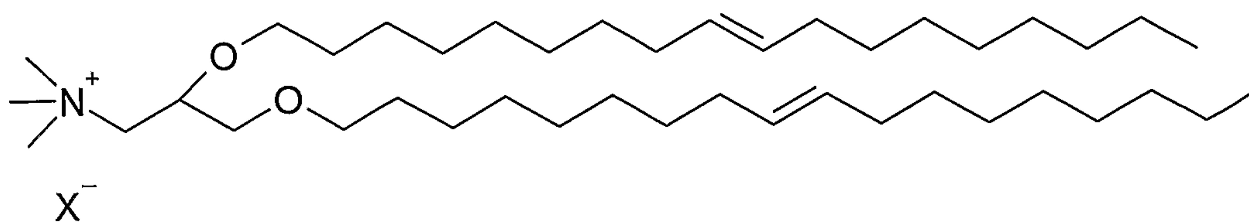
N-[1-(2,3-dioleyloxy)propyl]-N,N,N-trimethylammonium (DOTMA)
