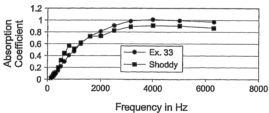
Fig. 6 Normal Incidence Sound Absorption Coefficient
