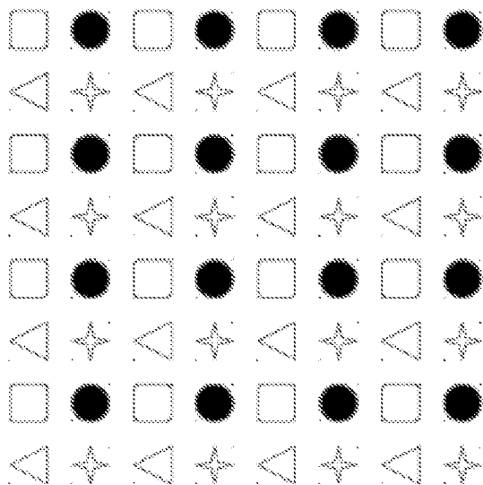
120 Dyadic sub-lattices
