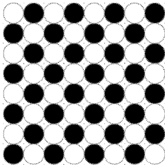
110 Quincunx sub-lattices
