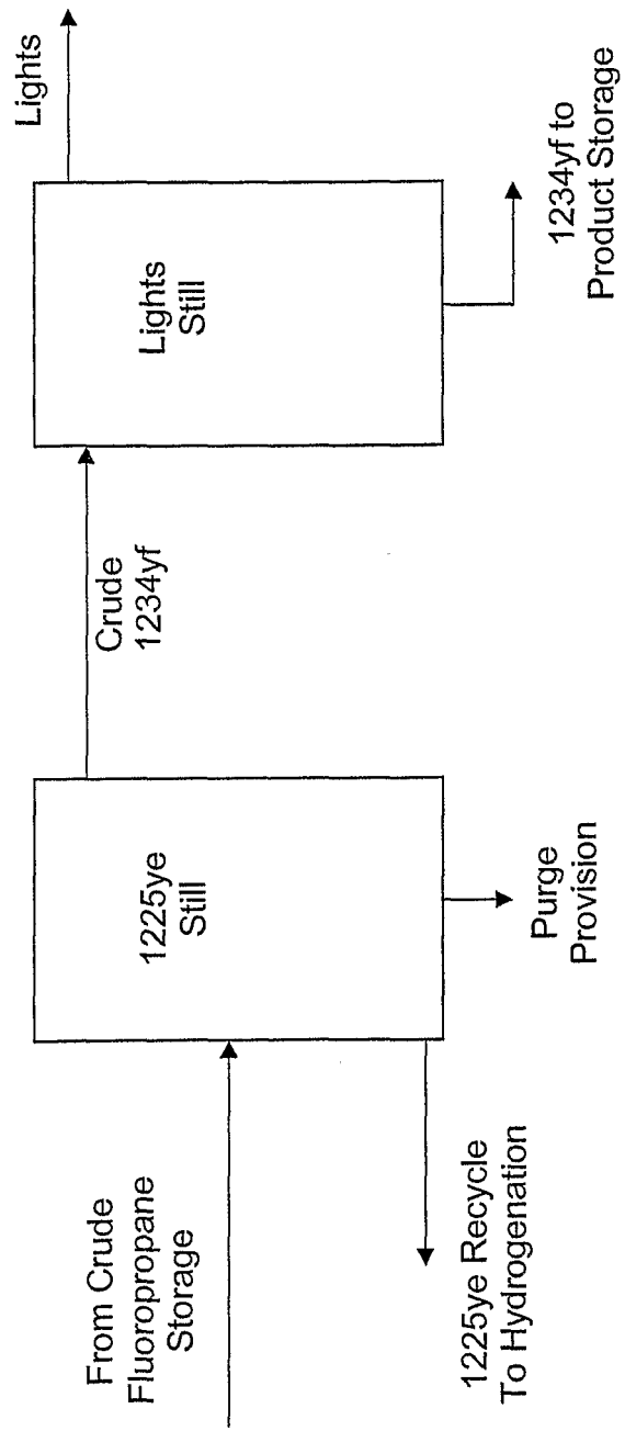
Figure 3: Purification of 1225ye and 1234yf
