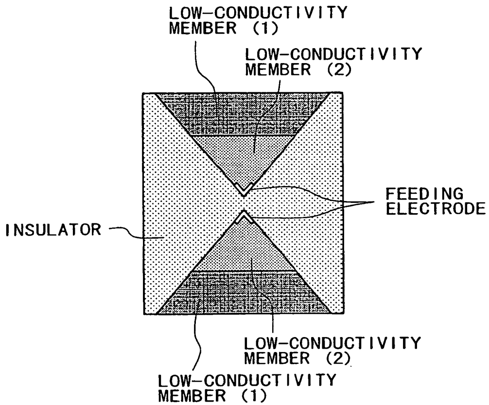
CROSS-SECTIONAL VIEW
