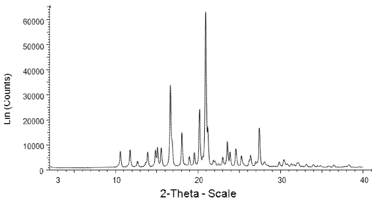
Figure A: X-Ray Powder Diffraction Pattern of Compound A, Form A
