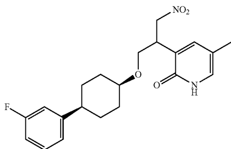
5-methyl-3-(1-nitro-3-([(CIS)-4-(3-fluorophenyl)cyclohexyl]oxy)propan-2-yl)-1,2-dihydropyridin-2-one
