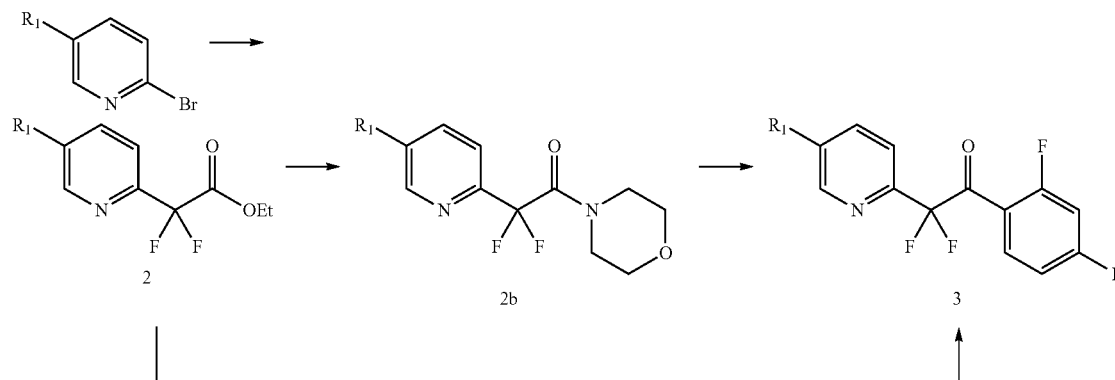
Scheme 2. Synthesis of ketone 3
