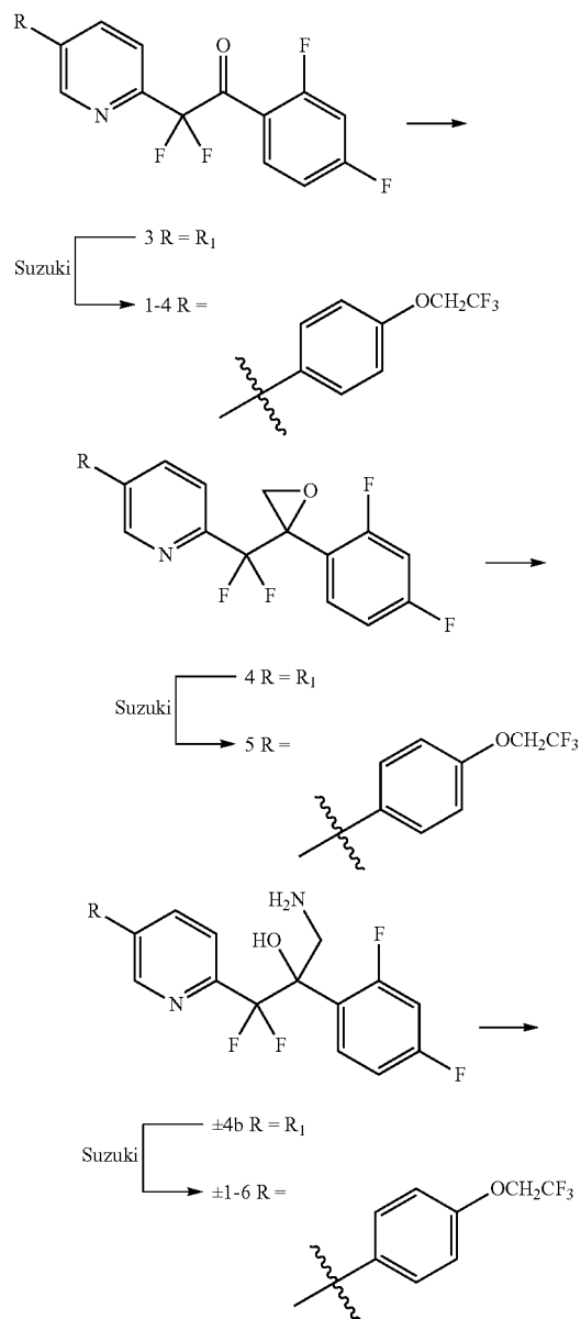
Scheme 3. Synthesis of 1 or 1a via TMSI Epoxidation Method
