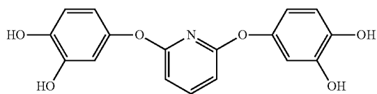
2,6-bis(3,4-dihydroxyphenoxy)pyridine
