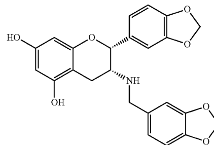
3-deoxy-3-(3,4-methylenedioxybenzyl)-aminoepicatechin
