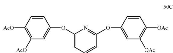
2,6-bis(3,4-diacetoxyphenoxy) pyridine
