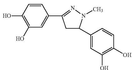
3,5-bis(3,4-dihydroxyphenyl)-1-methyl-1H-pyrazoline
