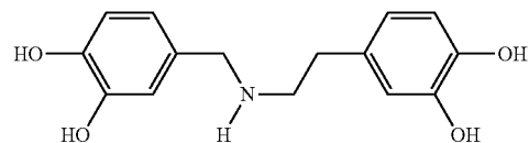
N-(3,4-dihydroxybenzyl)-3,4-dihydroxy(-) phenethylamine
