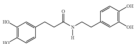
3-(3,4-dihydroxyphenyl)propionic acid 3,4-dihydroxyphenethylamide
