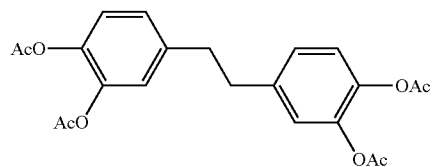
1,2-bis(3,4-diacetoxyphenyl)ethane
