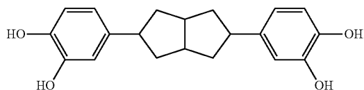
2,5-bis(3,4-dihydroxybenzyl)bicyclo[3.3.0](-) octane
