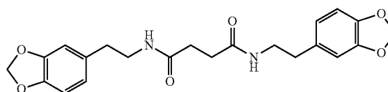
Succinic acid bis(3,4-methylenedioxyphenethylamide)
