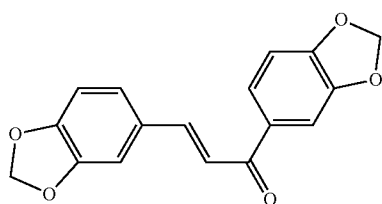
bis(3,4-methylenedioxy)chalcone
