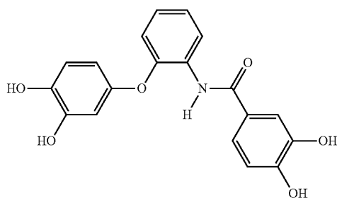
3,4-dihydroxybenzoic acid o-(3,4-dihydroxyphenoxy)anilide
