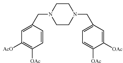
1,4-bis(3,4-diacetoxybenzyl)piperazine
