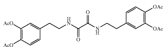
Oxalic acid bis(3,4-diacetoxylphenethylamide)
