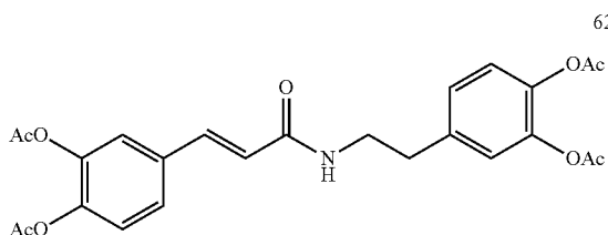
3,4-diacetoxycinnamic acid 3,4-diacetoxylphenethylamide
