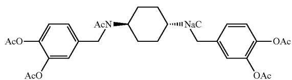
N,N'-bis(acetyl)-bis(3,4-diacetoxybenzyl)-trans-1,4-diaminocyclohexane
