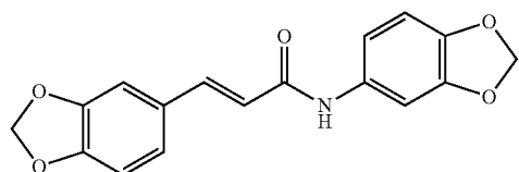
3,4-methylenedioxcinnamic acid 3,4-methylenedioxyanilide
