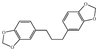
1,3-bis(3,4-methylenedioxyphenyl)propane
