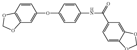
3,4-methylenedioxybenzoic acid p-(3,4-methylenedioxyphenoxy)anilide
