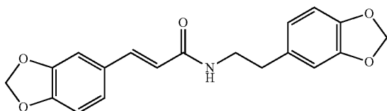
3,4-methylenedioxcinnamic acid 3,4-methylenedioxyphenethylamide
