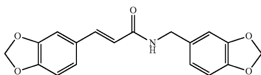
3,4-methylenedioxcinnamic acid 3,4-methylenedioxybenzylamide
