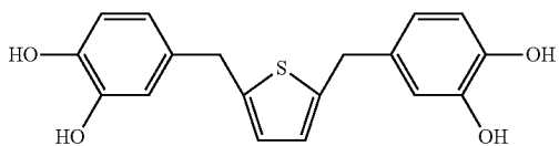
2,5-bis(3,4-dihydroxybenzyl)thiophene
