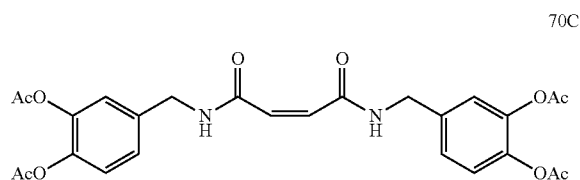
Maleic acid bis(3,4-diacetoxybenzylamide)
