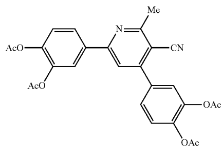
4,6-bis(3,4-diacetoxyphenyl)-3-cyano-2-methylpyridine
