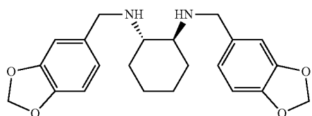
N,N'-bis(3,4-methylenedioxybenzyl)-trans-1,2-diaminocyclohexane
