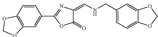
4-(3,4-methylenedioxybenzylaminomethylene)-1-(3,4-methylenedioxyphenyl)oxazolin-5-one
