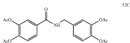
3,4-diacetoxybenzoic acid 3,4-diacetoxylbenzylamide
