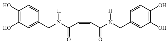
Maleic acid bis-(3,4-dihydroxybenzylanilide)
