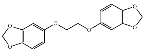
1,2-bis(3,4-methylenedioxyphenoxy) ethane
