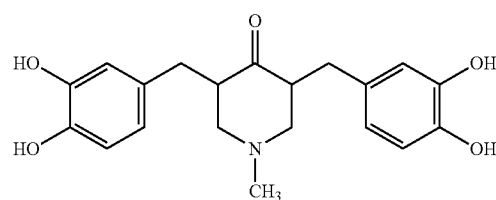
3,5-bis(3,4-dihydroxybenzyl)-1-methyl-4-piperidinone
