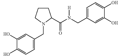
N-(3,4-dihydroxybenzyl)proline 3,4-dihydroxy-benzylamide
