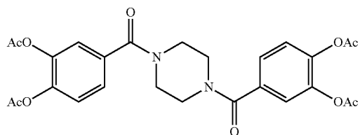
1,4-bis(3,4-diacetoxybenzoyl) piperazine
