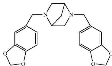
2,5-bis(3,4-methylenedioxybenzyl)-2,5-diaza[2,2,1]-bicycloheptane
