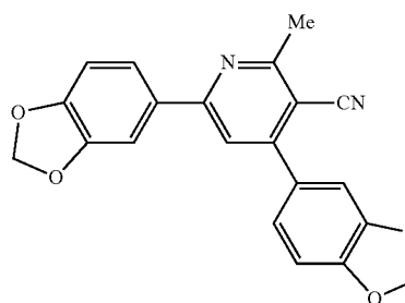
4,6-bis(3,4-methylenedioxyphenyl)-3-cyano-2-methylpyridine
