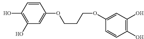
1,3-bis(3,4-dihydroxyphenoxy)propane
