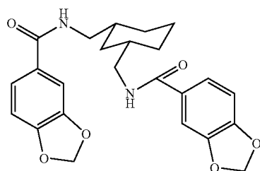
N,N'-bis(3,4-methylenedioxybenzoyl)-cis-1,3-bis-aminomethylcyclohexane
