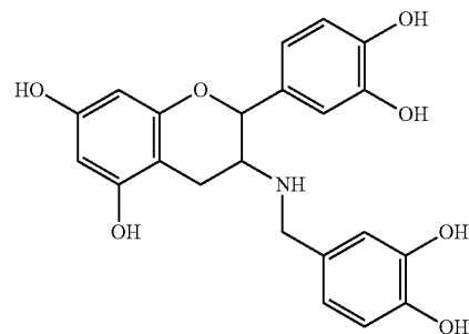
3-deoxy-3-(3,4-dihydroxybenzyl)(-)-amino- epicatechin
