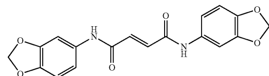
Fumaric acid bis-(3,4-methylenedioxyanilide)
