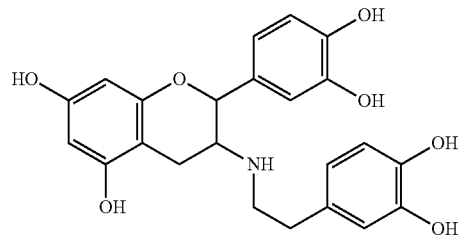
3-deoxy-3-(3,4-dihydroxyphenethyl)(-)-amino- epicatechin
