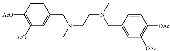
N,N'-bis(3,4-diacetoxybenzyl)-N,N'-dimethylethylenediamine
