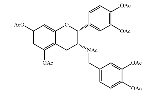
N-acetyl-3-deoxy-3-(3,4-diacetoxybenzyl)-amino-5,7,3',4'-tetraacetyl-epicatechin
