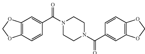
1,4-bis(3,4-methylenedioxybenzoyl) piperazine
