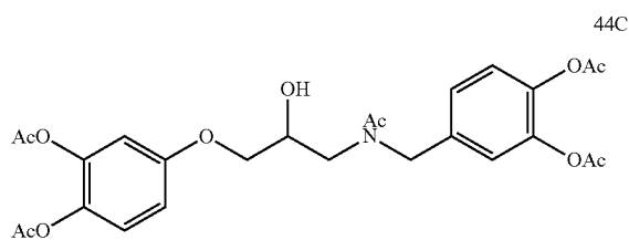
N-acetyl-N-(3,4-diacetoxybenzyl)-3-(3,4-diacetoxyphenoxy)-2-hydroxypropylamine
