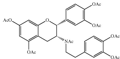
N-acetyl-3-deoxy-3-(3,4-diacetoxyphenethyl)-amino-5,7,3',4'-tetraacetyl-epicatechin
