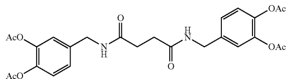
Succinic acid bis(3,4-diacetoxylbenzylamide)
