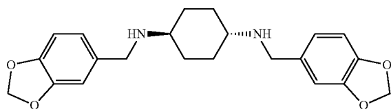
N,N'-bis(3,4-methylenedioxybenzyl)-trans-1,4-diaminocyclohexane
