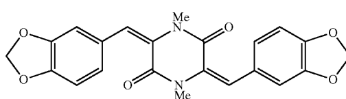
3,6-bis(3,4-methylenedioxybenzylidene)-1,4-dimethyl-2,5-diketopiperazine
