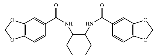
N,N'-bis(3,4-methylenedioxybenzoyl)-trans-diaminocyclohexane
