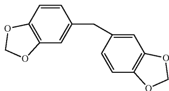
1,1-bis(3,4-methylenedioxyphenyl)methane
