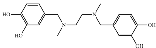
N,N'-bis(3,4-dihydroxybenzyl)-N,N'-dimethylethylenediamine
