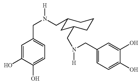
N,N'-bis(3,4-dihydroxybenzyl)-cis-1,3-bis-aminomethylcyclohexane
