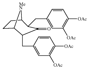
2,4-bis(3,4-diacetoxybenzyl)-3-tropinone
