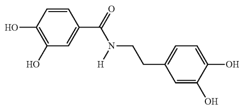
3,4-dihydroxybenzoic acid 3,4-dihydroxyphenethyl amide
