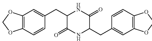
3,6-bis(3,4-methylenedioxybenzyl)-2,5-diketopiperazine
