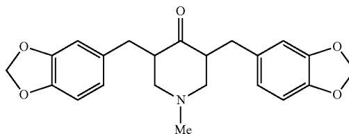
2,5-bis(3,4-methylenedioxybenzyl)-1-methyl-4-piperidinone
