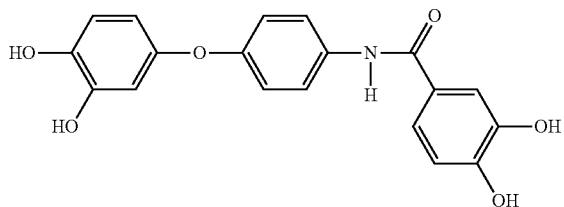
3,4-dihydroxybenzoic acid p-(3,4-dihydroxyphenoxy) anilide
