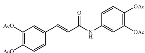
3,4-diacetoxycinnamic acid 3,4- diacetoxylanilide
