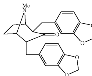
2,4-bis(3,4-methylenedioxybenzyl)-3-tropinone
