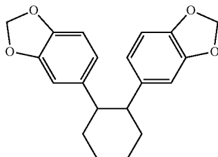
1,2-bis(3,4-methylenedioxyphenyl) cyclohexane
