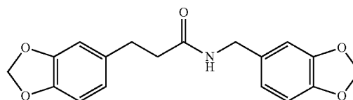
3-(3,4-methylenedioxyphenyl)propionic acid 3,4-methylenedioxybenzylamide
