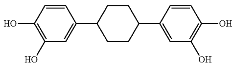
3,7-bis(3,4-dihydroxyphenyl)cyclohexane
