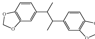
2,3-bis(3,4-methylenedioxyphenyl) butane
