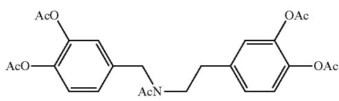
N-acetyl-N-(3,4-diacetoxybenzyl)-3,4-diacetoxyphenethylamine
