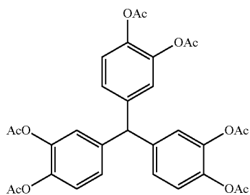
Tris-(3,4-diacetoxyphenyl)methane
