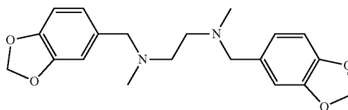
N,N'-bis(3,4-methylenedioxybenzyl)-N,N'-dimethyl-ethylenediamine
