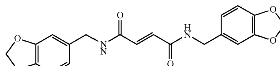
Fumaric acid bis-(3,4-methylenedioxybenzylamide)
