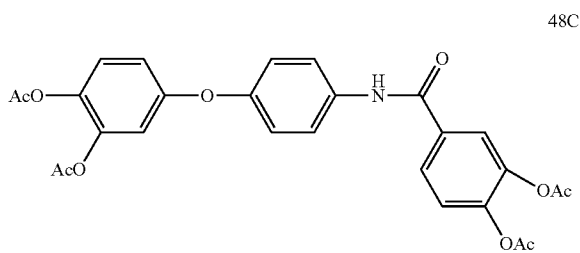
3,4-diacetoxybenzoic acid p-(3,4-diacetoxyphenoxy)anilide
