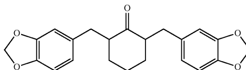
2,6-bis(3,4-methylenedioxybenzyl) cyclohexanone
