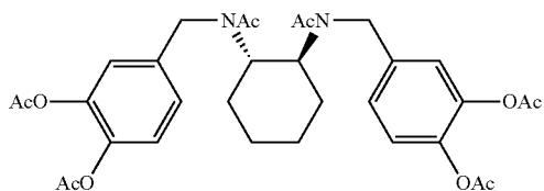
N,N'-bis(acetyl)-bis(3,4-diacetoxybenzyl)-trans-1,2-diaminocyclohexane
