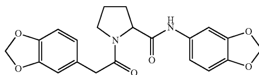
N-(3,4-methylenedioxyphenylacetyl)-proline-3,4-methylenedioxyanilide
