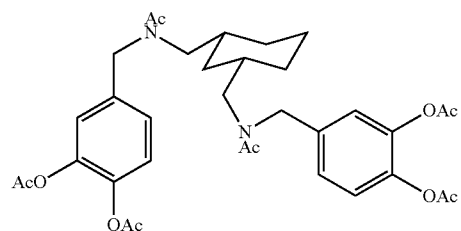
N,N'-bis(acetyl)-bis(3,4-diacetoxybenzyl)-cis-1,3-bis-aminomethylcyclohexane
