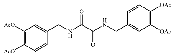
Oxalic acid bis(3,4-diacetoxylbenzylamide)
