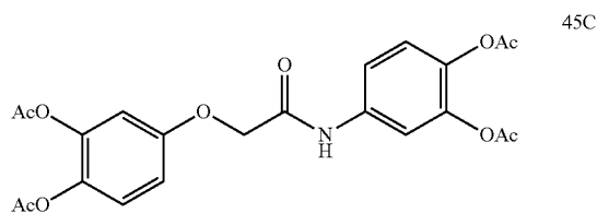
3,4-diacetoxyphenoxyacetic acid 3,4-diacetoxyanilide
