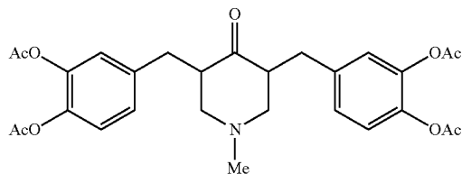
3,5-bis(3,4-diacetoxybenzyl)-1-methyl-4-piperidinone
