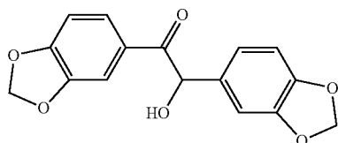
bis(3,4-methylenedioxy)benzoin
