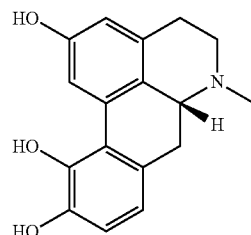
6-Methyl-5,6,6a,7-tetrahydro-4H-dibenzo[de,g]quinoline-2,10,11-triol
