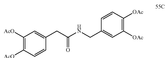
3,4-diacetoxyphenylacetic acid 3,4-diacetoxylbenzylamide
