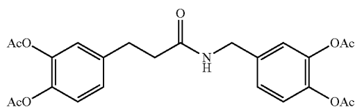
3-(3,4-diacetoxyphenyl)propionic acid 3,4-diacetoxylbenzylamide
