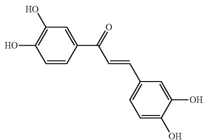
3,4,3',4'-Tetrahydroxychalcone
