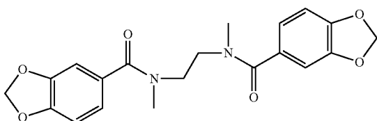
N,N'-bis(3,4-methylenedioxybenzoyl)-N,N'-dimethyl(-)ethylenediamine
