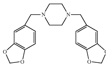
1,4-bis(3,4-methylenedioxybenzyl)piperazine
