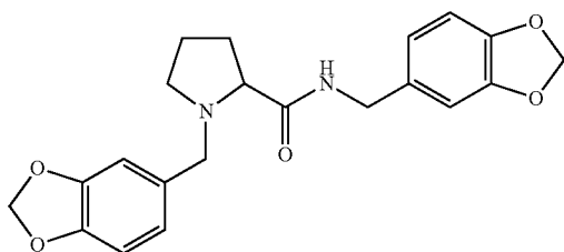
N-(3,4-methylenedioxybenzyl)proline-3,4-methylenedioxybenzylamide
