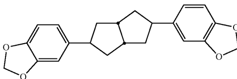
3,7-bis(3,4-methylenedioxyphenyl) bicyclo[3,3,0]octane
