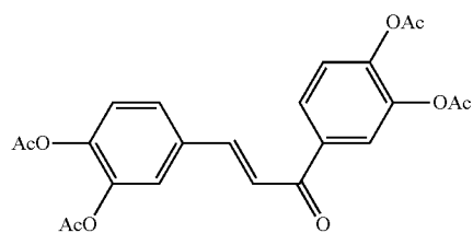
bis(3,4-diacetoxy)chalcone
