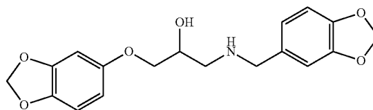
N-(3,4-methylenedioxybenzyl)-3-(3,4-methylenedioxy(-) phenoxy)-2-hydroxypropylamine
