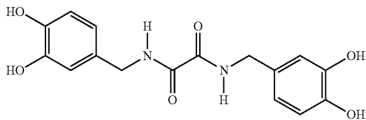
Oxalic acid-bis(3,4-dihydroxybenzyl(-) amide)
