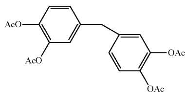
1,1-bis(3,4-diacetoxyphenyl)methane
