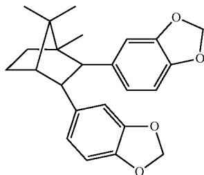
2,3-bis(3,4-methylenedioxyphenyl)-1,7,7- trimethyl-bicyclo[2,2,1]heptane
