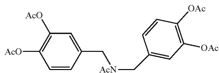
N-acetyl-bis-(3,4-diacetoxybenzyl)-amine
