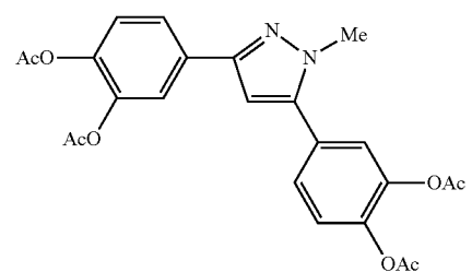
3,5-bis(3,4-diacetoxyphenyl)-1-methyl-1H-pyrazoline
