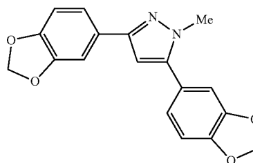
3,5-bis(3,4-methylenedioxyphenyl)-1-methyl-1H-pyrazole
