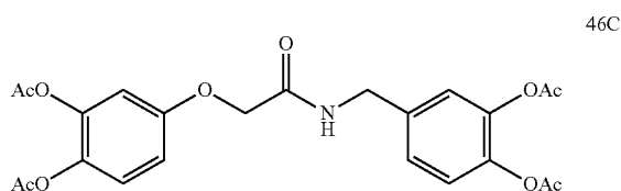
3,4-diacetoxyphenoxyacetic acid 3,4-diacetoxylbenzylamide
