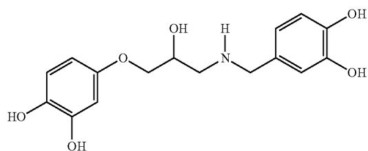
N-(3,4-dihydroxybenzyl)-3-(3,4-dihydroxyphenyl)propan-1-amine
