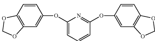
2,6-bis(3,4-methylenedioxyphenoxy)pyridine
