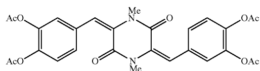
3,6-bis(3,4-diacetoxybenzylidene)-1,4-dimethyl-2,5-diketopiperazine
