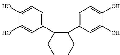
1,2-bis(3,4-dihydroxyphenyl)cyclohexane
