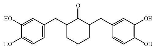
2,6-bis(3,4-dihydroxybenzyl)cyclohexanone
