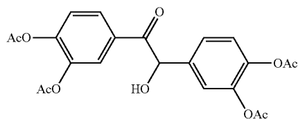
bis(3,4-diacetoxy)benzoin
