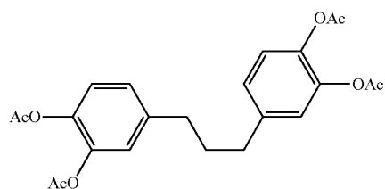
1,3-bis(3,4-diacetoxyphenyl)propane
