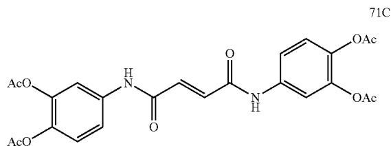
Fumaric acid bis-(3,4-diacetoxyanilide)
