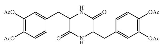
3,6-bis(3,4-diacetoxybenzyl)-2,5-diketopiperazine
