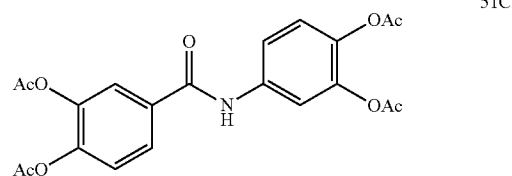
3,4-diacetoxybenzoic acid 3,4-diacetoxyanilide
