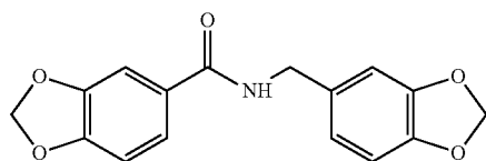
3,4-methylenedioxybenzoic acid 3,4-methylenedioxybenzylamide
