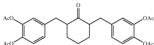
2,6-bis(3,4-diacetoxybenzyl) cyclohexanone
