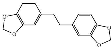
1,2-bis(3,4-methylenedioxyphenyl)ethane
