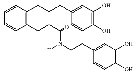
2-(3,4-dihydroxybenzyl)isoquinoline-3-carboxylic acid 3,4-dihydroxyphenethylamide
