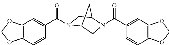
2,5-bis(3,4-methylenedioxybenzoyl)-2,5-diaza[2,2,1]-bicycloheptane
