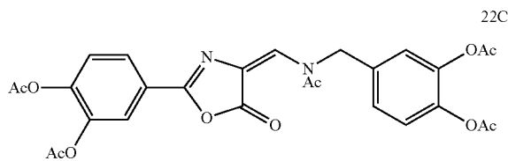
N-acetyl-4-(3,4-diacetoxybenzylamino-methylene)-2-(3,4-diacetoxyphenyl)-oxazolin-5-one
