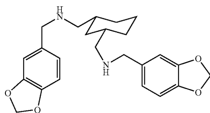
N,N'-bis(3,4-methylenedioxybenzyl)-cis-1,3-bis-aminomethylcyclohexane
