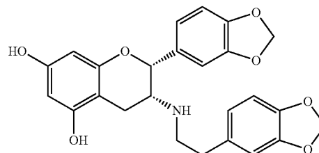
3-deoxy-3-(3,4-methylenedioxyphenethyl)-aminoepicatechin
