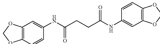
Succinic acid bis(3,4-methylenedioxyanilide)
