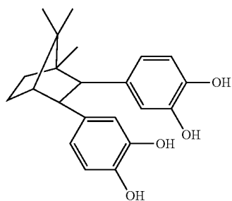
2,3-bis(3,4-dihydroxyphenyl)-1,7,7-trimethyl- bicyclo[2.2.1]heptane
