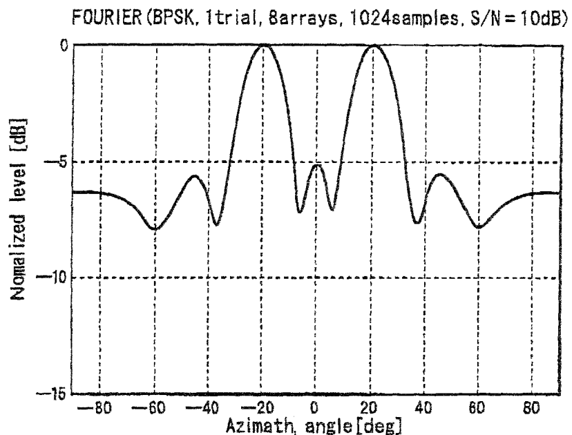
(a) DIRECTION ESTIMATION RESULT FOR PATH 1=20°, PATH 2=-20°
