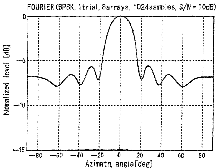
(b) DIRECTION ESTIMATION RESULT FOR PATH 1=5°, PATH 2=-5°
