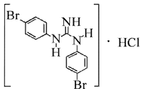
Bromo-DTG
