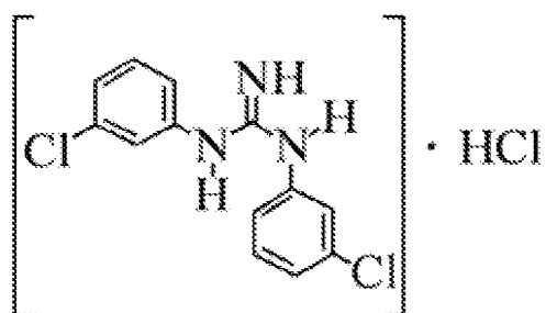
Chloro-DTG
