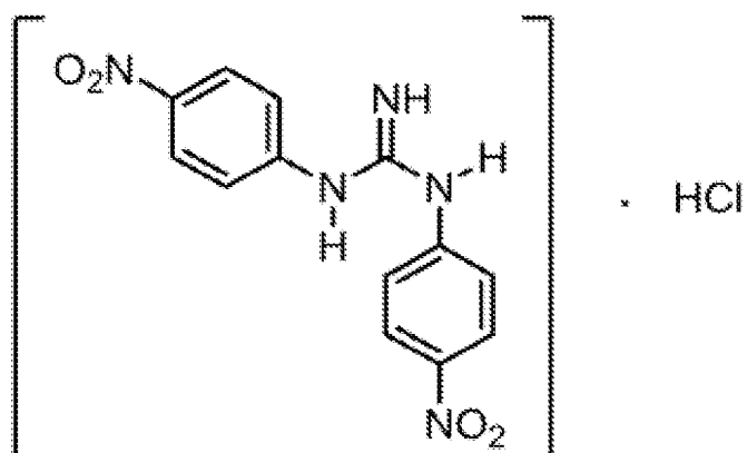
Chloro-DTG
