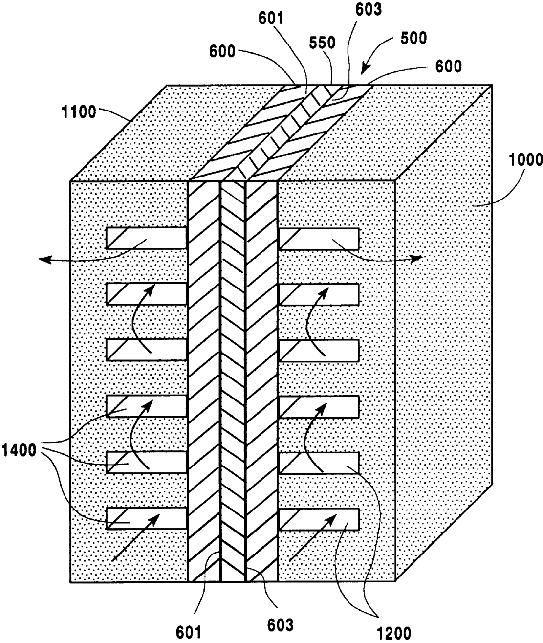
Fig. 9 (PRIOR ART)
