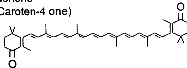
Canthaxanthin ( \beta,\beta -Caroten-4,4'-dione)
