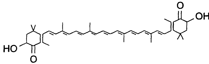
Astaxanthin (3,3' -Dihydroxy- \beta,\beta -Carotene-4,4'-dione)
