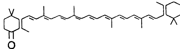
Echinenone ( \beta,\beta -Caroten-4 one)
