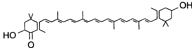
Adonixanthin (3,3' -Dihydroxy- \beta,\beta -Carotene-4-one)
