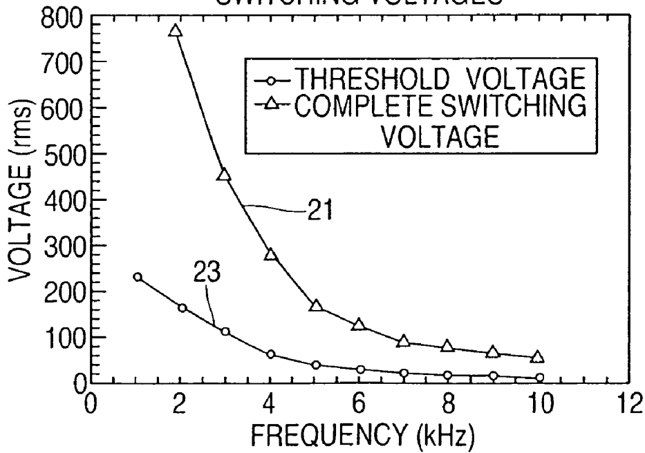
FREQUENCY DEPENDENCE OF GRATING SWITCHING VOLTAGES
