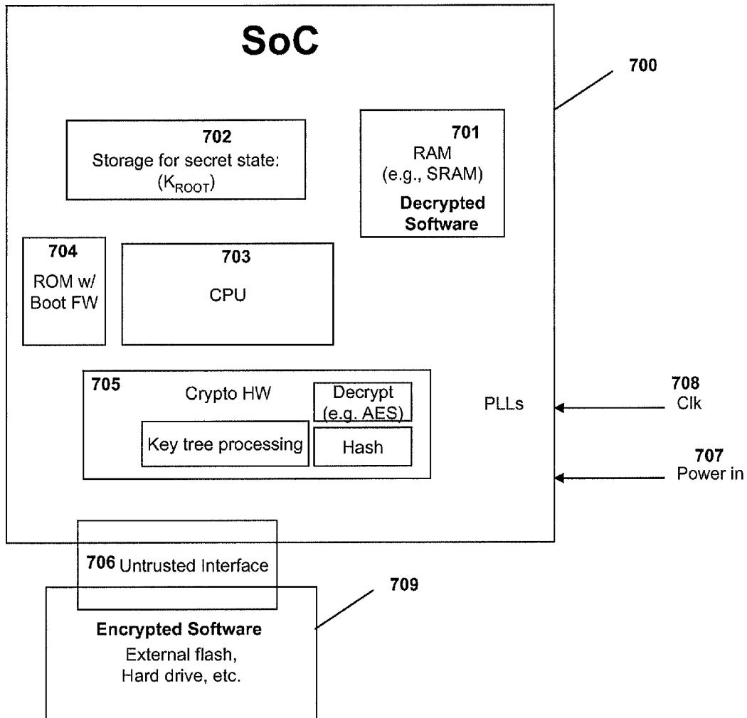
Figure 7: Firmware loading
