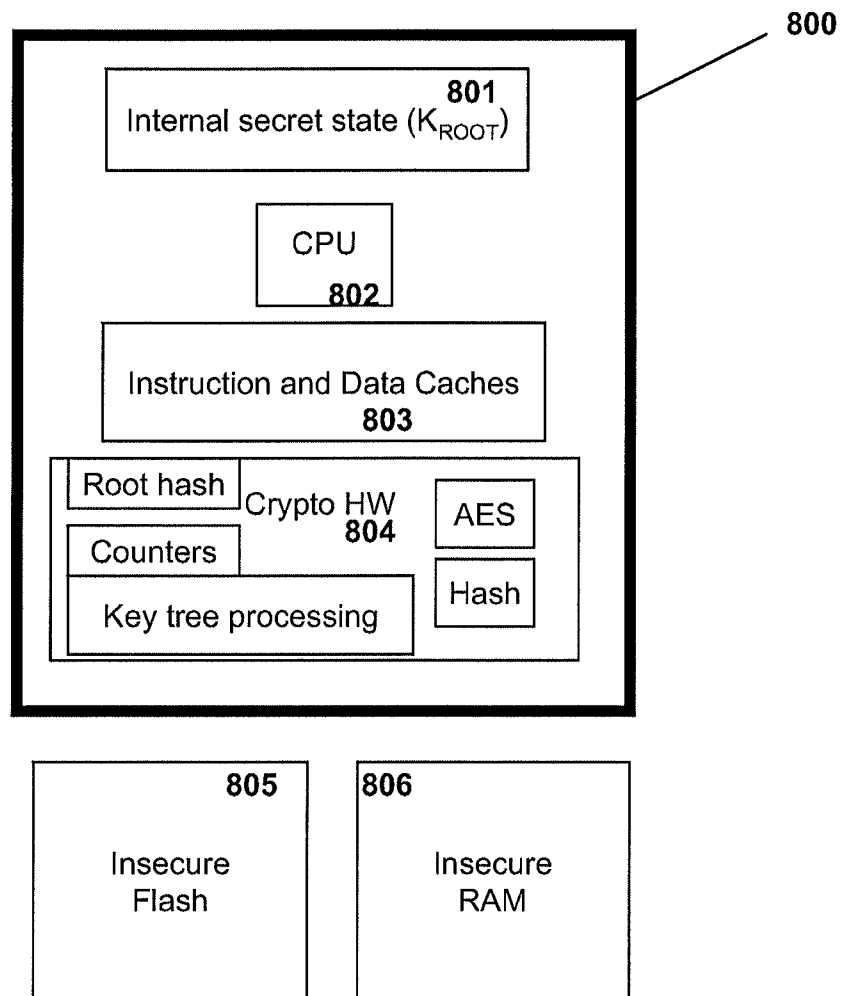
Figure 8: Secure CPU
