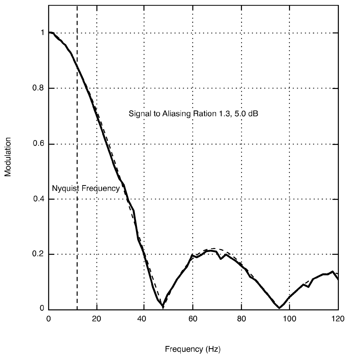
Temporal Modulation Transfer Functions (24 fps, 180 Degree Shutter)
