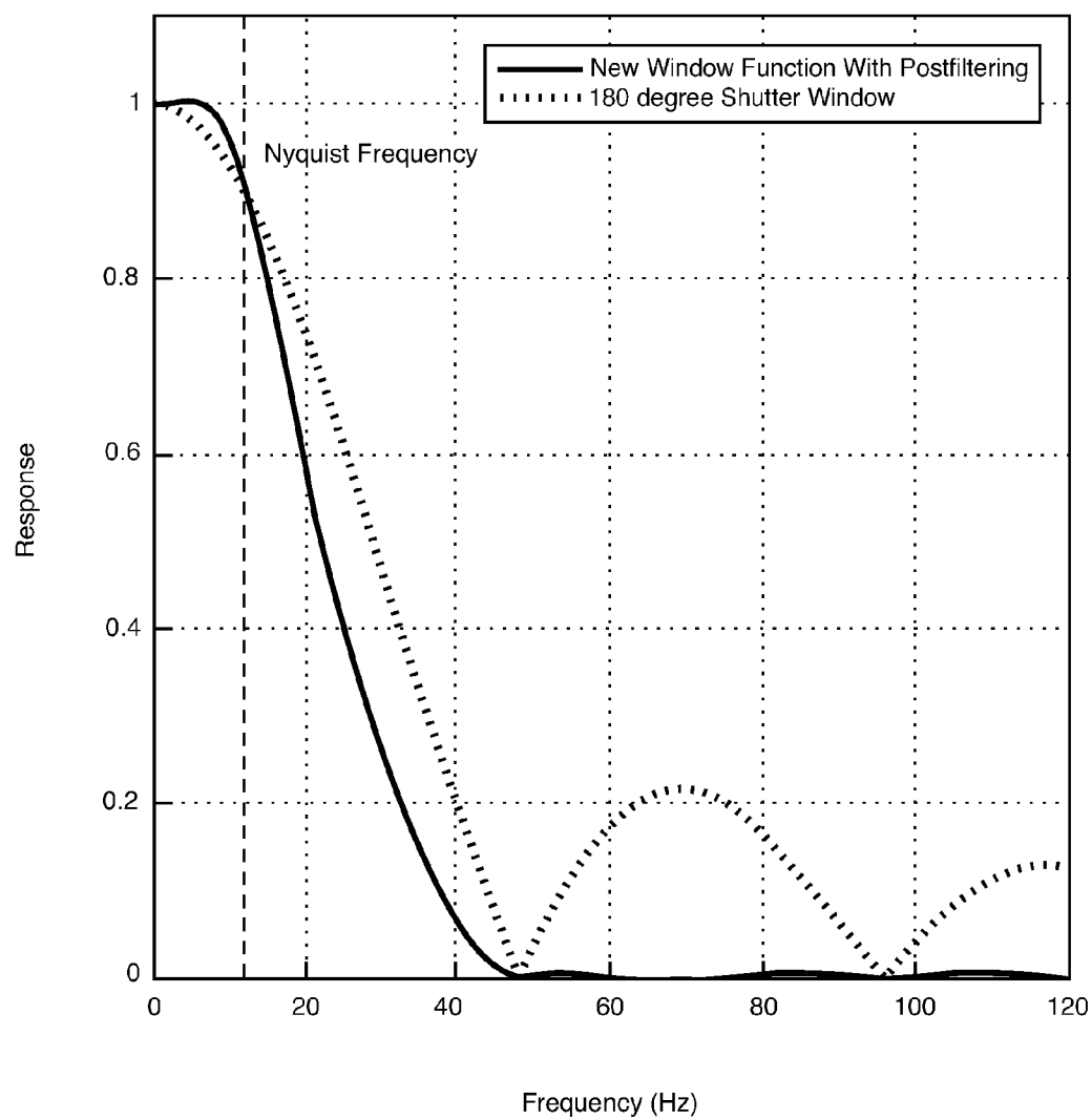
Modulation Transfer Function for Exposure Window With Postfiltering
