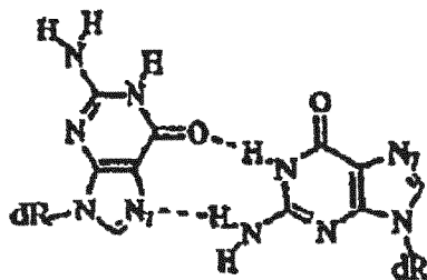
GG base pair
