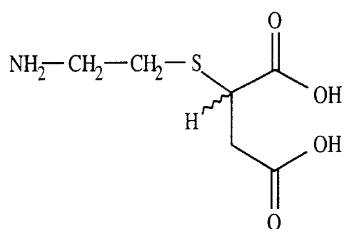
S -2-( 2R , 2S -SUCCINYL)-CYSTEAMINE
