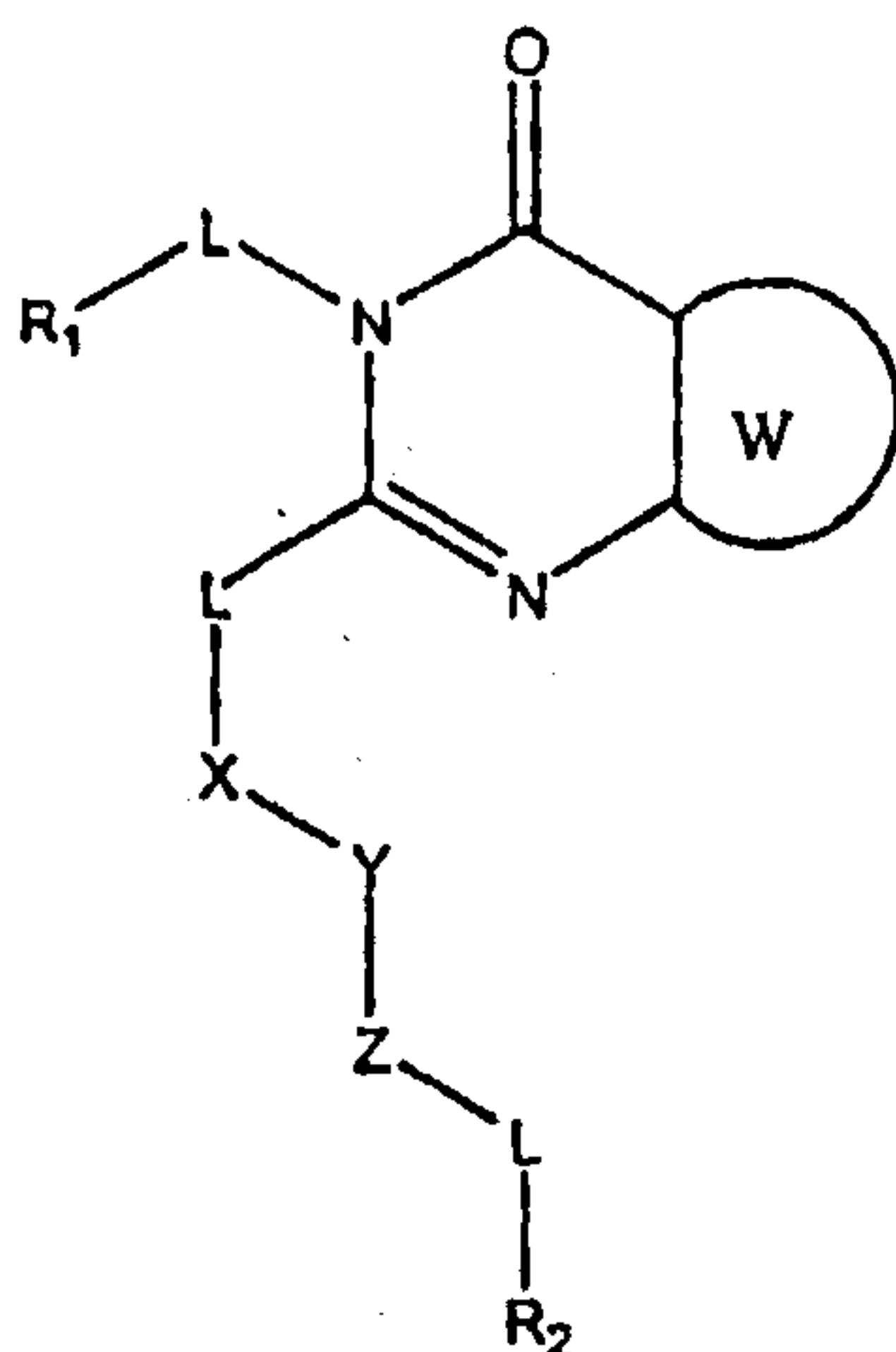
Formula II
