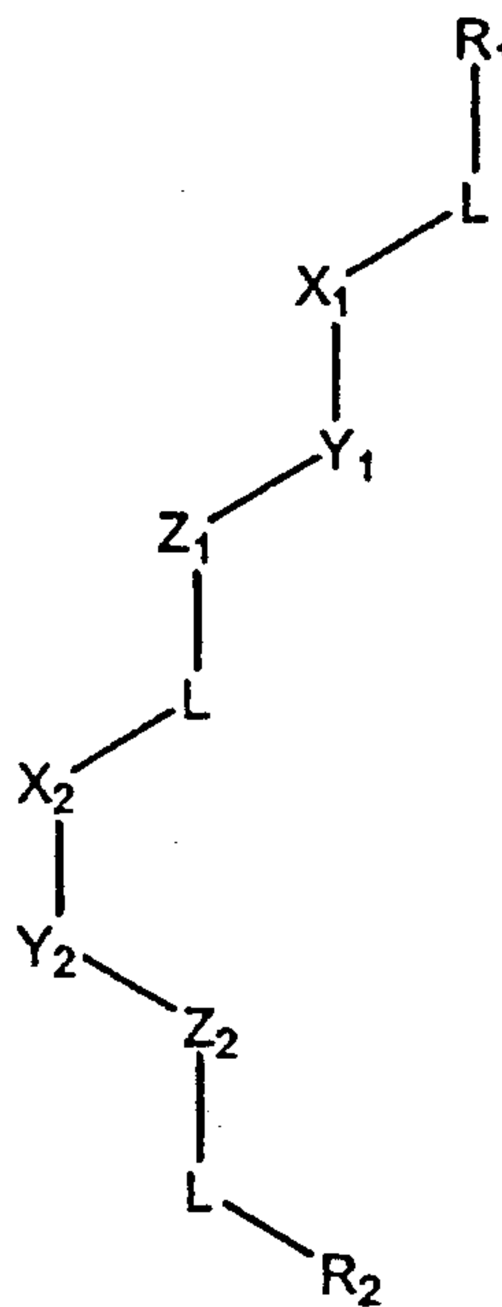
Formula I
