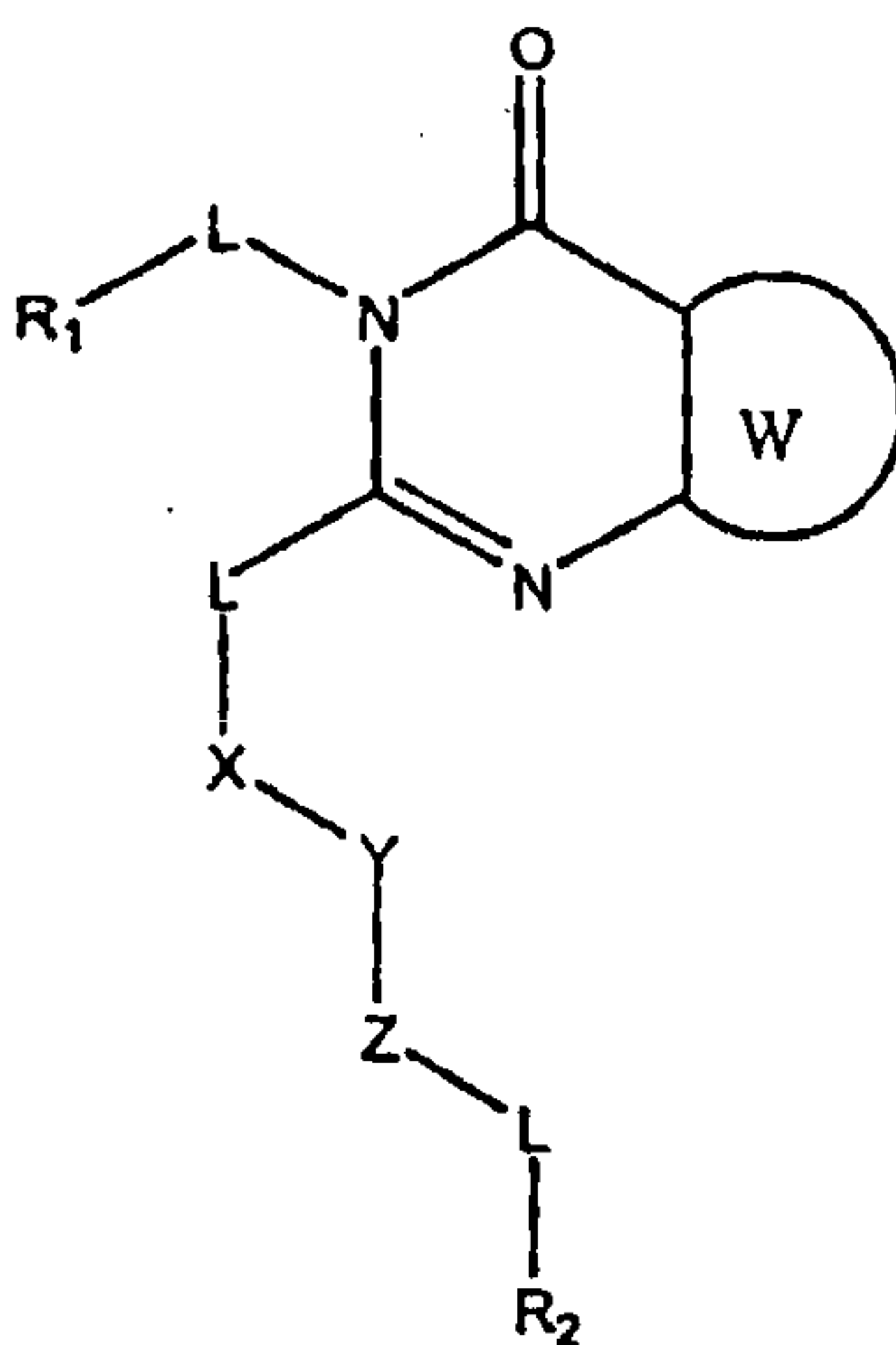
15 Formula II
