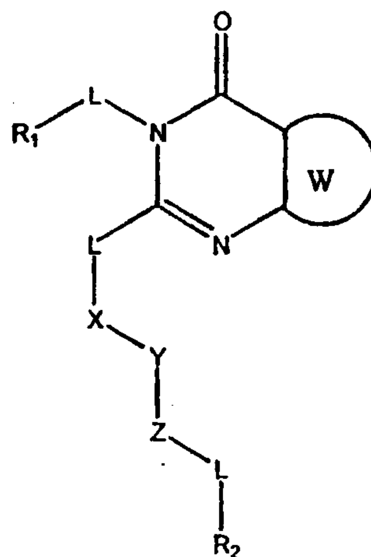
Formula II
