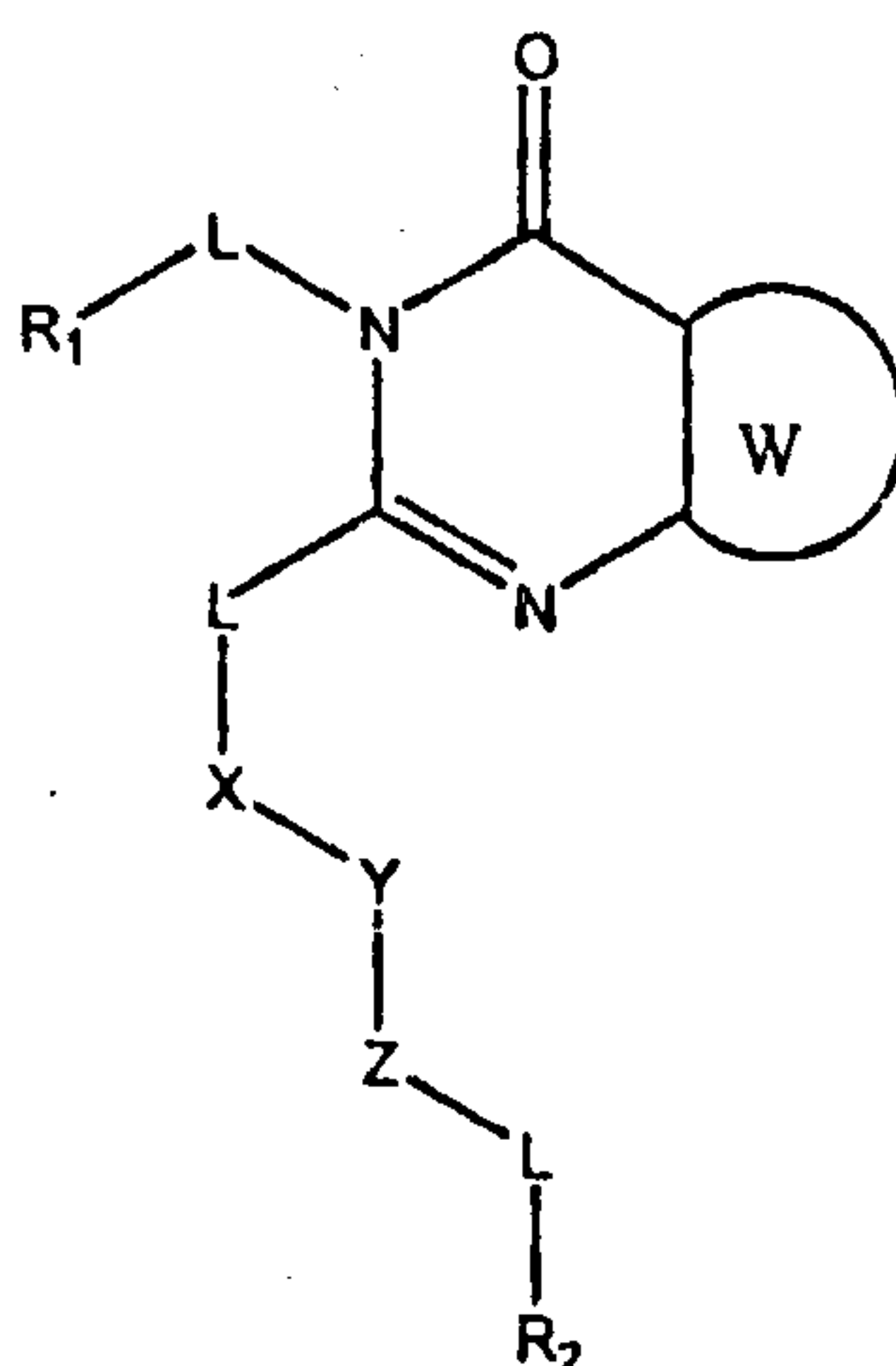
Formula II
