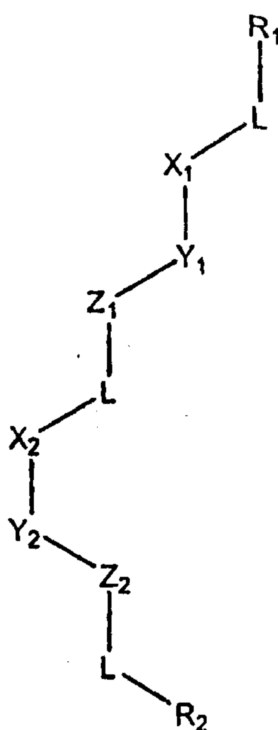
Formula I
