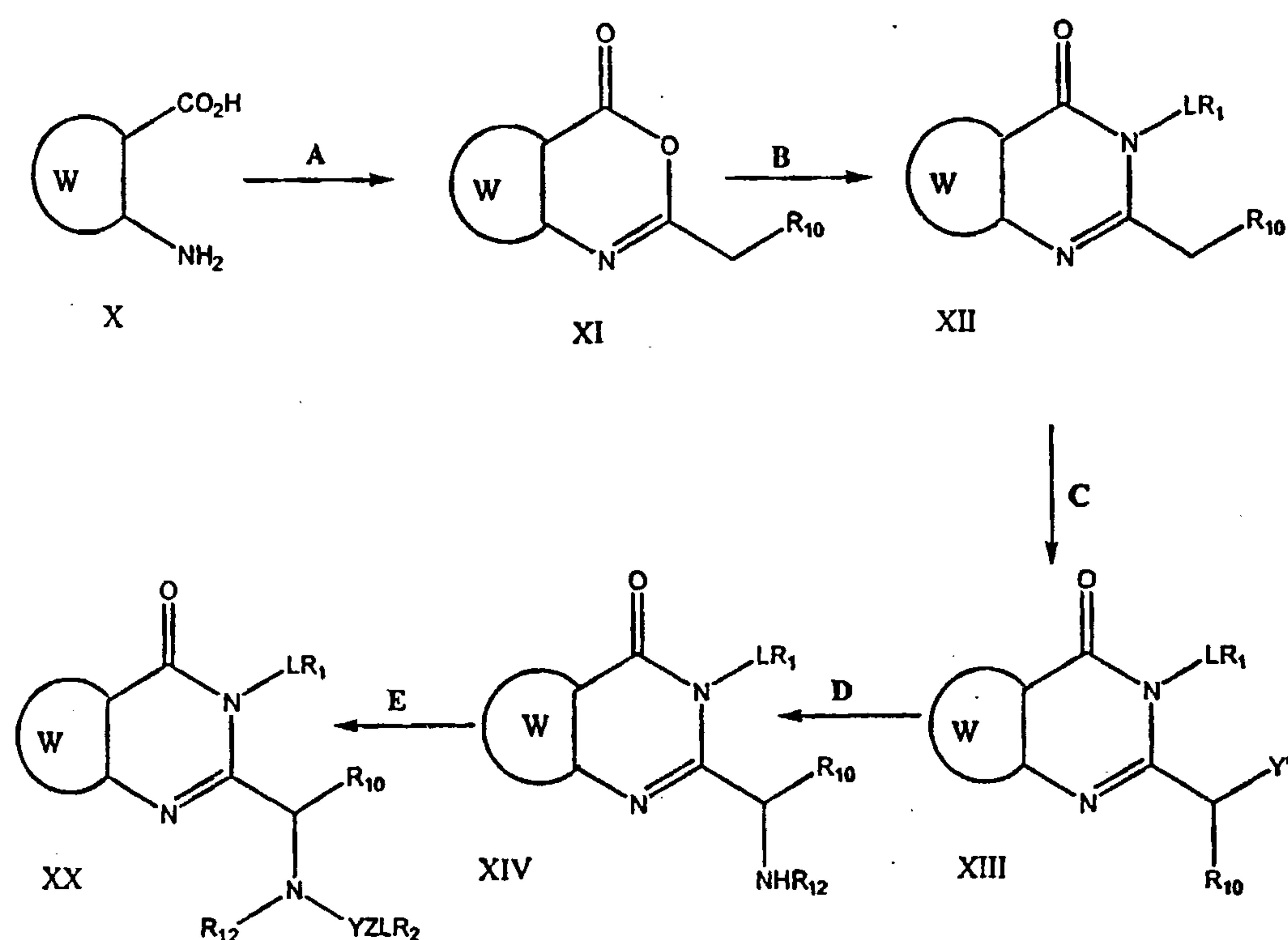
Scheme I
