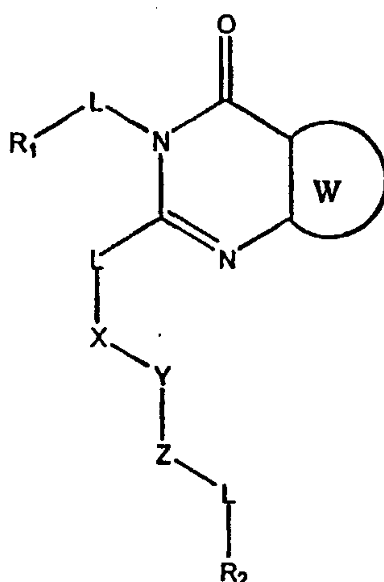
Formula II
