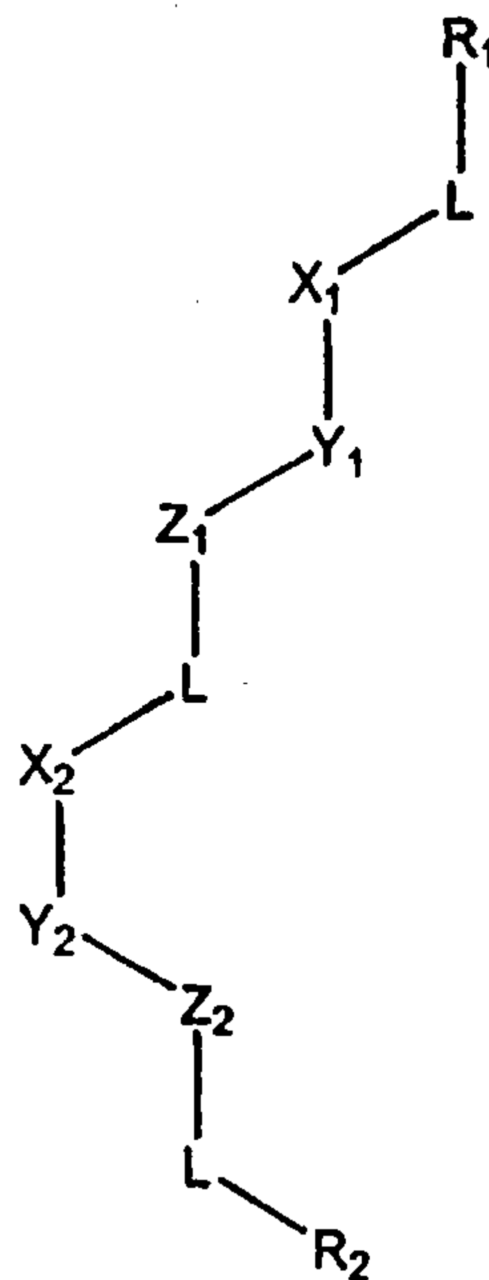
Formula I
