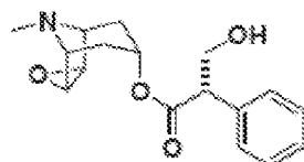
Scopolamine non-selective muscarinic receptor antagonist
