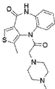
Telenzepine M1-selective muscarinic receptor antagonist
