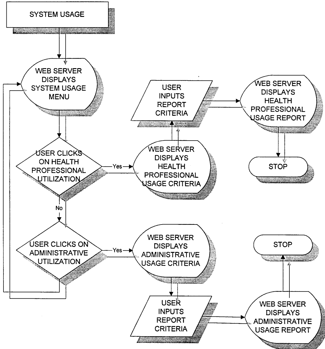
Figure 69: System Usage Flowchart
