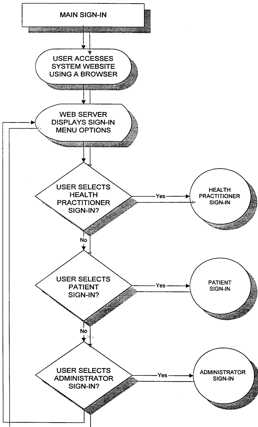
Figure 5: Main Sign-in Flowchart
