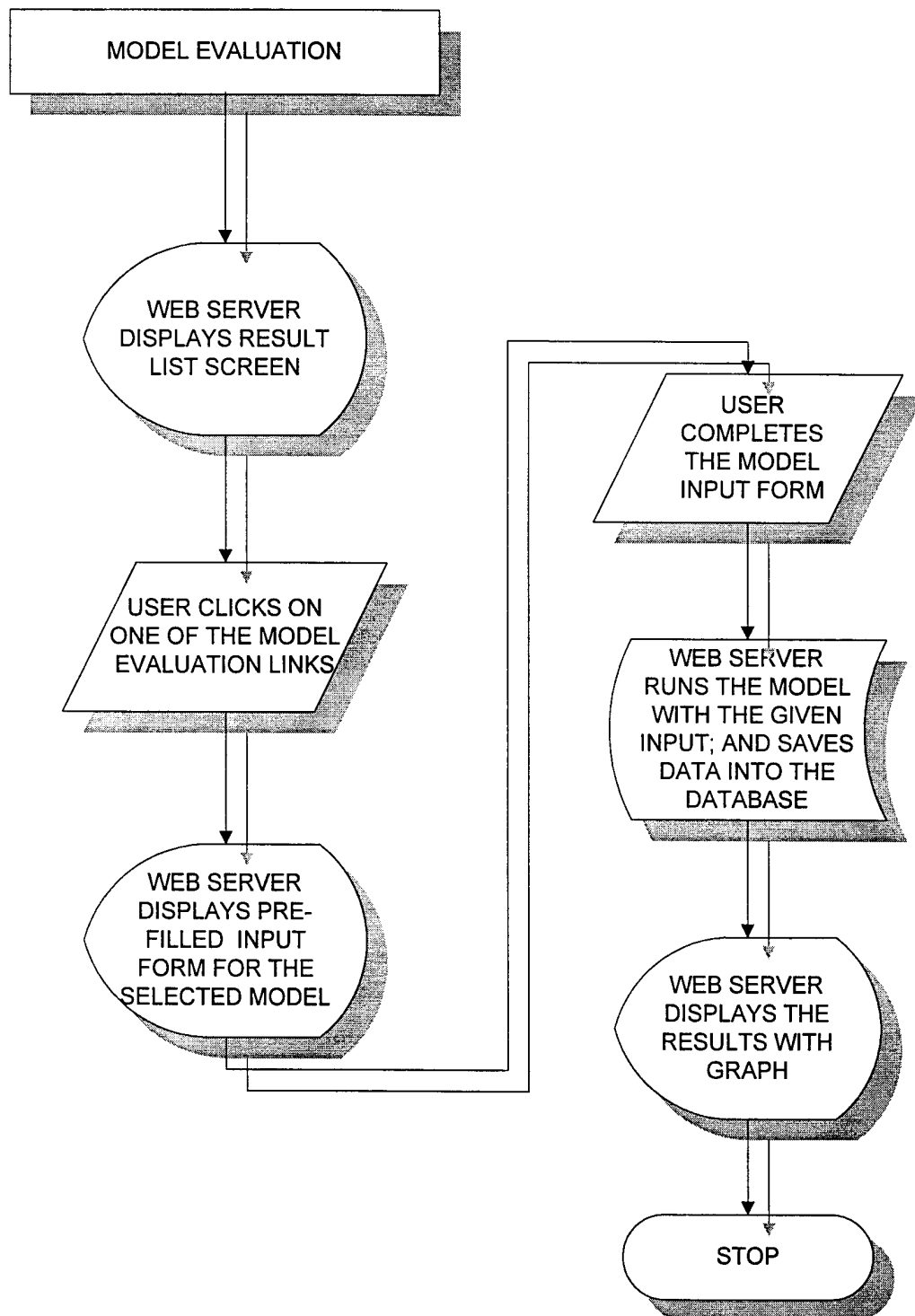
Figure 87: Model Evaluation Flowchart
