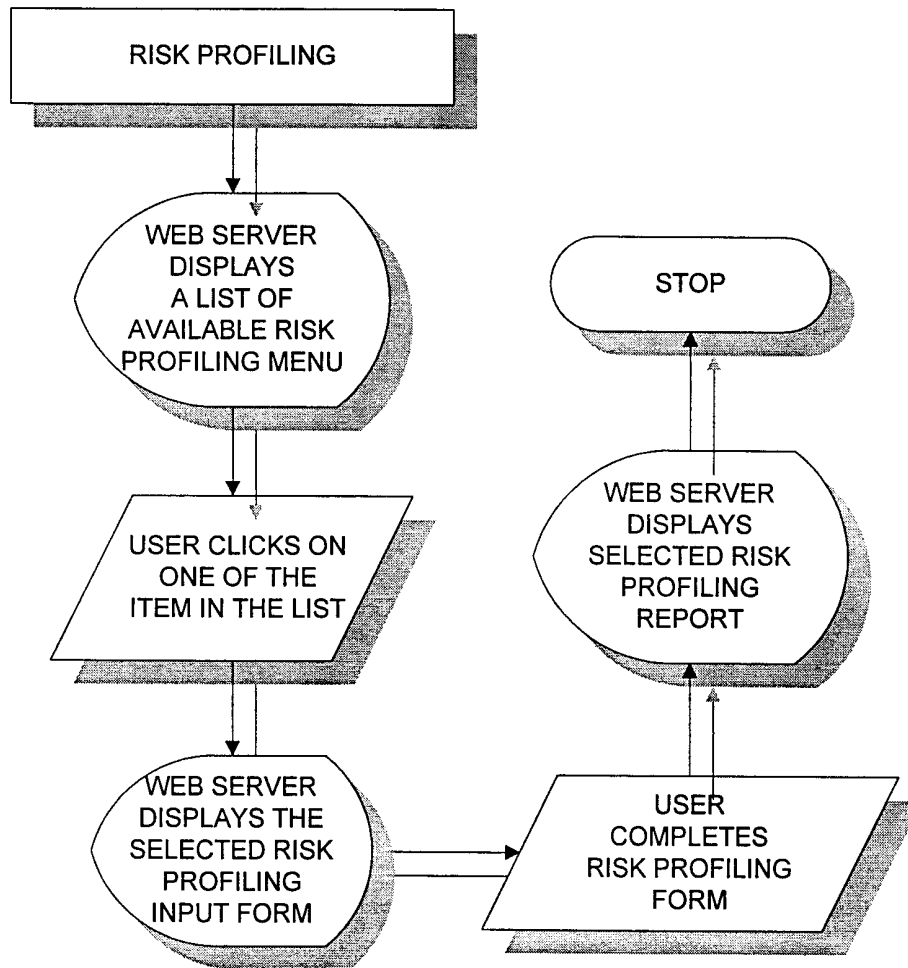
Figure 86: Risk Profiling Flowchart
