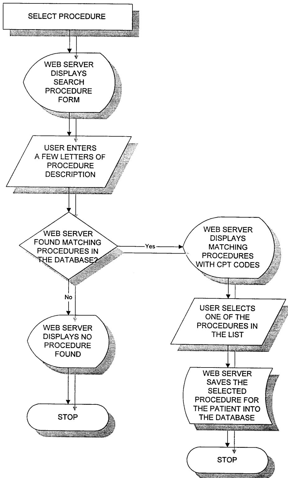
Figure 32: Select Procedure Flowchart
