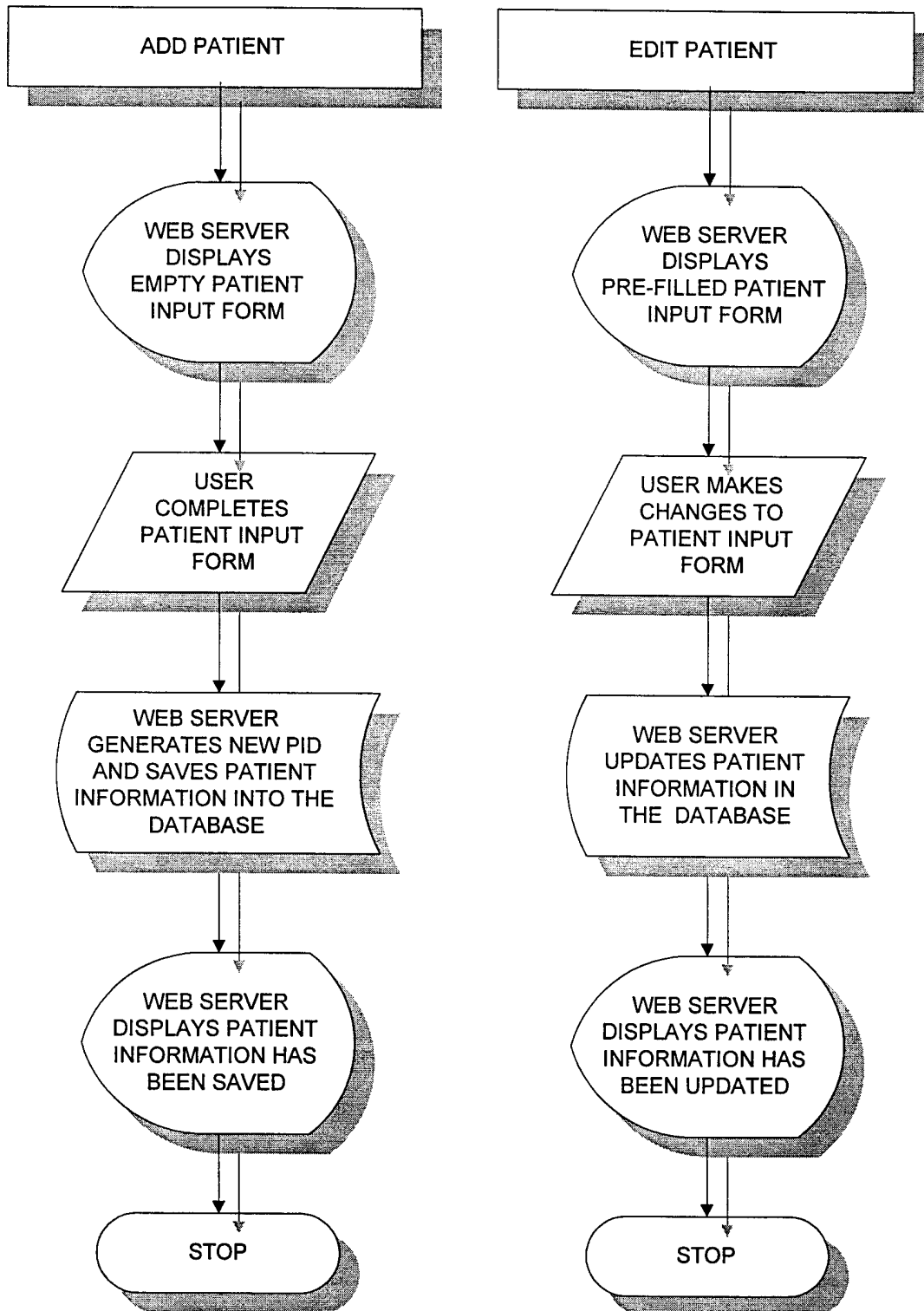
Figure 31: Add/Edit Patient Flowchart
