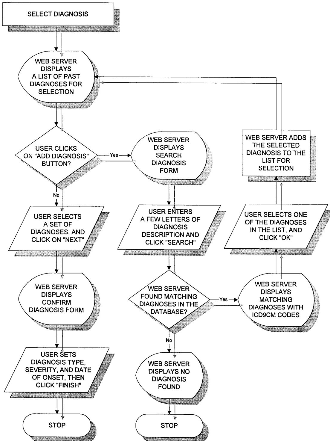
Figure 21: Select Diagnosis Flowchart
