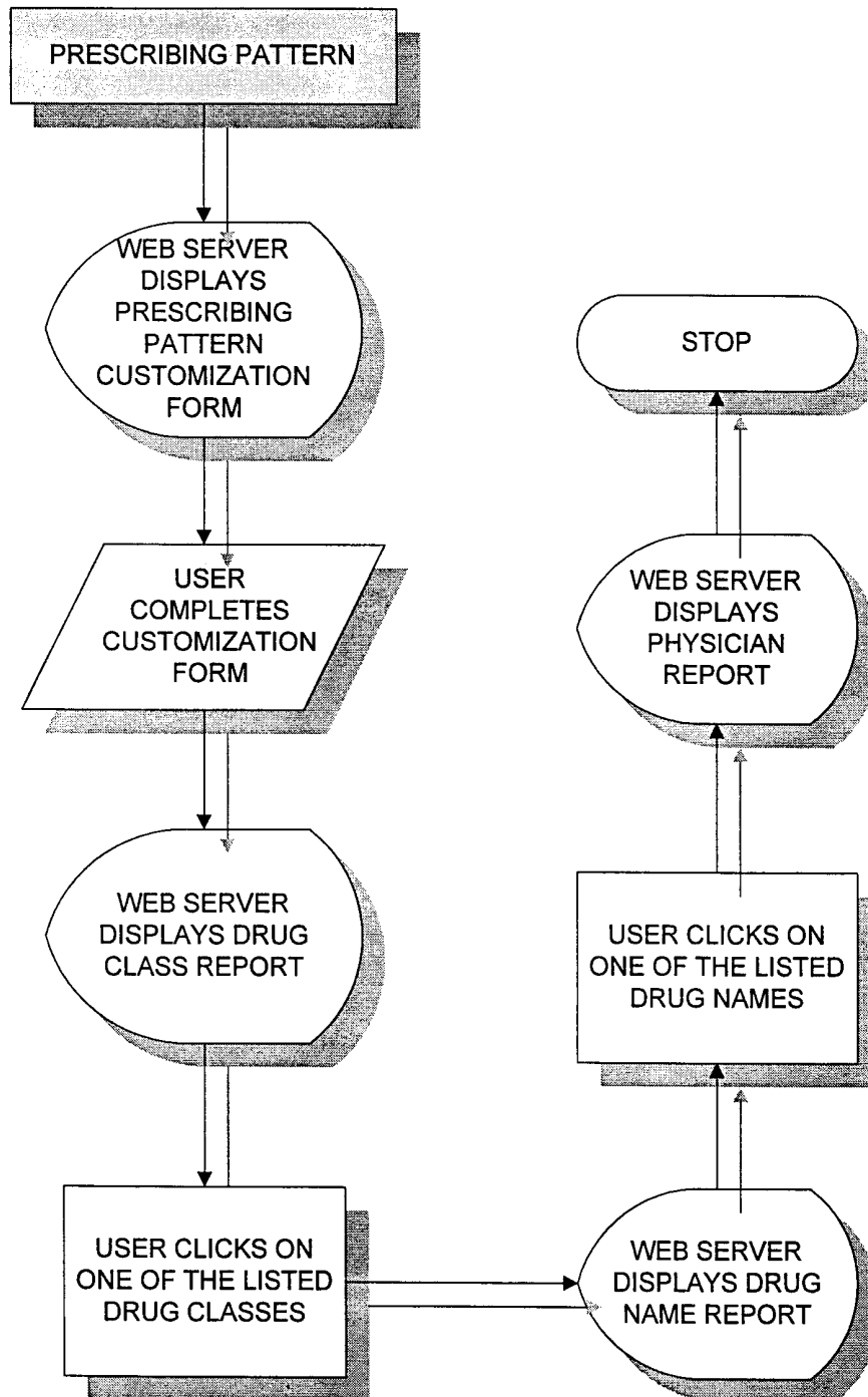
Figure 74: Prescribing Pattern Flowchart
