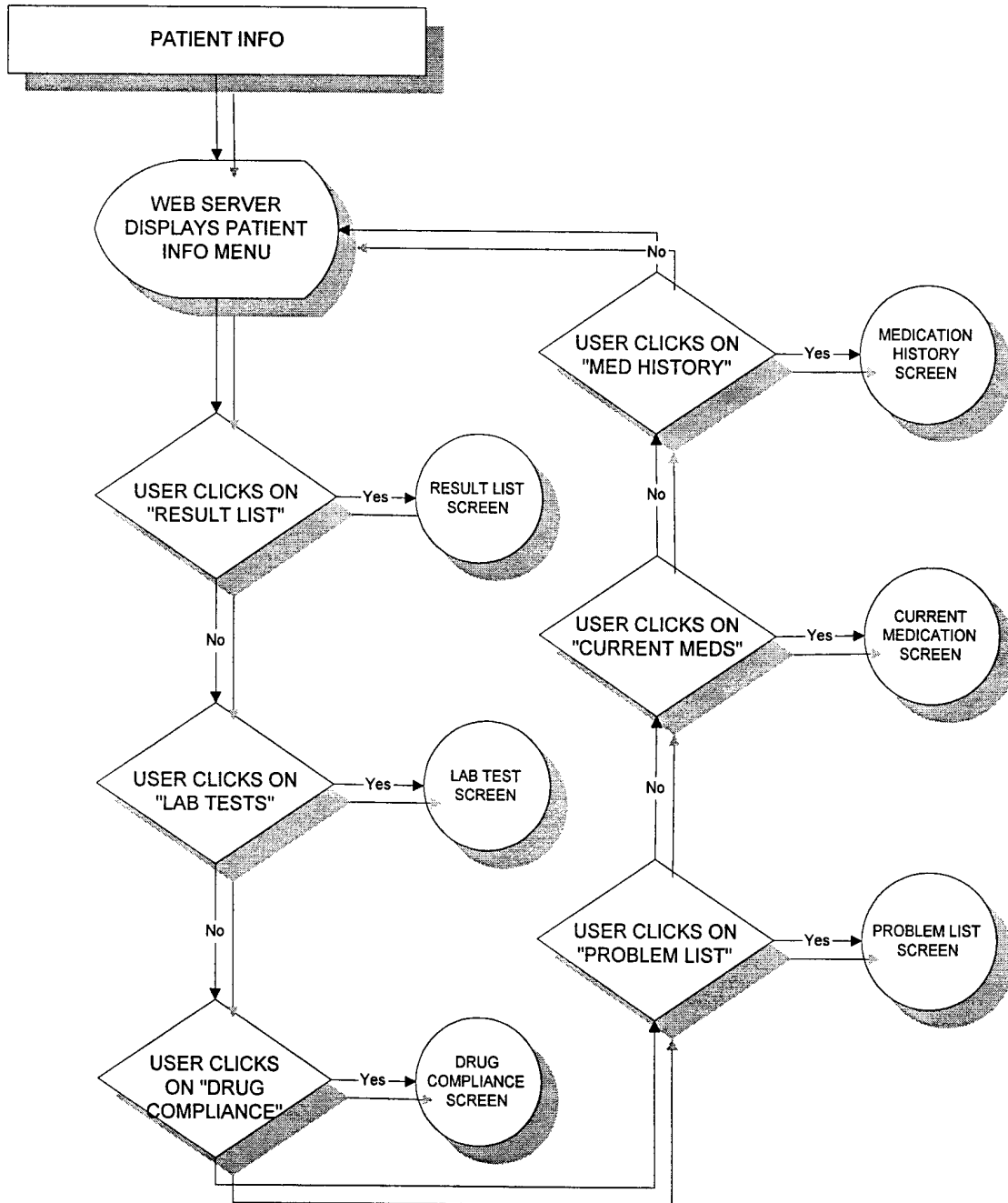
Figure 28: Patient Info Flowchart
