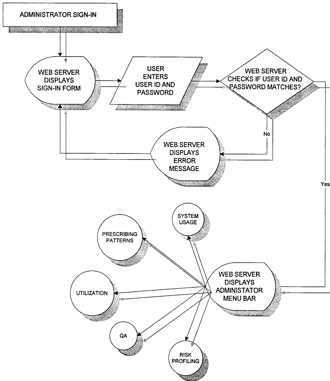
Figure 63: Administrator Sign-in Flowchart
