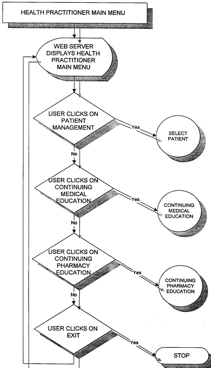
Figure 10: Health Practitioner Main Menu Flowchart
