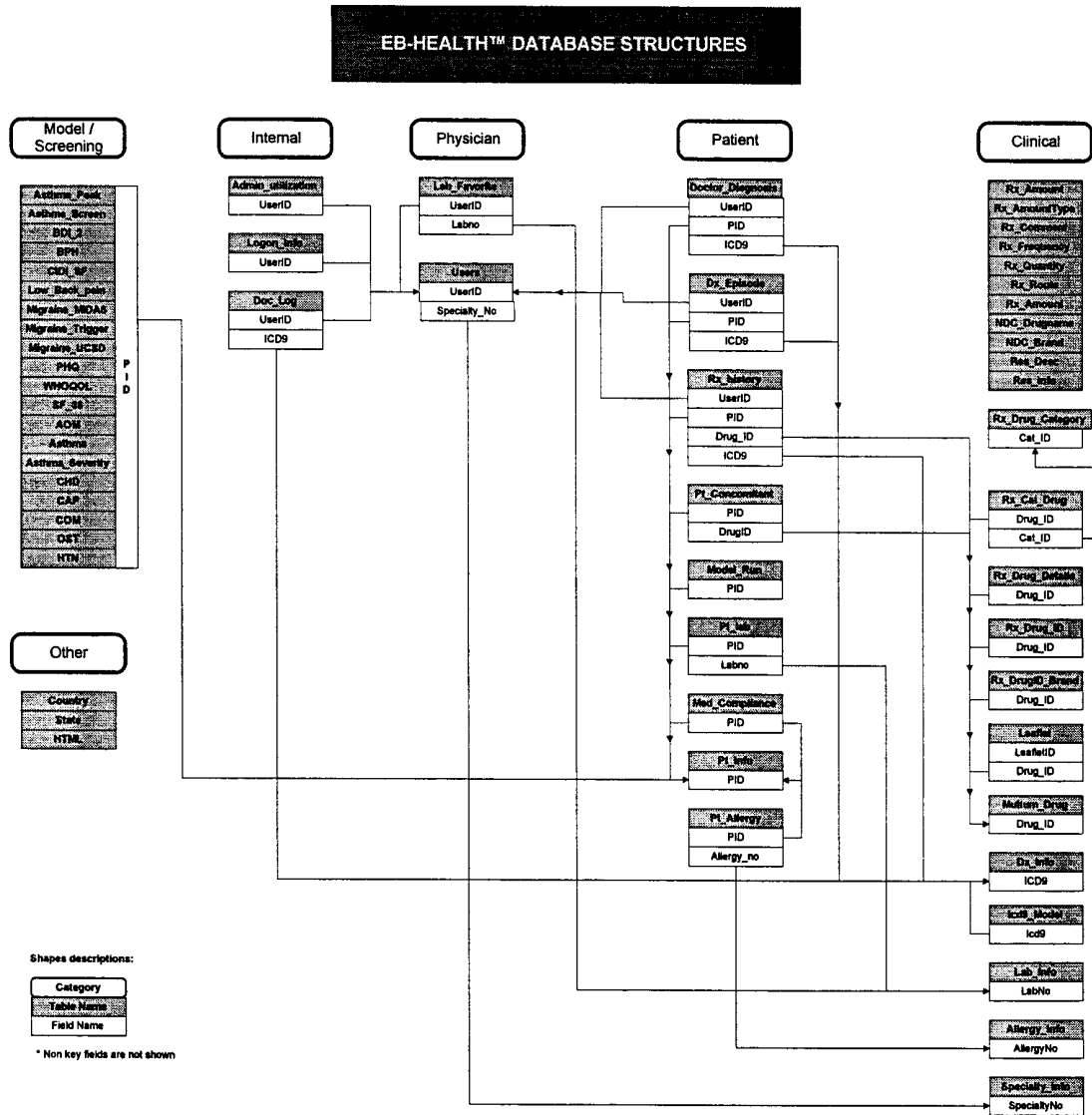
Figure 13: Database Structures
