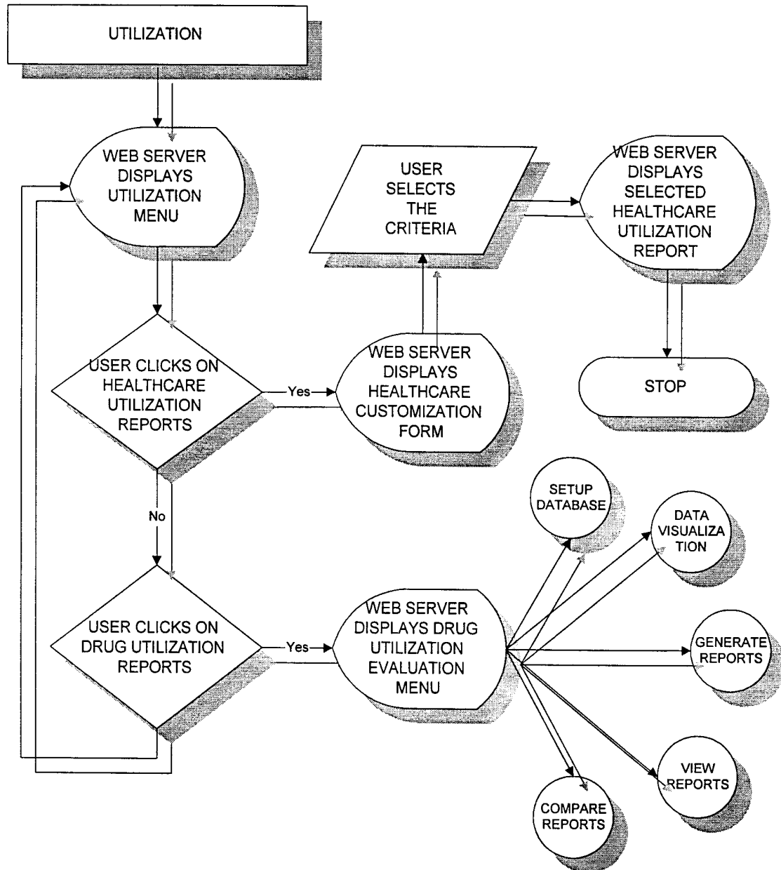
Figure 81: Utilization Flowchart
