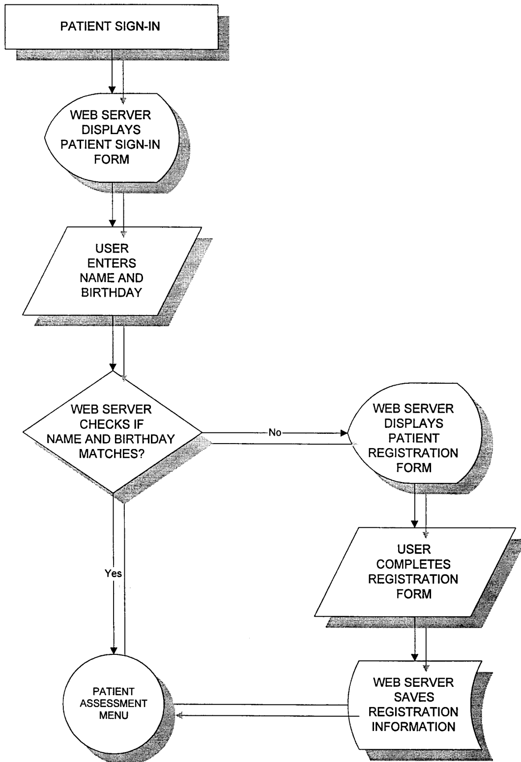
Figure 58: Patient Sign-in Flowchart
