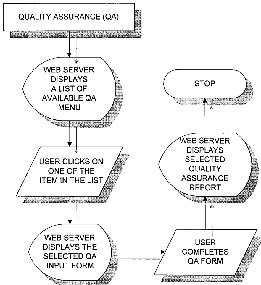
Figure 83: Quality Assurance Flowchart
