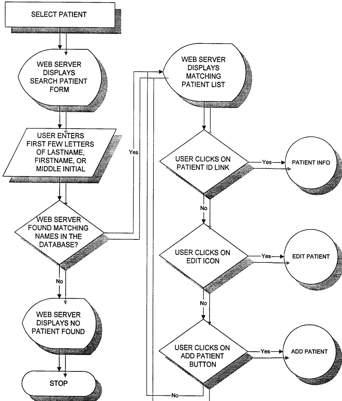
Figure 15: Select Patient Flowchart
