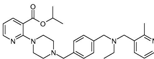
1-piperazinyl)-3-pyridinecarboxylate
