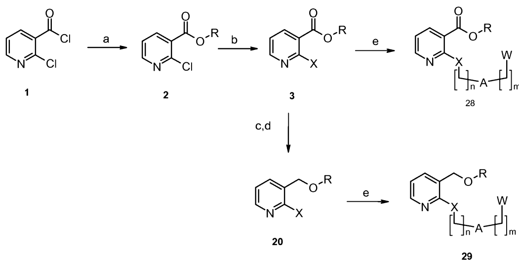
Scheme 7
