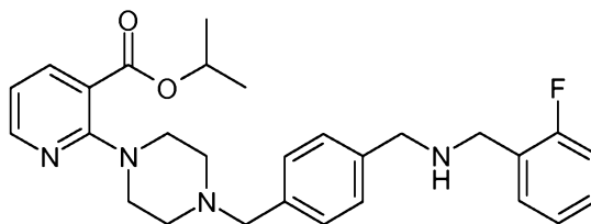
piperazinyl)-3-pyridinecarboxylate
