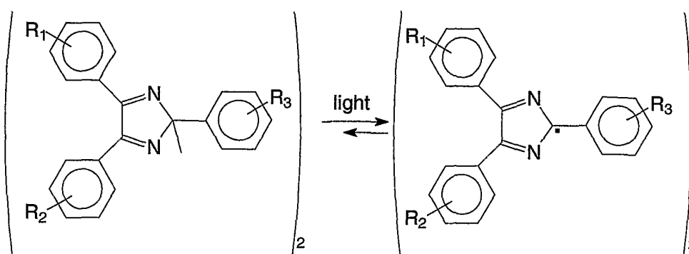
5 Scheme 3: Photochromic dyes
