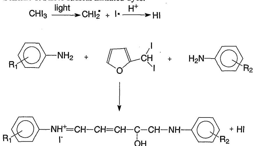
Scheme 1. Photo radical initiated dyes.
