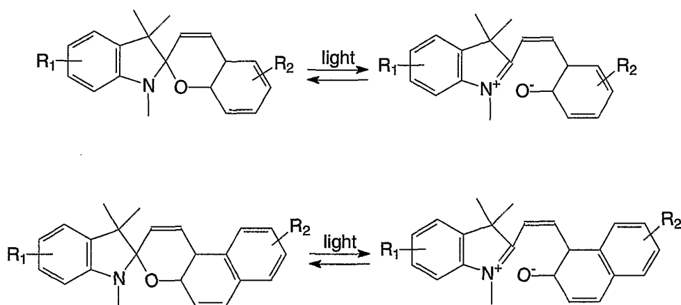
5 Scheme 3: Photochromic dyes
