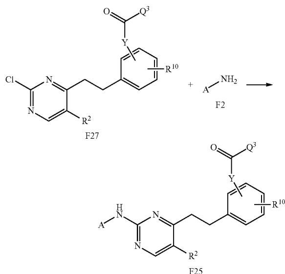
Scheme U
