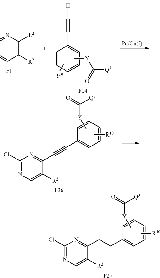
Scheme T
