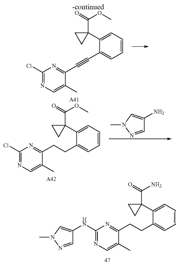
(c) 1-(2-(2-(5-Methyl-2-((1-methyl-1H-pyrazol-4-yl)amino)pyrimidin-4-yl)ethyl)phenyl)cyclopropanecarboxamide (47)
