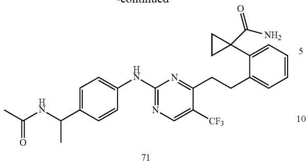
1-(2-(2-(2-(4-(1-Acetamidoethyl)phenylamino)-5-(trifluoromethyl)pyrimidin-4-yl)ethyl)phenyl)cyclopropanecarboxamide (71)
