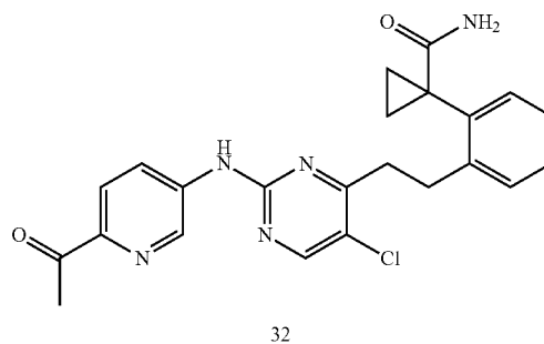
1-(2-(2-(2-((6-Acetylpyridin-3-yl)amino)-5-chloropyrimidin-4-yl)ethyl)phenyl)cyclopropanecarboxamide (32)
