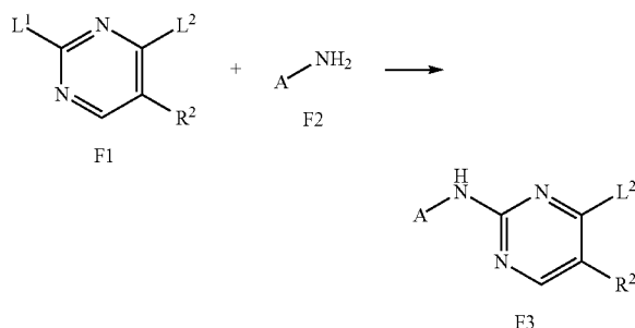
Scheme A
