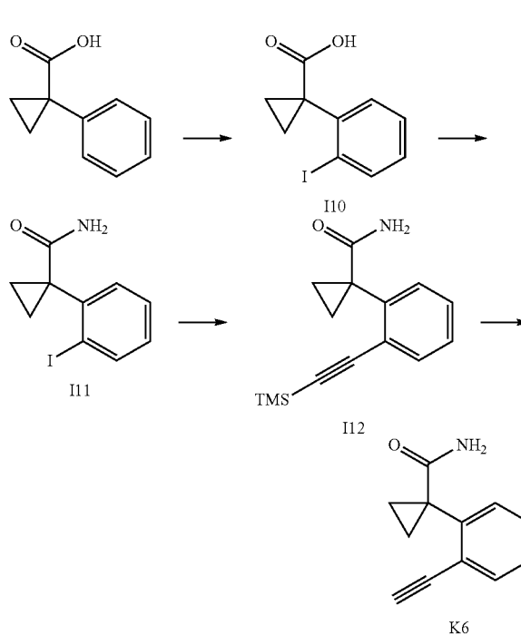
(a) 1-(2-Iodophenyl)cyclopropanecarboxylic Acid (I10)
