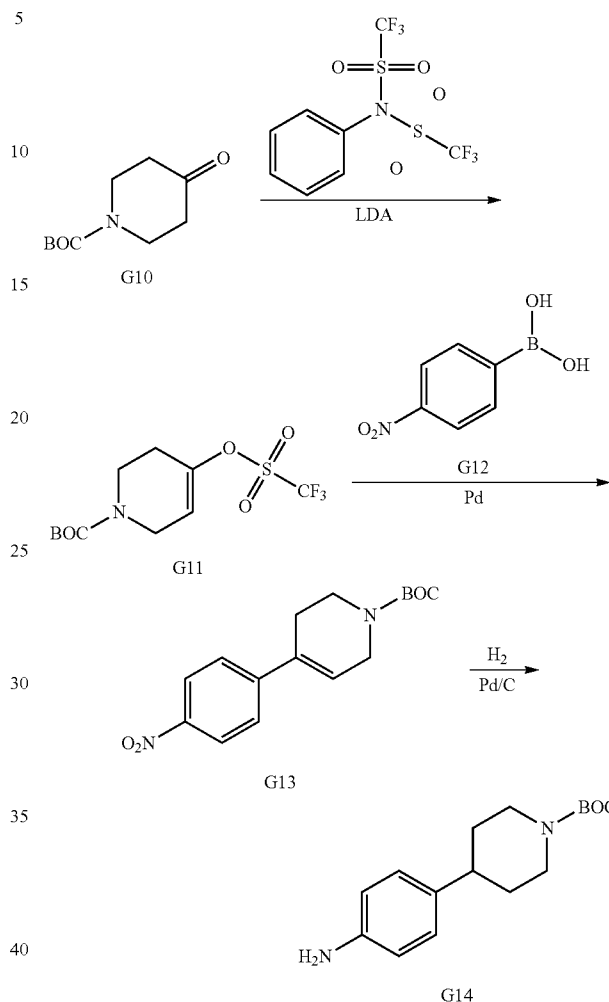
Scheme E
