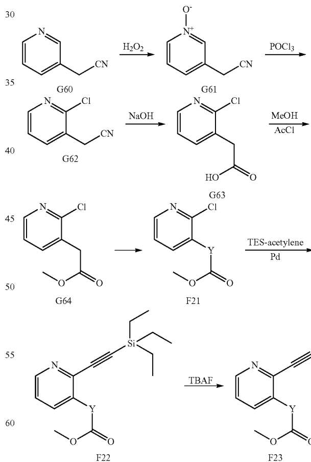
Scheme R
