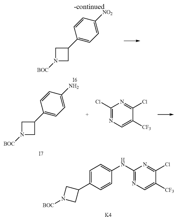
(a) tert-Butyl-3-(4-nitrophenyl)azetidine-1-carboxylate (I6)
