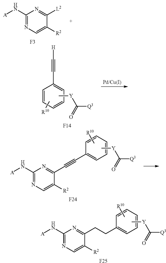
Scheme S
