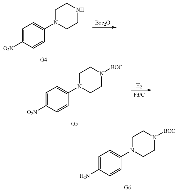
Scheme C
