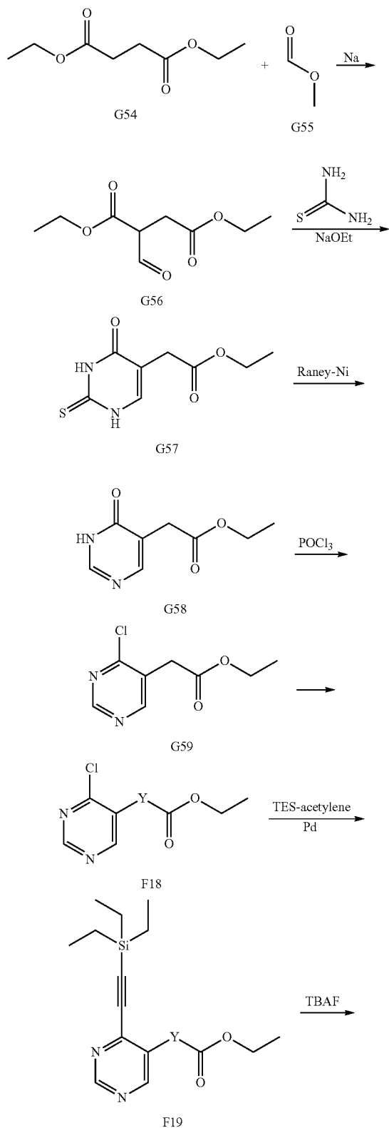
Scheme Q
