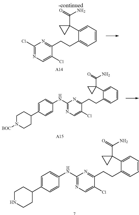
(a) tert-Butyl 4-((4-(2-(1-carbamoylcyclopropyl)phenethyl)-5-chloropyrimidin-2-yl)amino)phenyl piperidine-1-carboxylate (A15)
