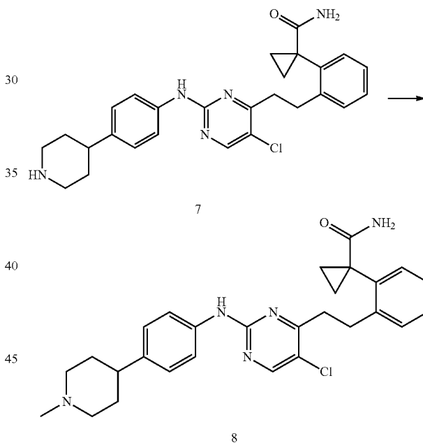
(a) tert-Butyl 4-((4-(2-(1-carbamoylcyclopropyl)phenethyl)-5-chloropyrimidin-2-yl)amino)phenyl piperidine-1-carboxylate (A15)
