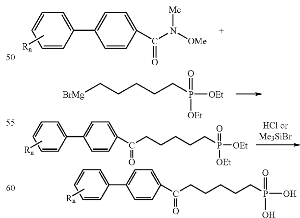
Scheme 20
