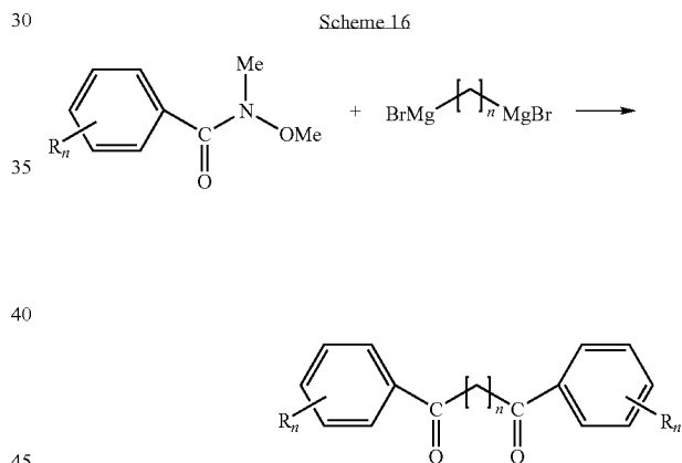
Scheme 16
