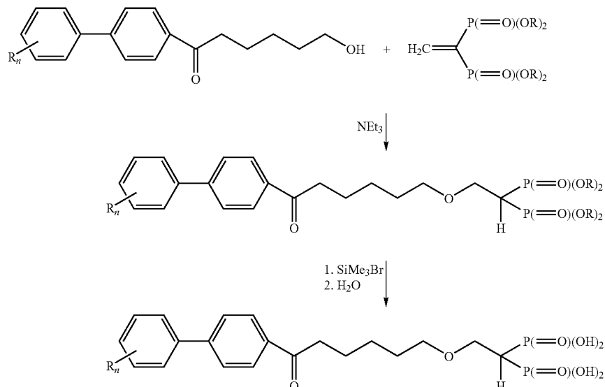
Scheme 17
