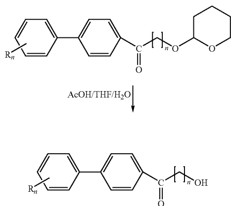
Scheme 11
