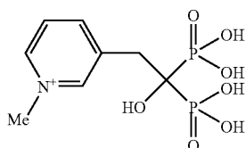
methyl pyridinium analogue
