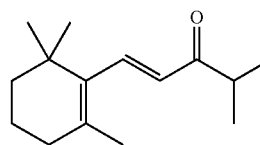
2,4-dimethyl-1-(2,6,6-trimethylcyclohex-1-en-1-yl)pent-1-en-3-one
