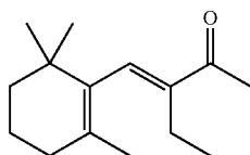
1-(2,6,6-trimethylcyclohex-2-en-1-yl)hex-1-en-3-one
