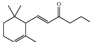
-continued 1-(2,2-dimethyl-6-methylcyclohexyl)-2-methylhex-1-en-3-one
