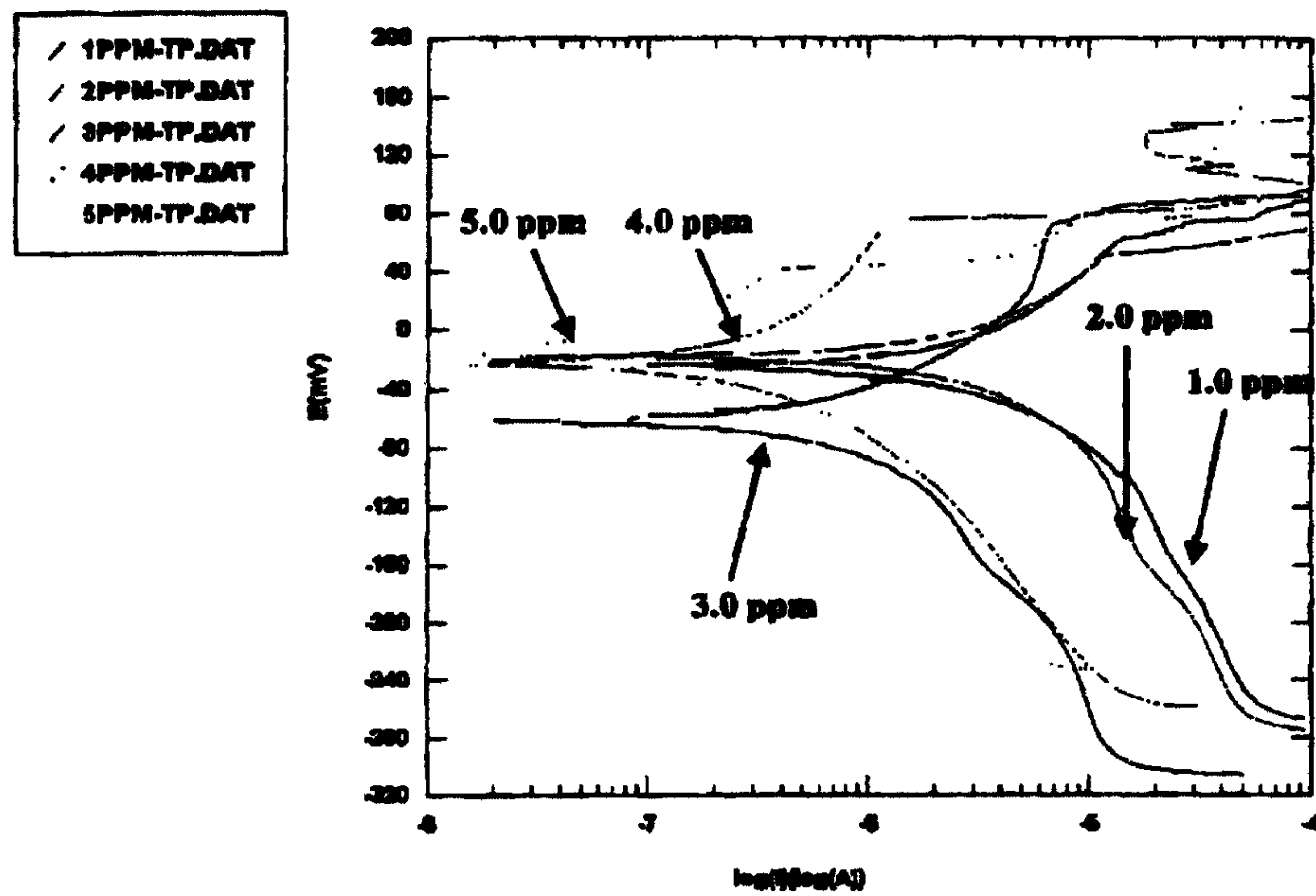
Figure 4. Tafel Comparison of Active Di-benzyl CCI Dosages on admiralty brass electrodes
