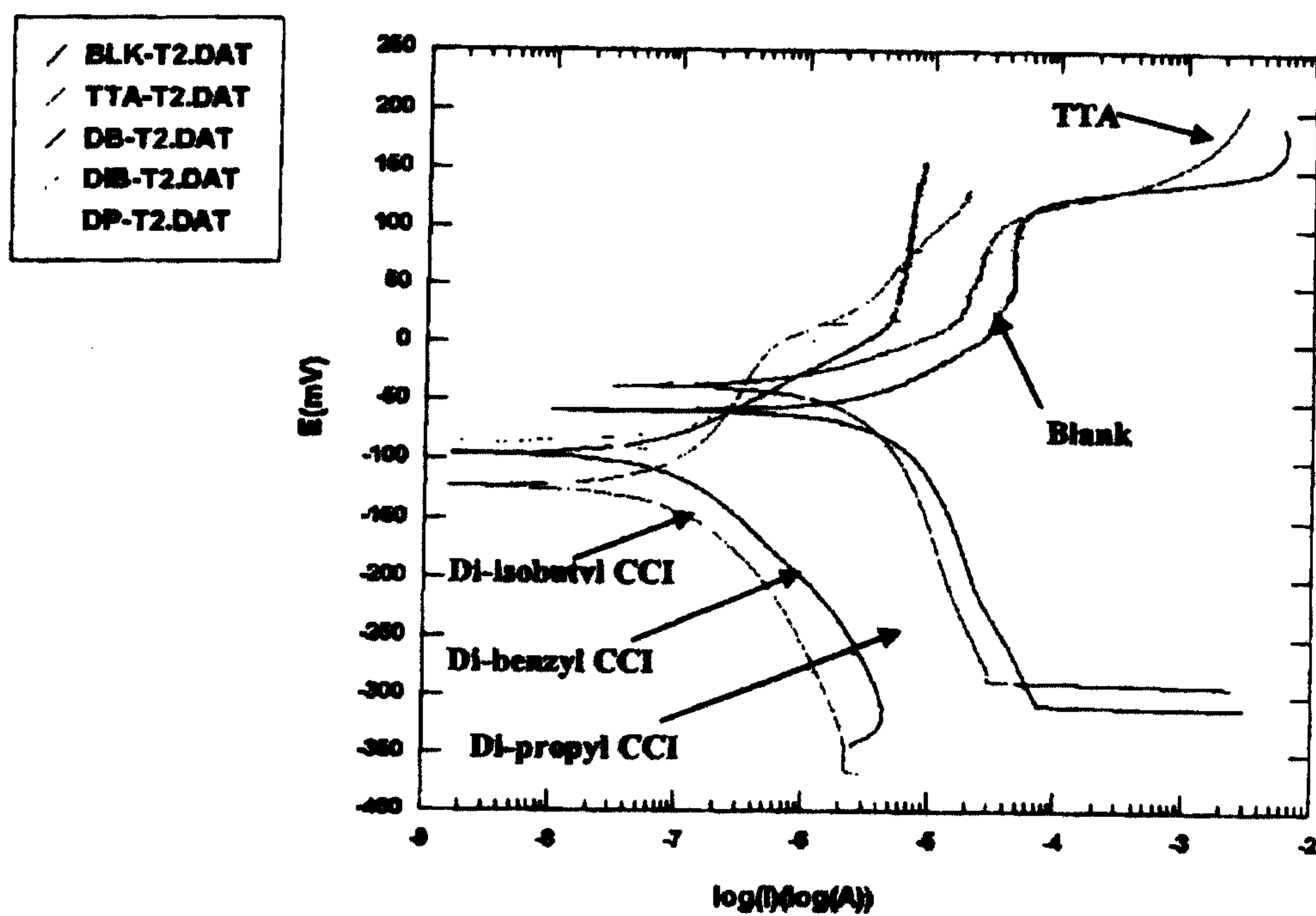
Figure 6. Tafel Plots of Inhibitors without Residual Inhibitor
