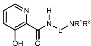
Formula (V)
