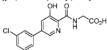
Compound 1
