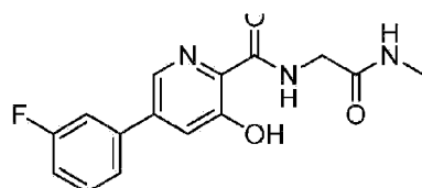
Compound 11
