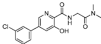
Compound 6
