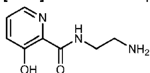
Compound 13
