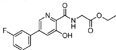
Compound 9
