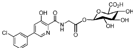
Metabolite 2
