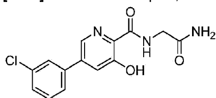
Compound 4
