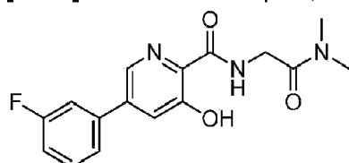
Compound 12
