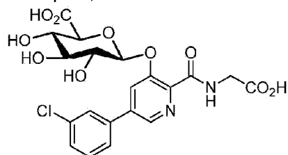
Metabolite 1
