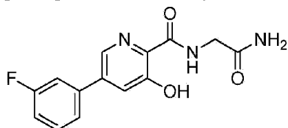
Compound 10
