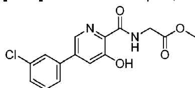
Compound 2
