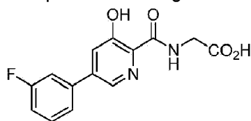
Compound 7
