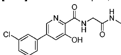
Compound 5
