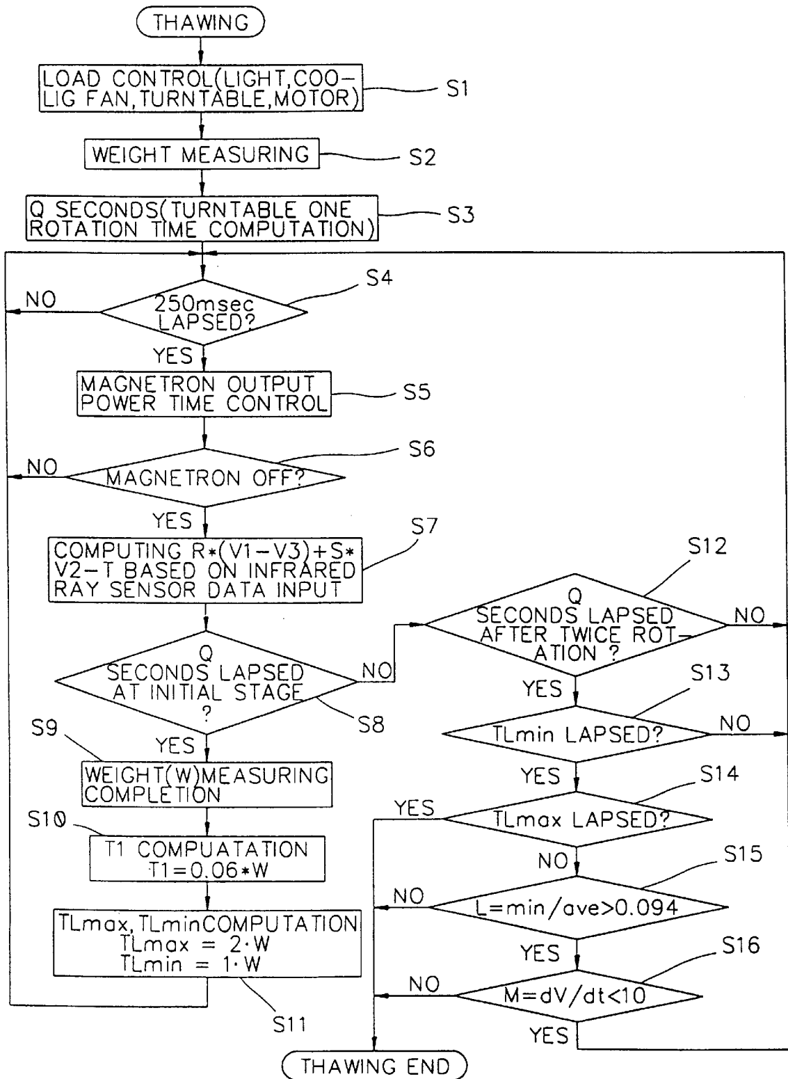
FIG. 3 CONVENTIONAL ART
