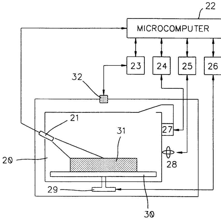
FIG. 1 CONVENTIONAL ART
