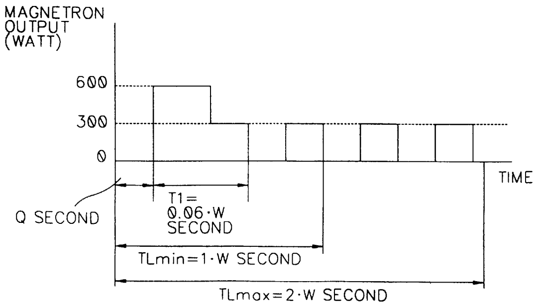
FIG. 2 CONVENTIONAL ART
