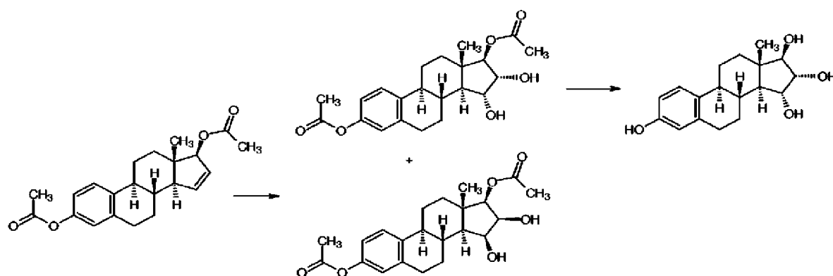
Reaction Scheme 2
