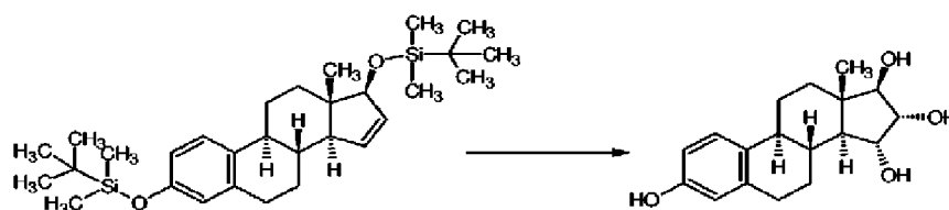
Reaction Scheme 4
