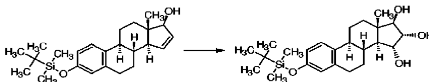
Reaction Scheme 9
