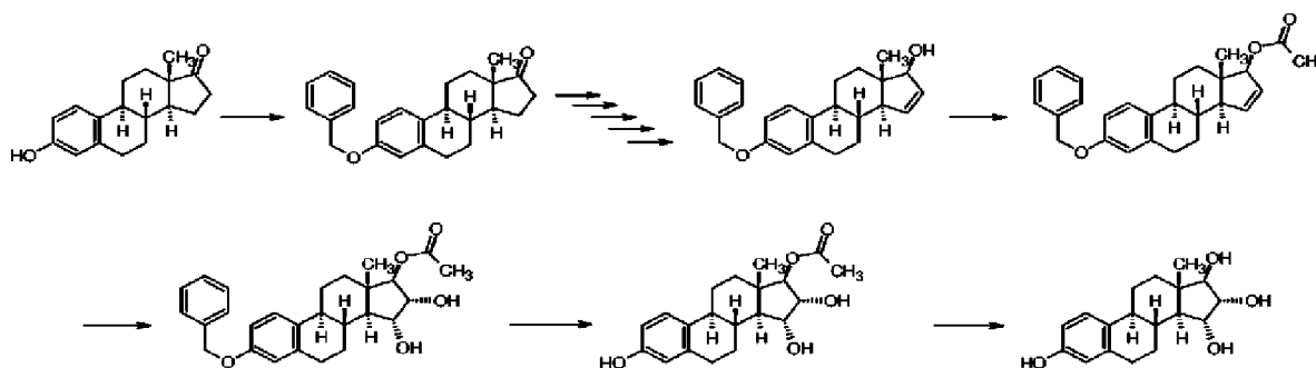
Reaction Scheme 3
