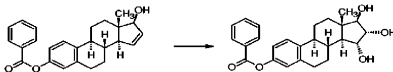
Reaction Scheme 8
