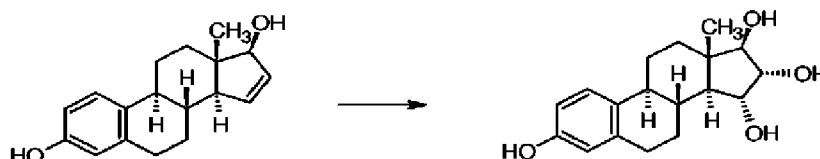
Reaction Scheme 6
