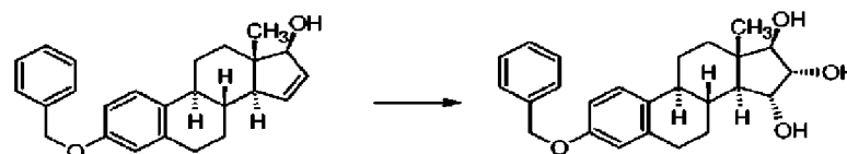
Reaction Scheme 7
