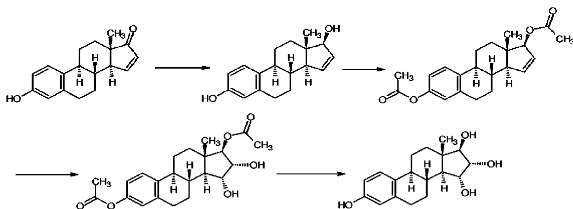
Reaction Scheme 1
