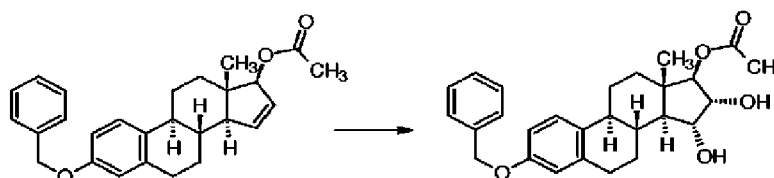
Reaction Scheme 5
