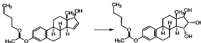
Reaction Scheme 10
