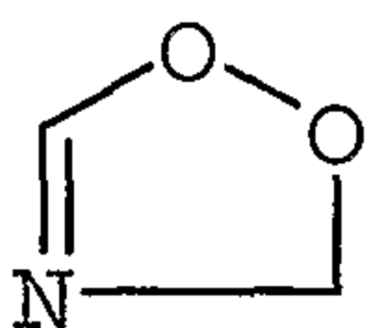
1,2,4-dioxazolyl
