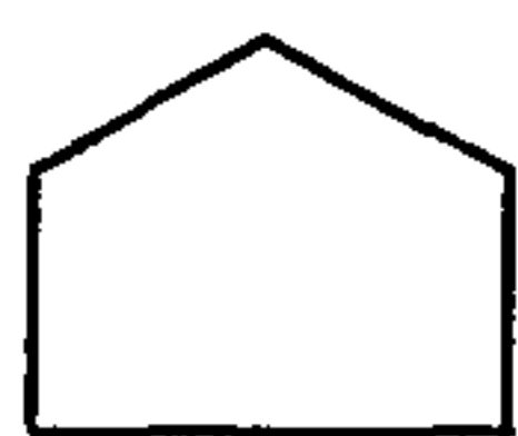
cyclopentyl
