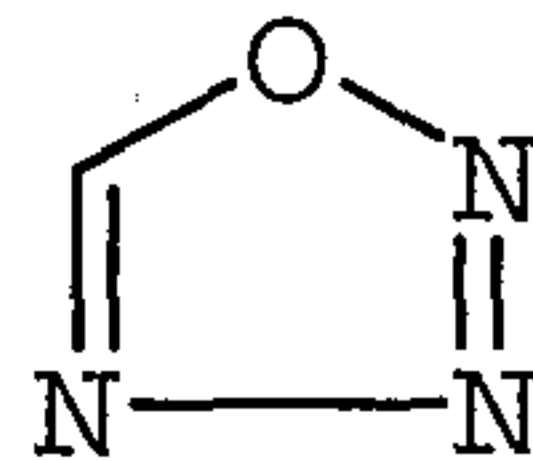
1,2,3,4-oxatriazolyl
