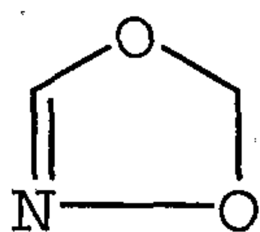
1,3,4-dioxazolyl
