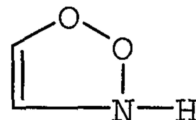
3H-1,2,3-dioxazolyl
