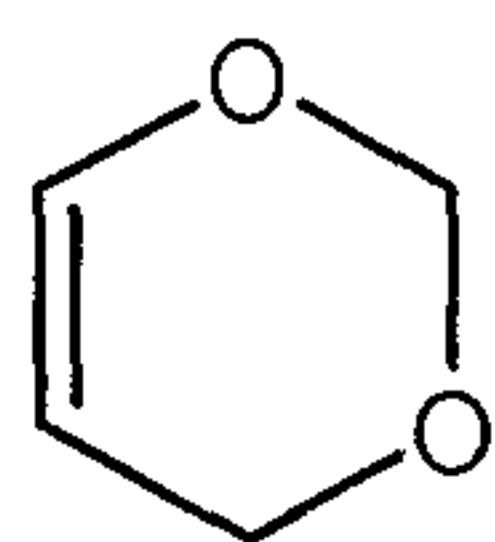
20 1,3-dioxinyl
