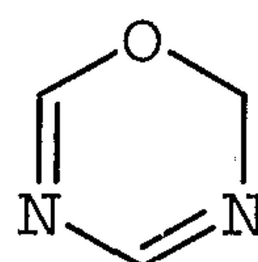
1,3,5,2-oxadiazinyl
