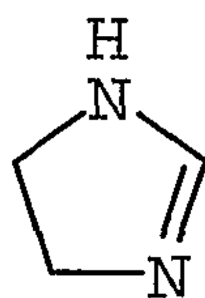
2-imidazolinylyl
