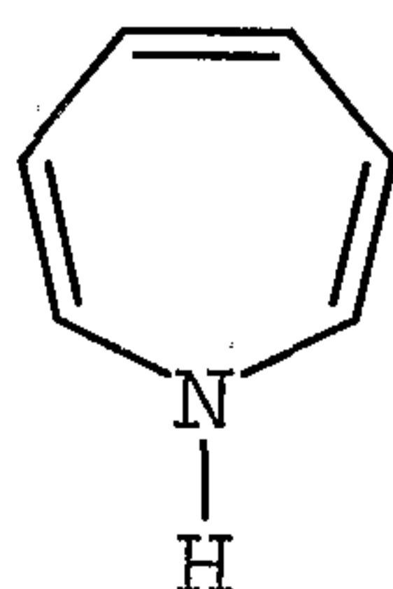
azepinyl
