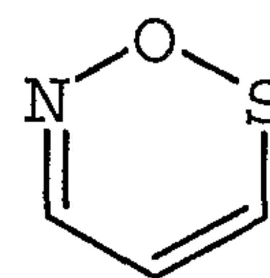
1,2,6-oxathiazinyl
