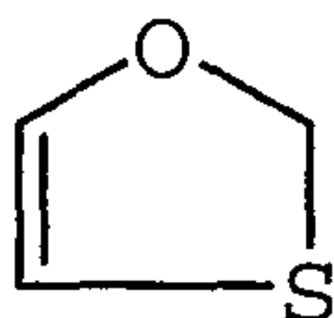
1,3-oxathiolyl
