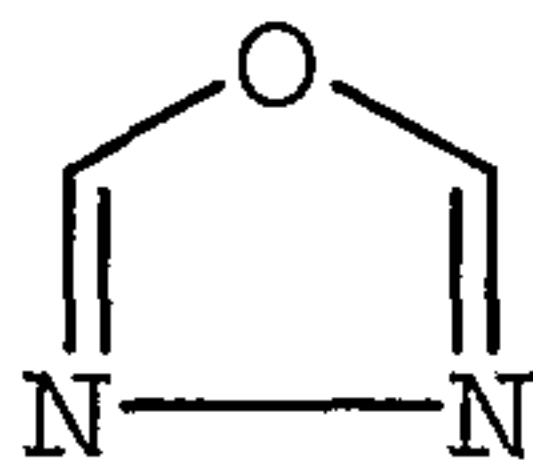
1,3,4-oxadiazolyl
