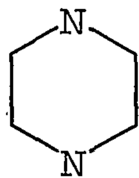
5 piperazinyl
