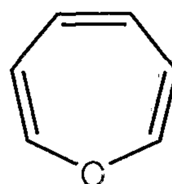
oxepinyl
