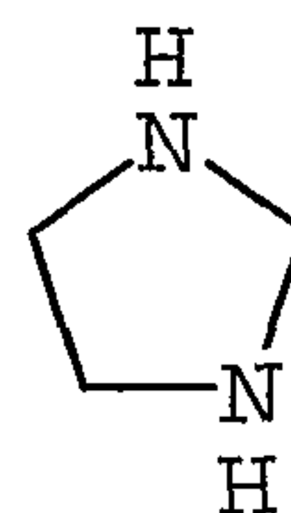
imidazolidinylyl
