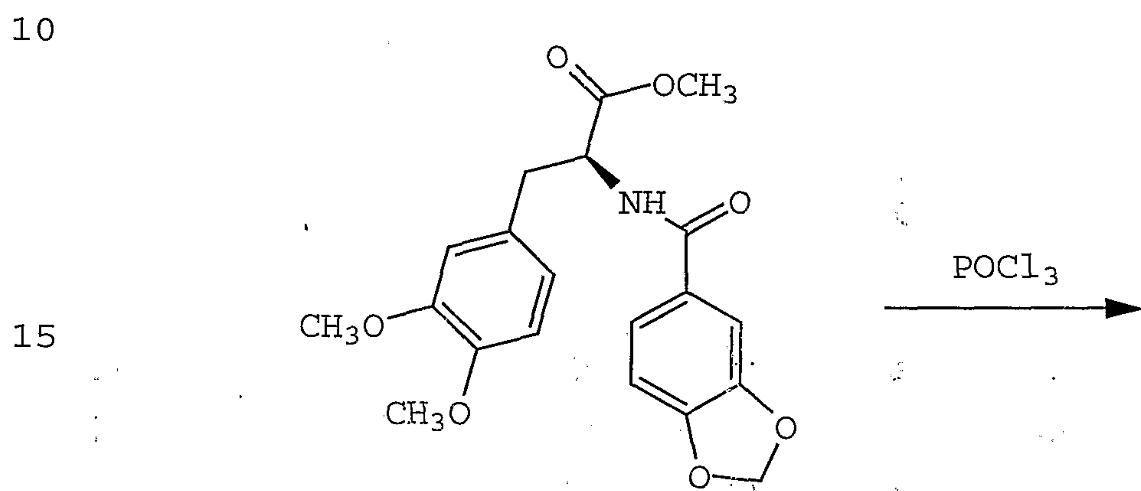
Intermediate 5.
