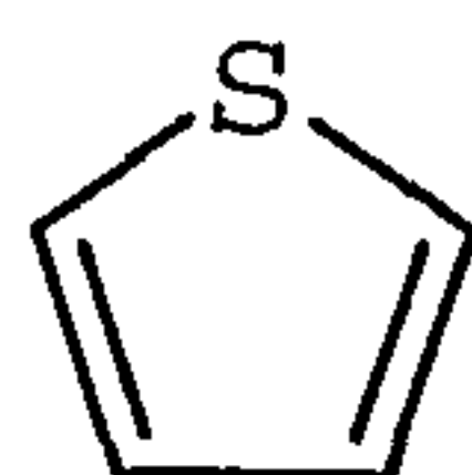
thienyl
