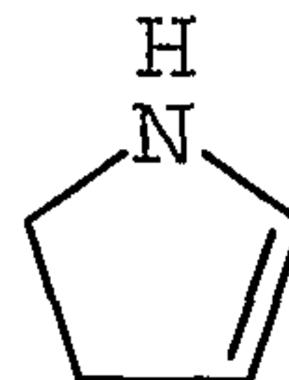
2-pyrrolynyl
