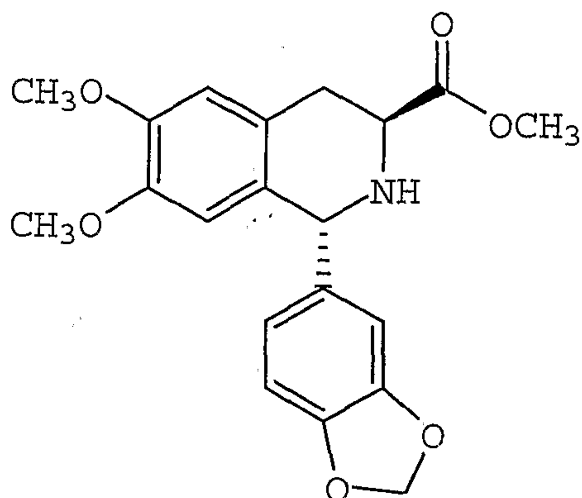
Intermediate 7
