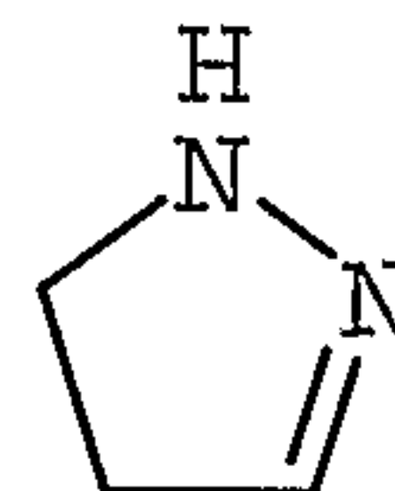
2-pyrazolinyl
