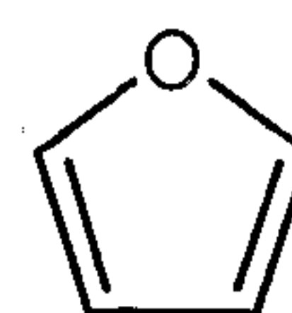
furanyl
