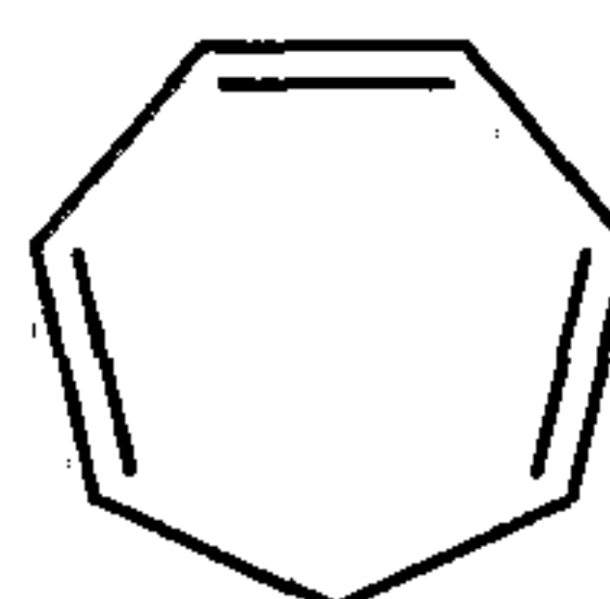
1,3,5-cycloheptatrienyl
