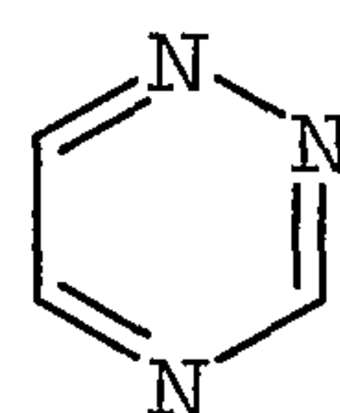
1,2,4-triazinyl
