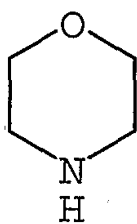
morpholinyl
