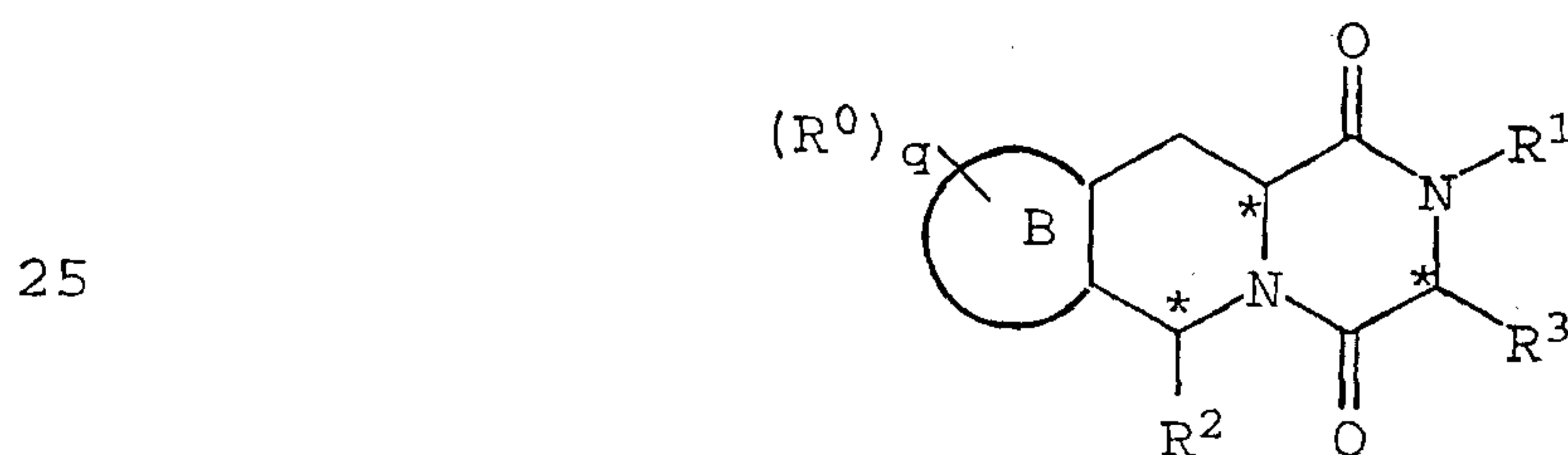
(I)
