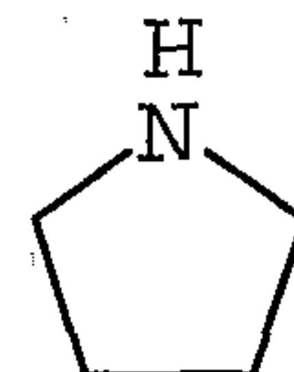
pyrrolidinyl
