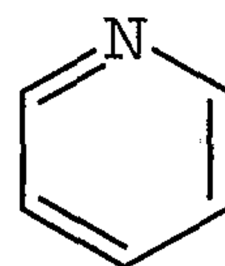
pyridinyl
