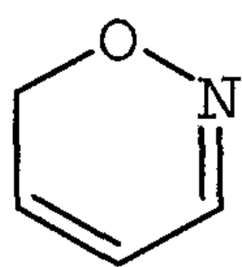
6H-1,2-oxazinyl
