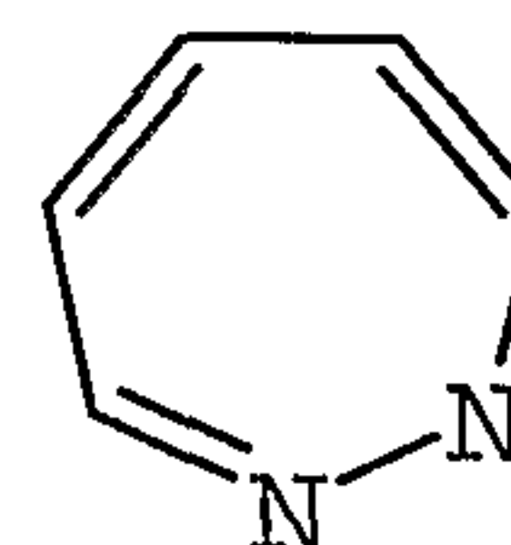
1,2,4-diazepinyl
