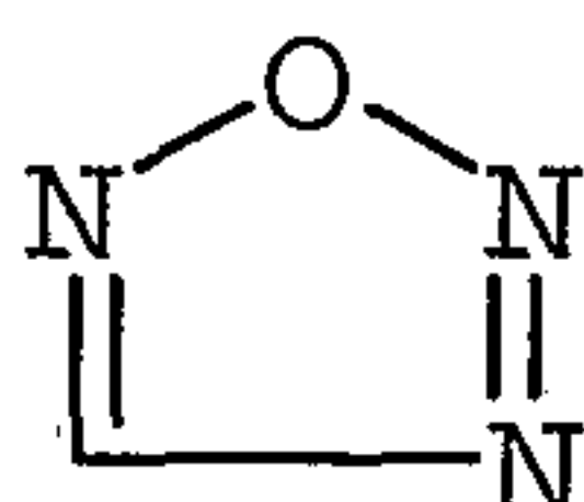
1,2,3,5-oxatriazolyl
