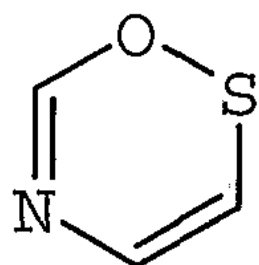
1,2,5-oxathiazinyl
