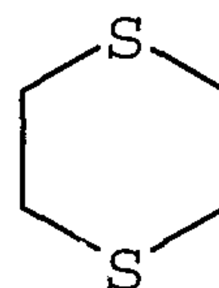
1,4-dithianyl
