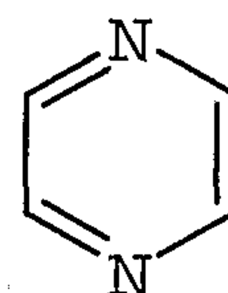
pyrazinyl
