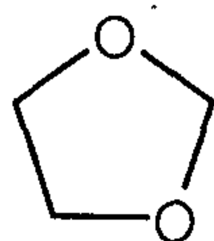
1,3-dioxolanyl
