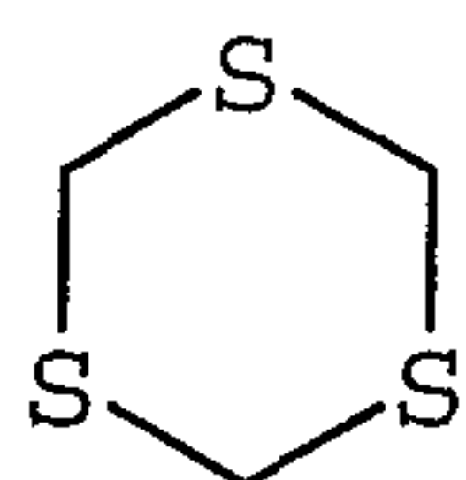
10 1,3,5-trithianyl
