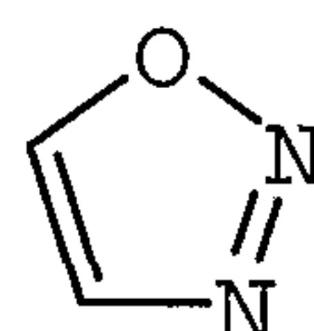
1,2,3-oxadiazolyl
