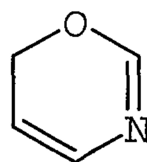
6H-1,3-oxazinyl
