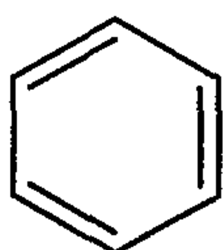
phenyl
