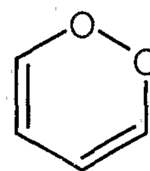
1,2-dioxinyl
