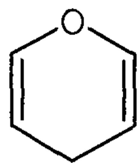
4H-pyranyl
