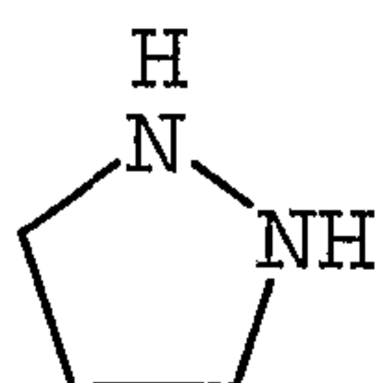
pyrazolidinyl
