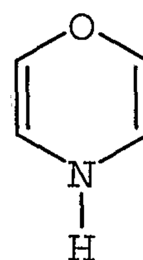
4H-1,4-oxazinyl
