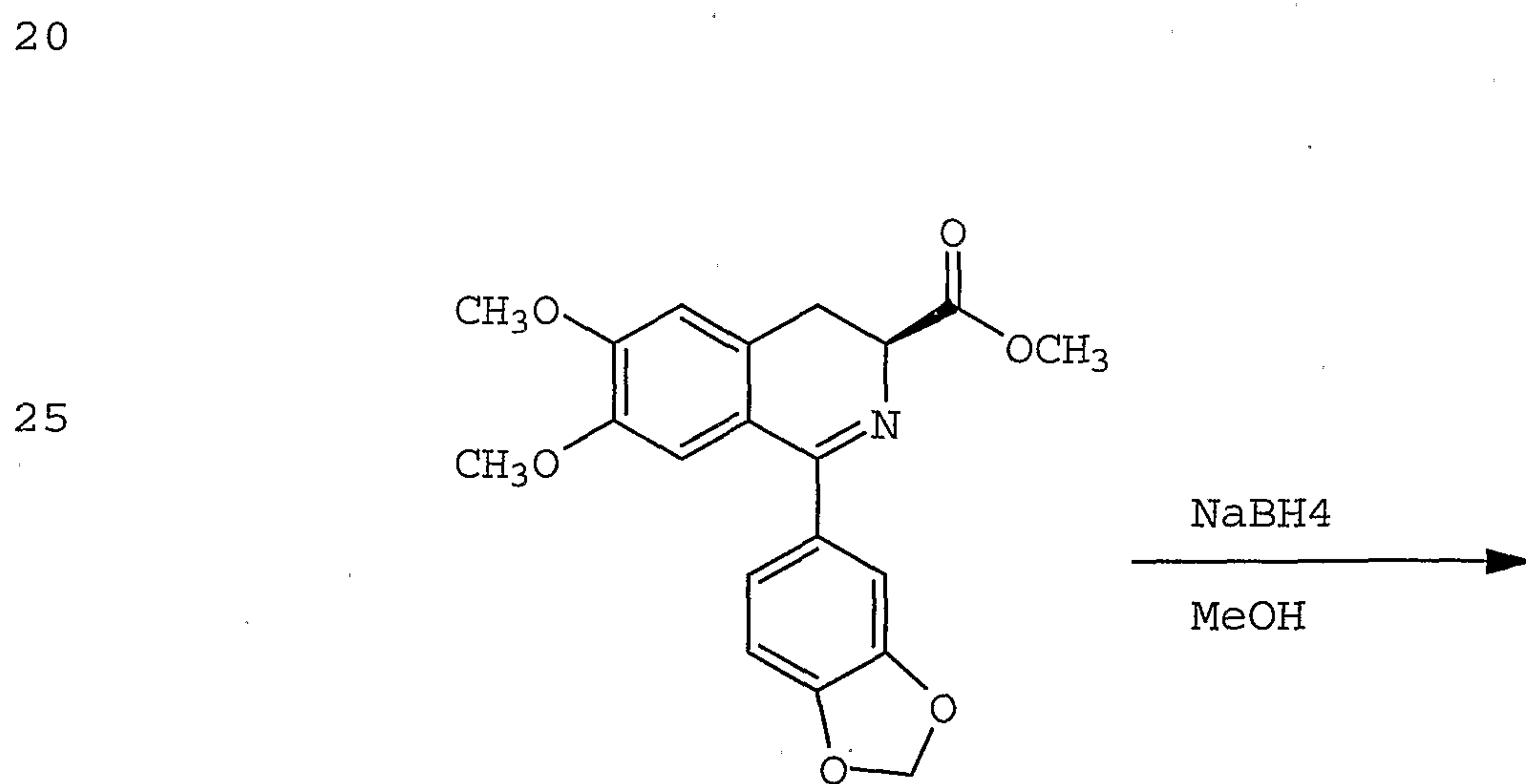
Intermediate 6
