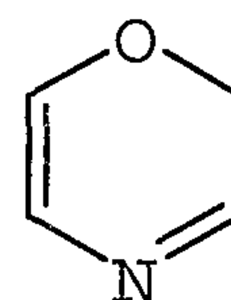
1,4-oxazinyl
