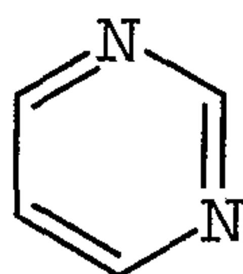
pyrimidinyl
