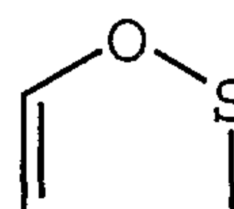
3H-1,2-oxathiolyl
