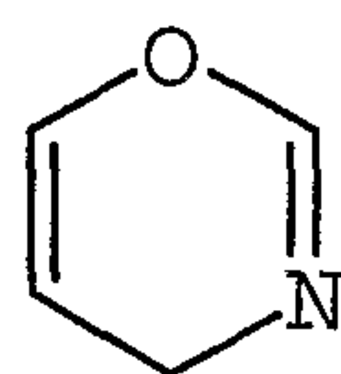
4H-1,3-oxazinyl
