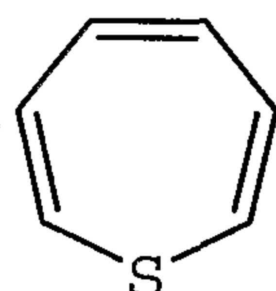
thiopinyl
