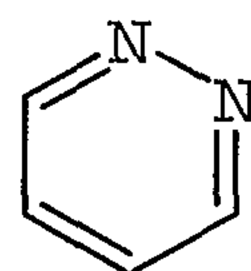
pyridazinyl
