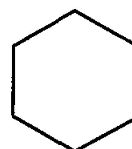
cyclohexyl
