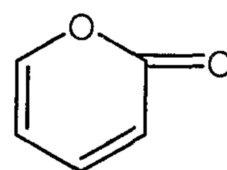
2-pyronyl
