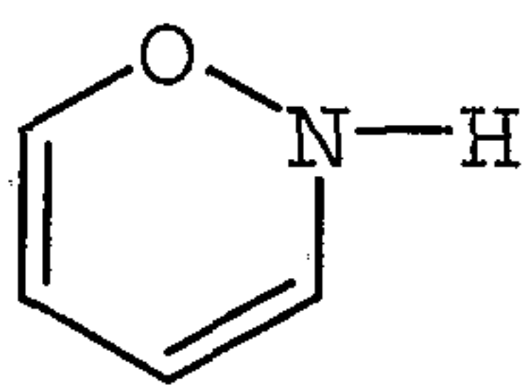
2H-1,2-oxazinyl
