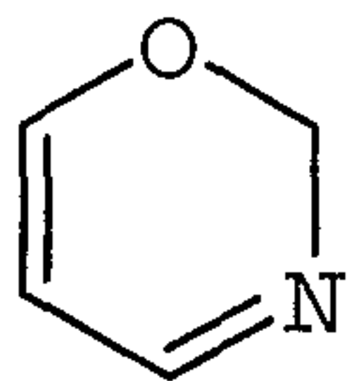
2H-1,3-oxazinyl
