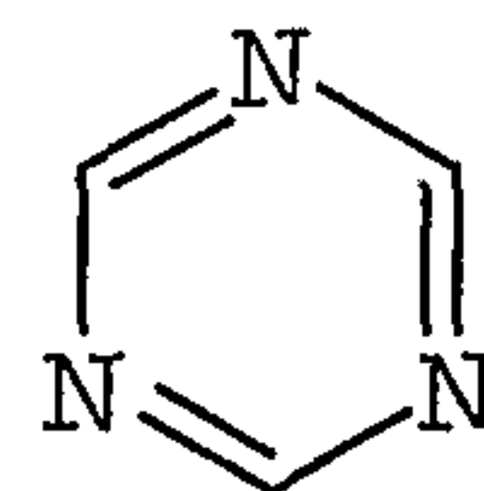
1,3,5-triazinyl
