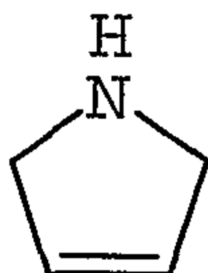
3-pyrrolynyl
