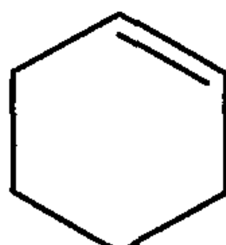
cyclohexenyl
