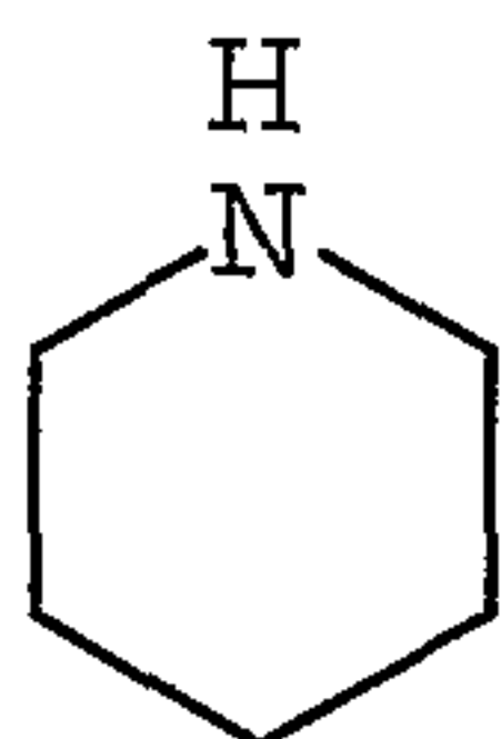
piperidinyl
