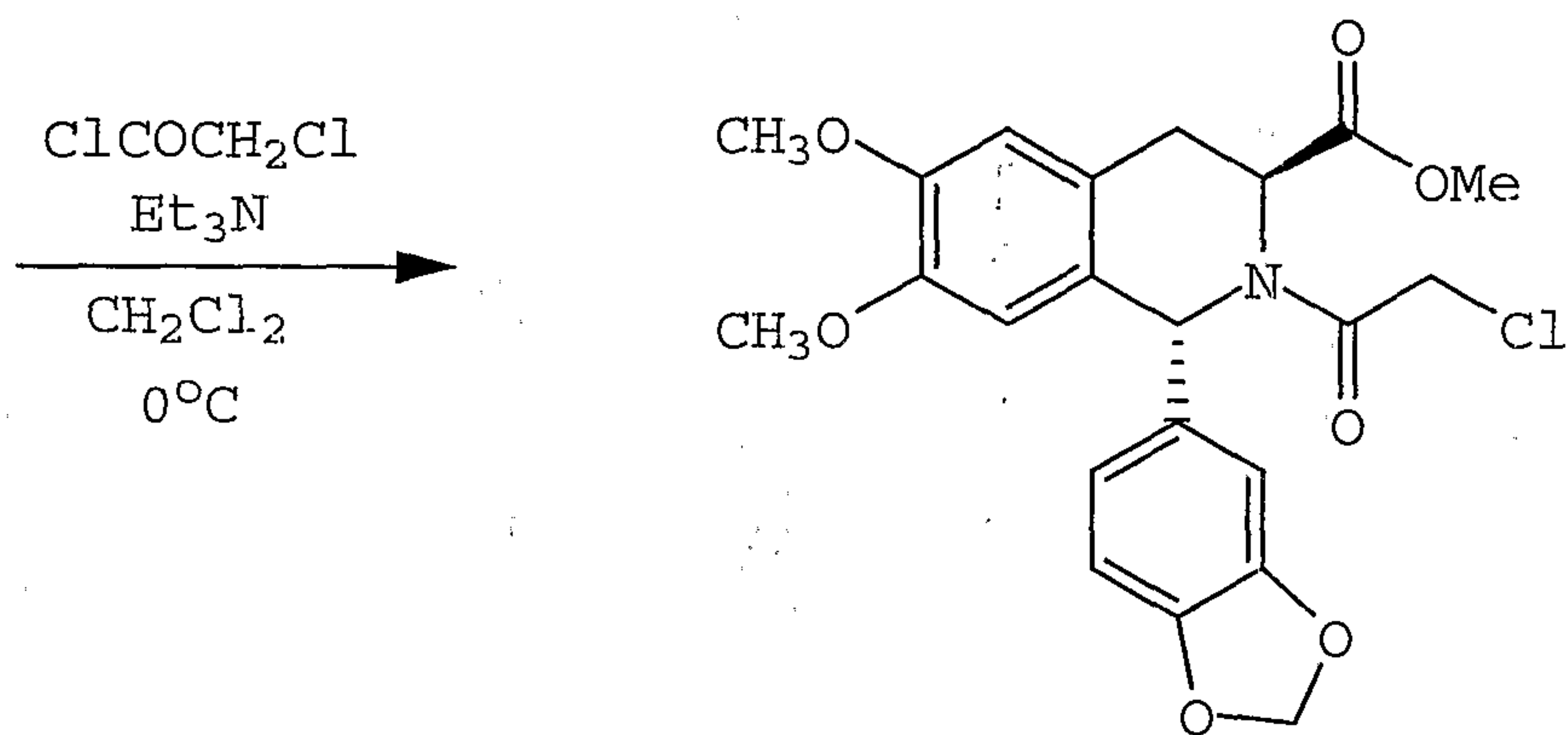
Intermediate 8
