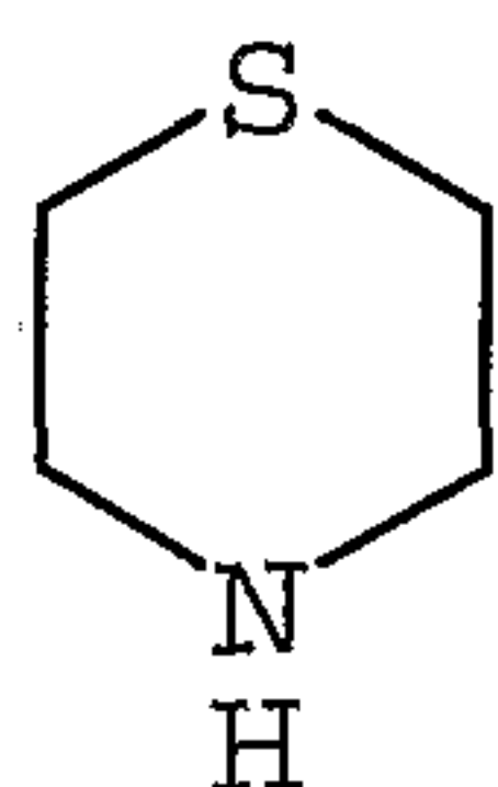
thiomorpholinyl
