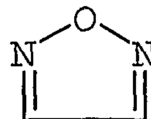
1,2,5-oxadiazolyl
