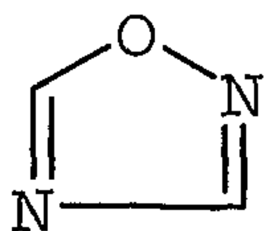
1,2,4-oxadiazolyl
