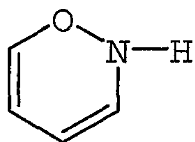
o-isoxazinyl
