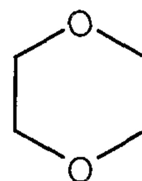
1,4-dioxanyl
