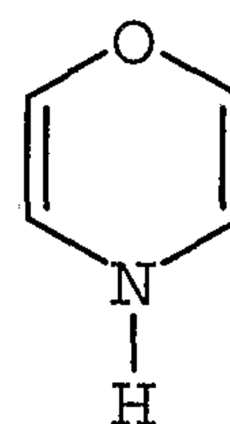
p-isoxazinyl
