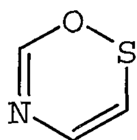
1,2,5-oxathiazinyl
