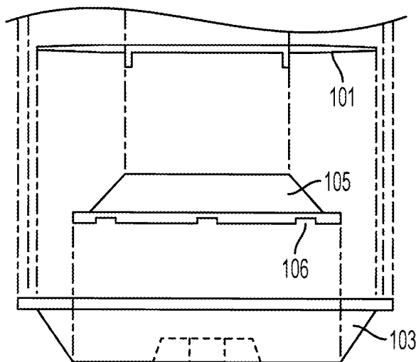
FIG. 1B (SIDE VIEW)
