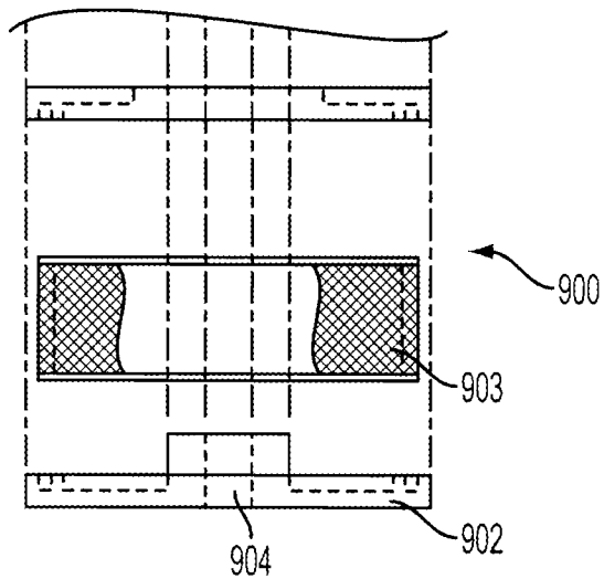
FIG. 9B (SIDE VIEW)
