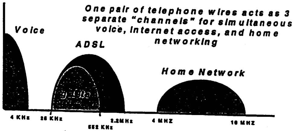
Spectral Allocation of Existing services sharing the Phoneline Media
