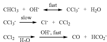
[Reaction Scheme 3]
