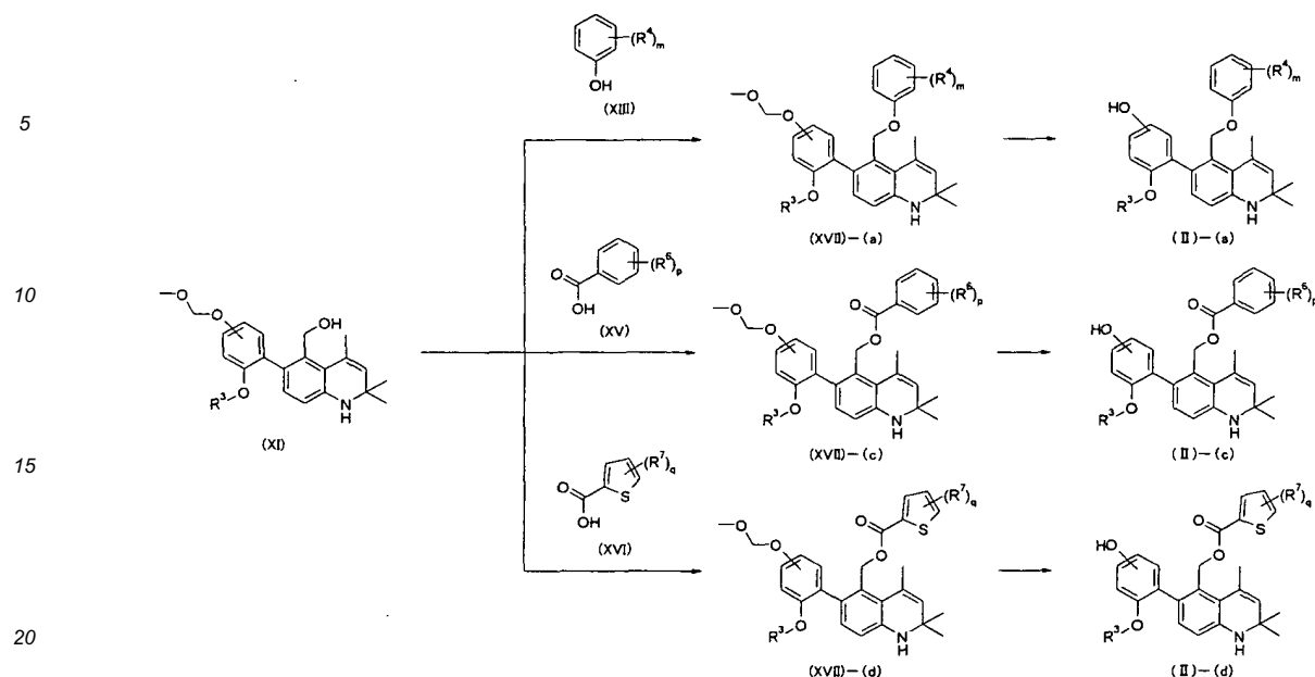
Synthetic Route 7
