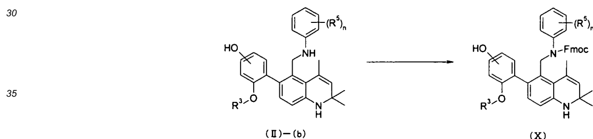
Synthetic Route 8
