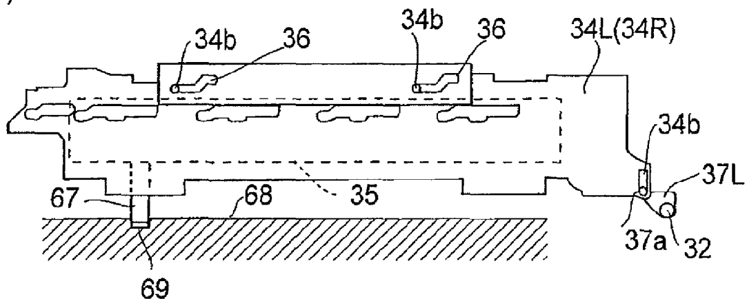
(a) CLOSED STATE
