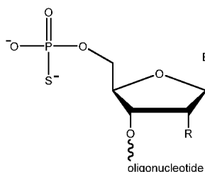
5' phosphorothioate monophosphate
