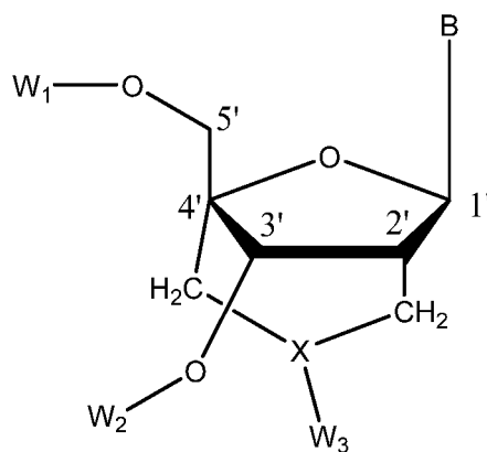
Formula I
