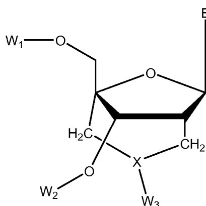
Formula I
