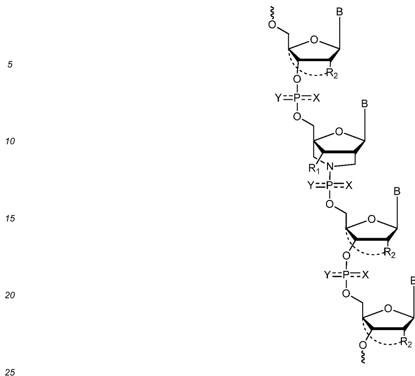
Formula II
