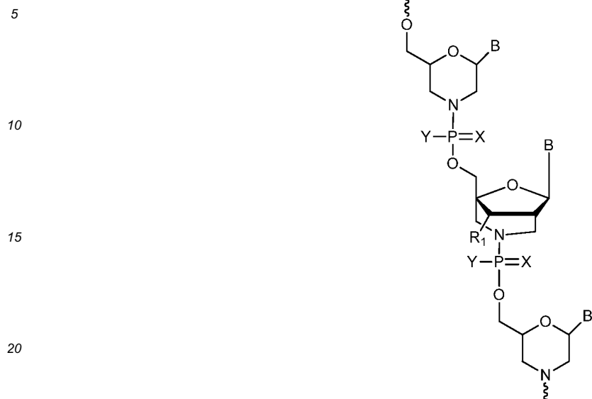
25 Formula IV
