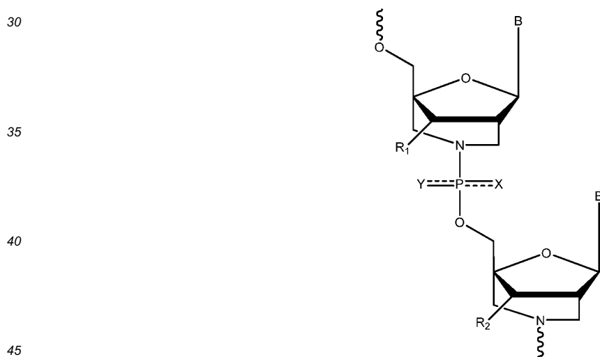
Formula III
