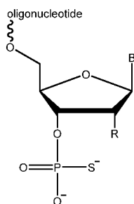
3' phosphorothioate monophosphate
