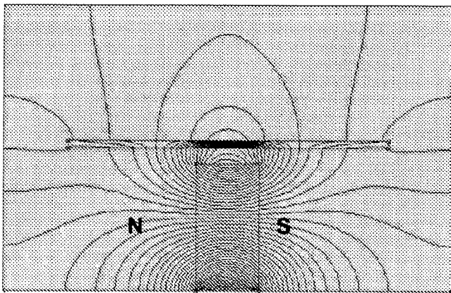
0.060" thick sheet metal from the steel 1018
