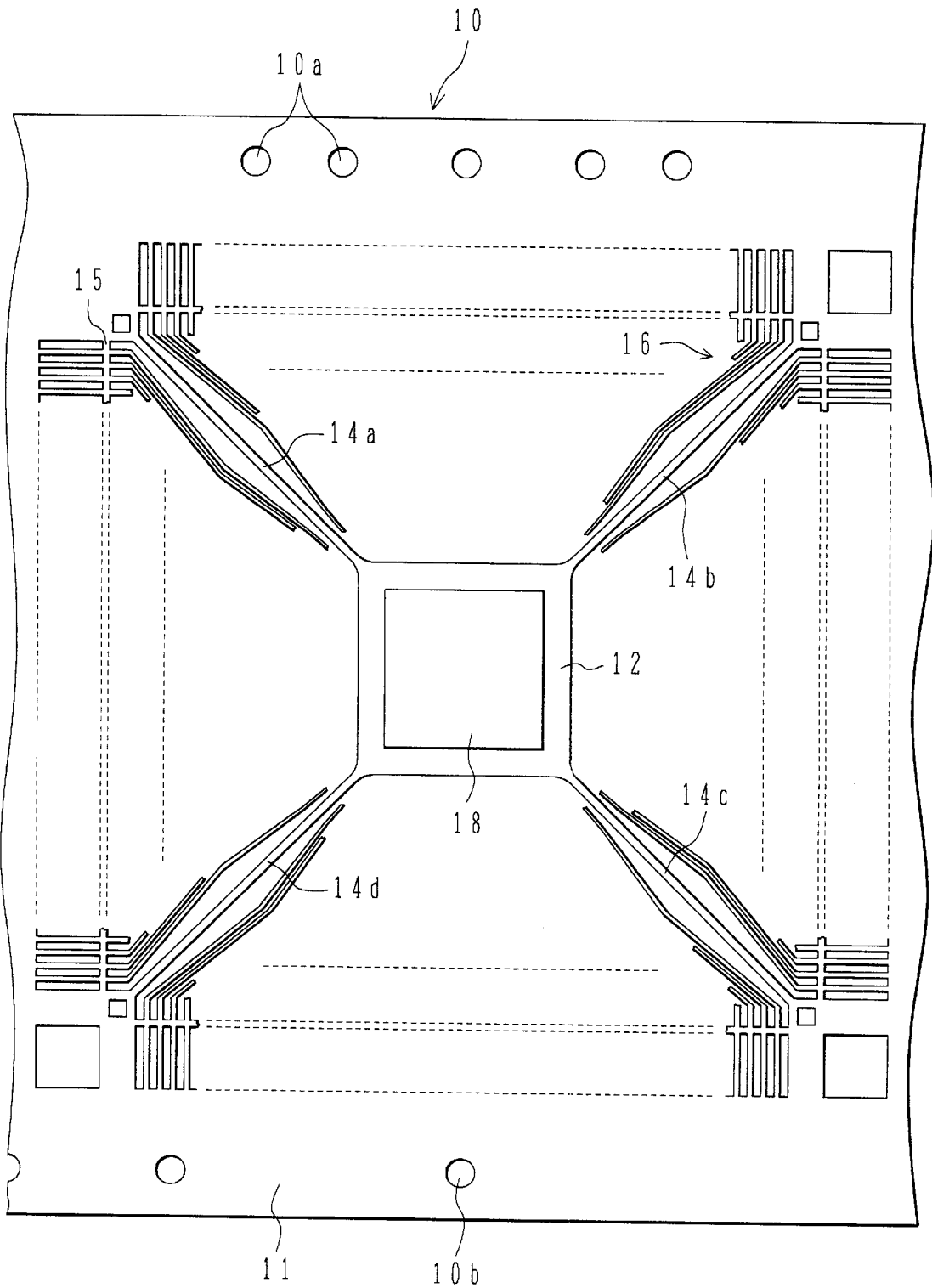
FIG. 9 PRIOR ART
