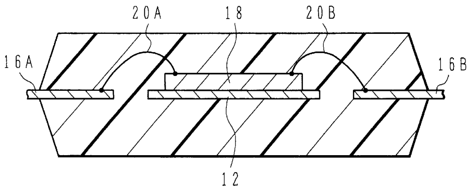
FIG.12 PRIOR ART
