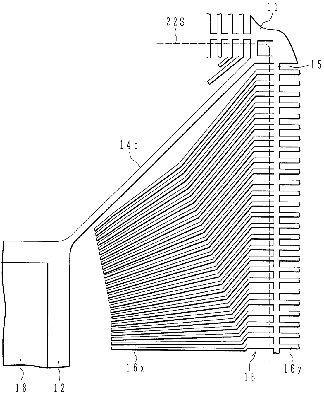
FIG.10 PRIOR ART
