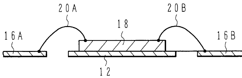
FIG.11 PRIOR ART
