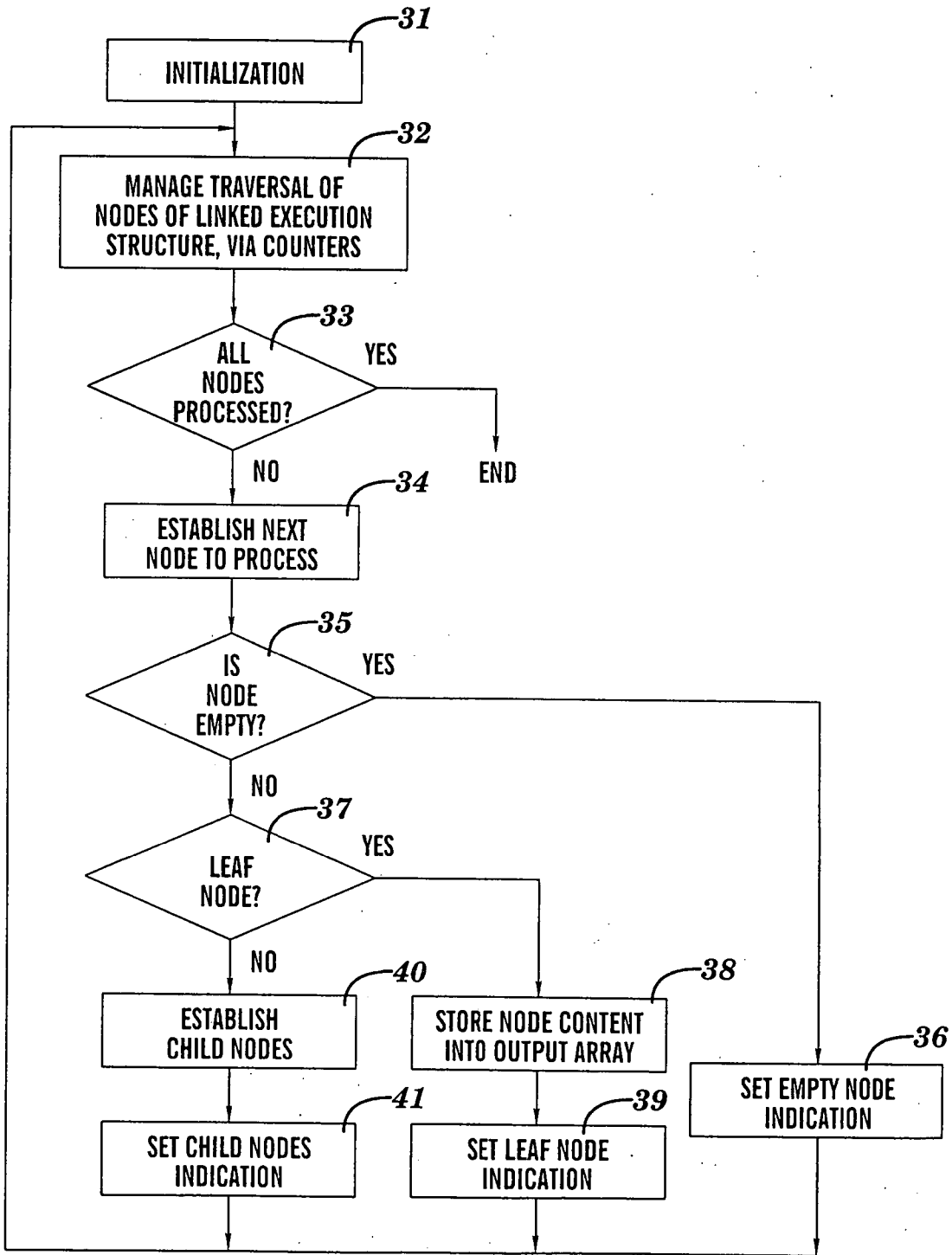
FIG. 6 (COUNTER-CONTROLLED LOOPING)
