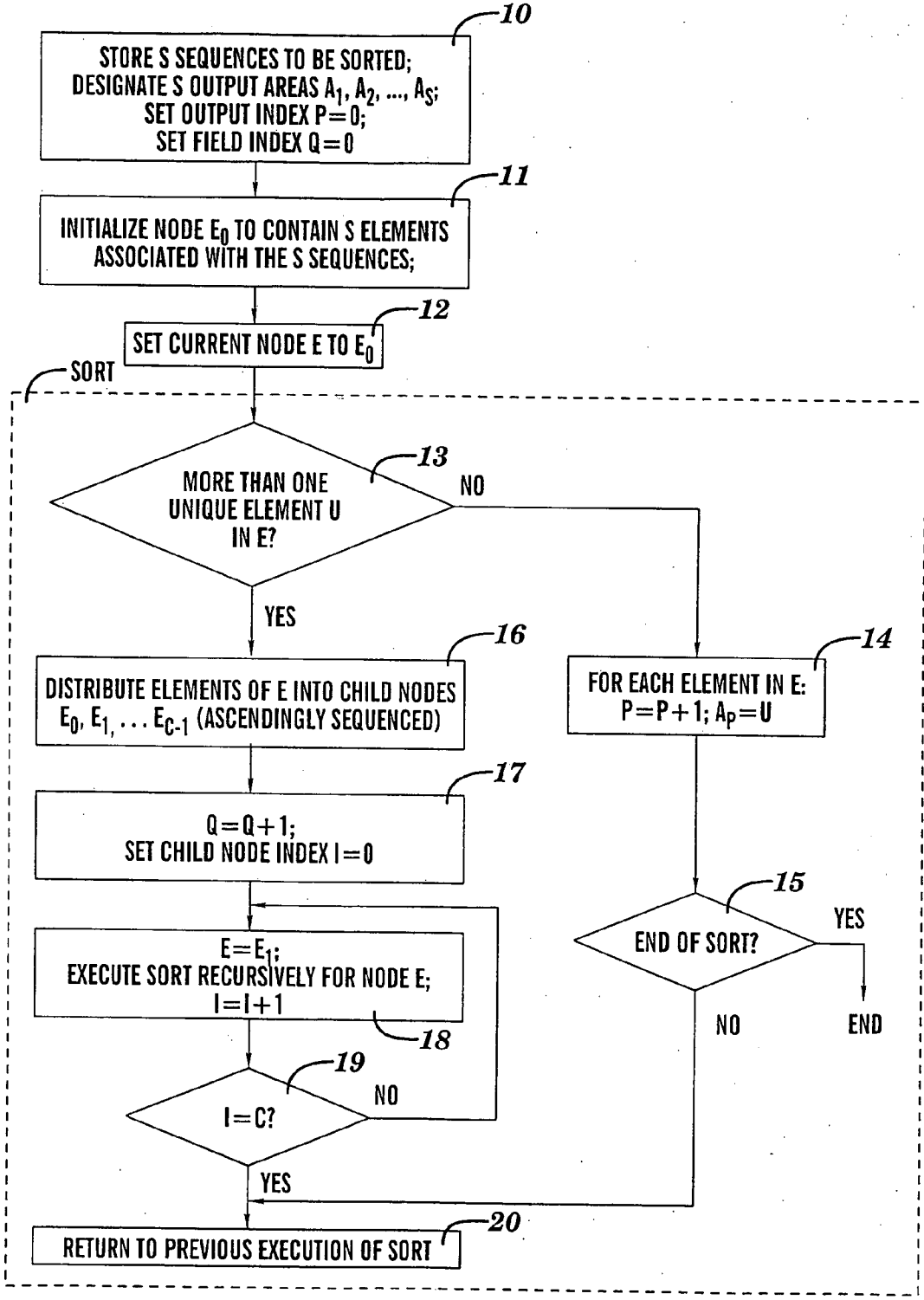
FIG. 5 (RECURSIVE EXECUTION)
